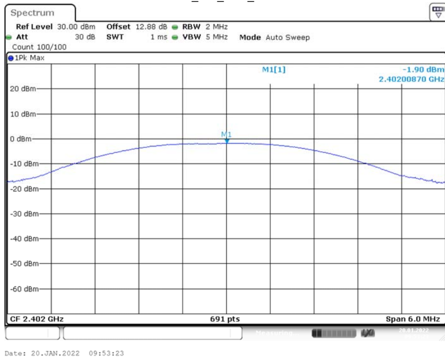
BLE_1M_Ant1_2402
