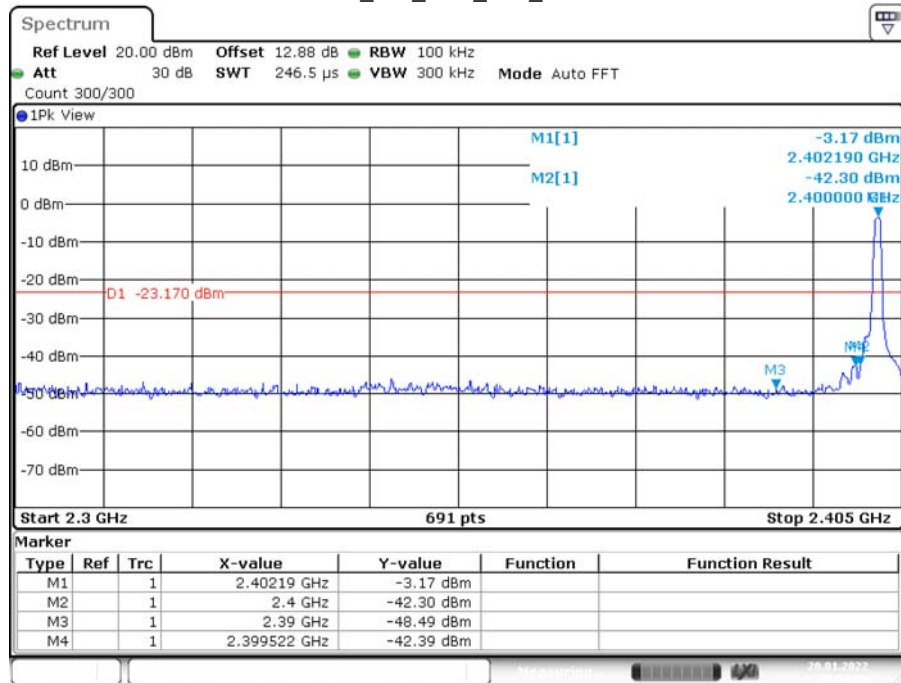
BLE_1M_Ant1_Low_2402
