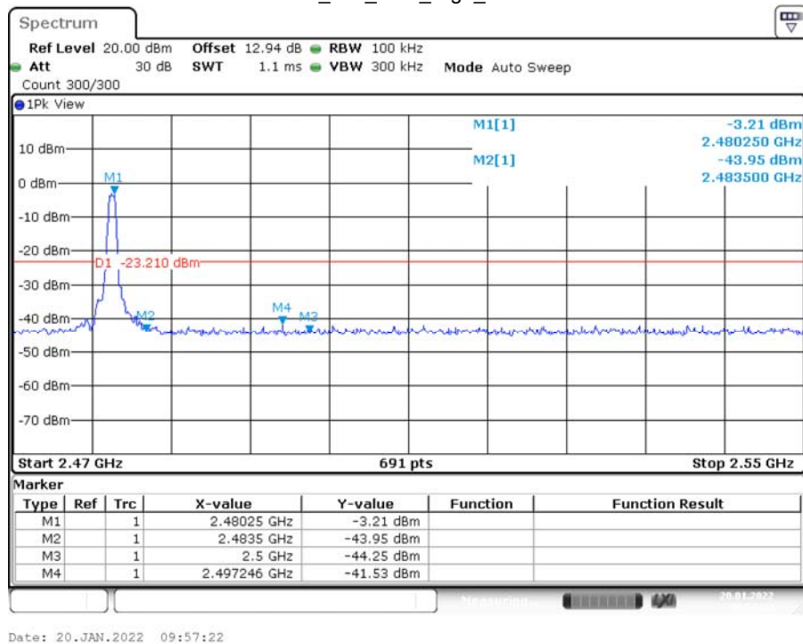
BLE_1M_Ant1_High_2480
