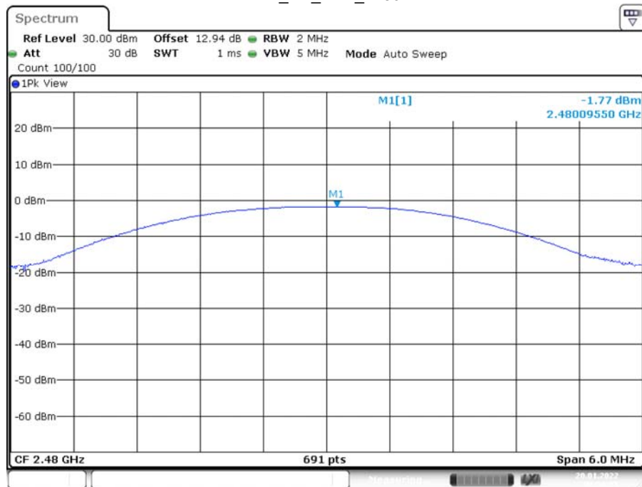
BLE_1M_Ant1_2480
