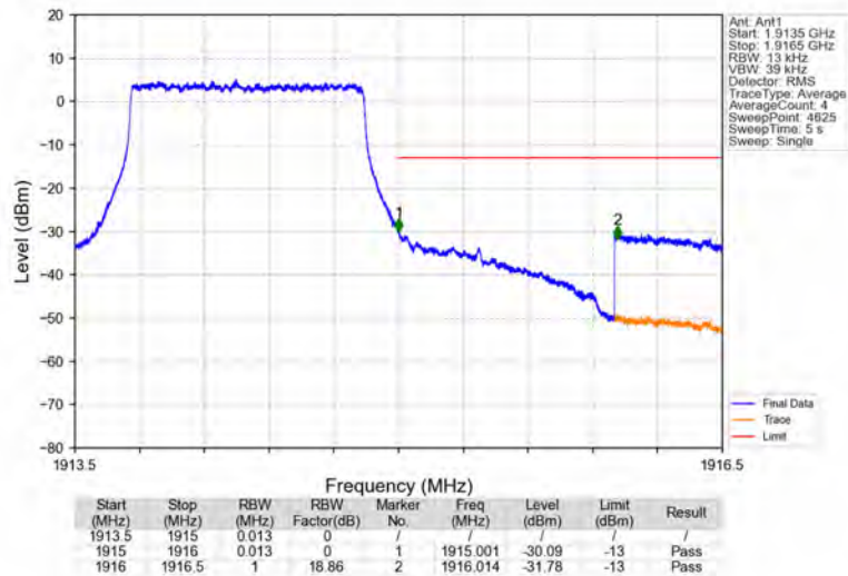
Band25_1.4MHz_QPSK_HCH_1914.3MHz_RB_6_0_NTNV
