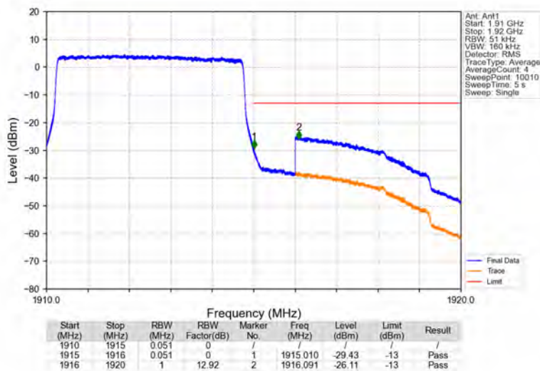
Band25_5MHz_QPSK_HCH_1912.5MHz_RB_25_0_NTNV
