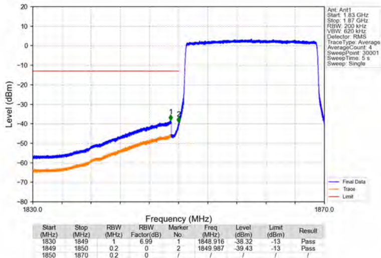
Band25_20MHz_16QAM_LCH_1860MHz_RB_100_0_NTNV
