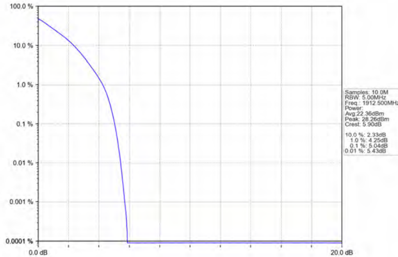
Band25_5MHz_QPSK_HCH_1912.5MHz_RB_25_0_NTNV
