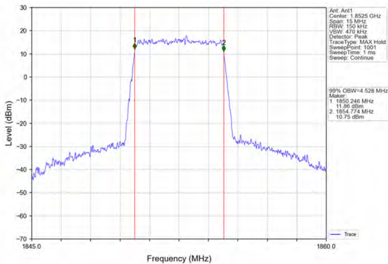
Band25_5MHz_16QAM_LCH_1852.5MHz_RB_25_0_NTNV
