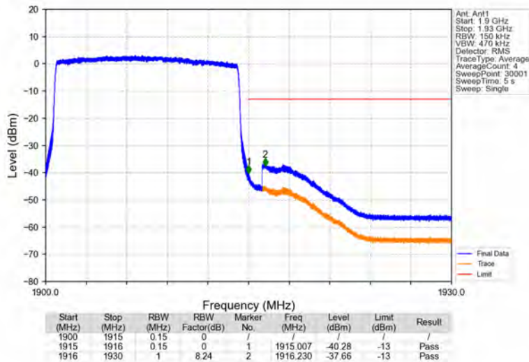
Band25_15MHz_64QAM_HCH_1907.5MHz_RB_75_0_NTNV
