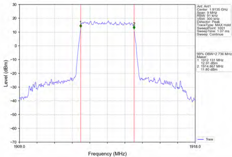
Band25_3MHz_QPSK_HCH_1913.5MHz_RB_15_0_NTNV
