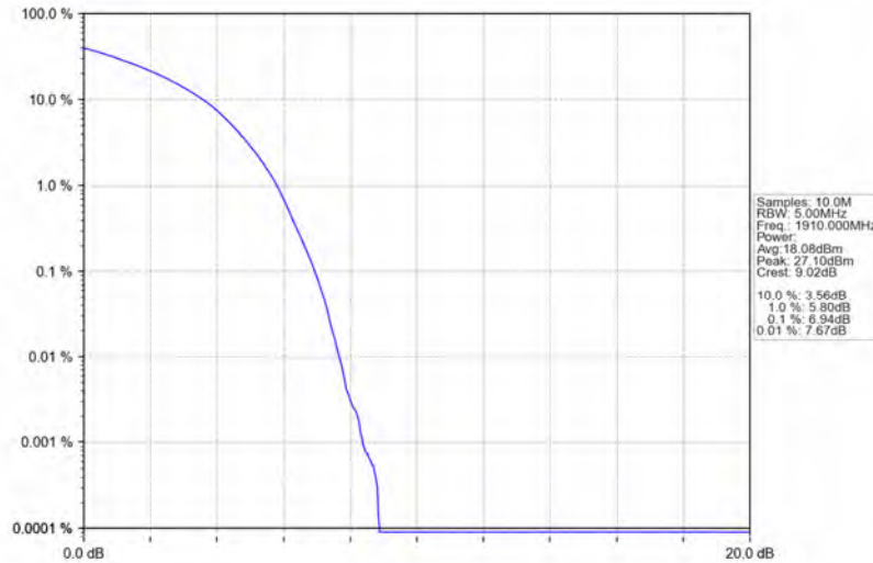
Band25_10MHz_64QAM_HCH_1910MHz_RB_50_0_NTNV
