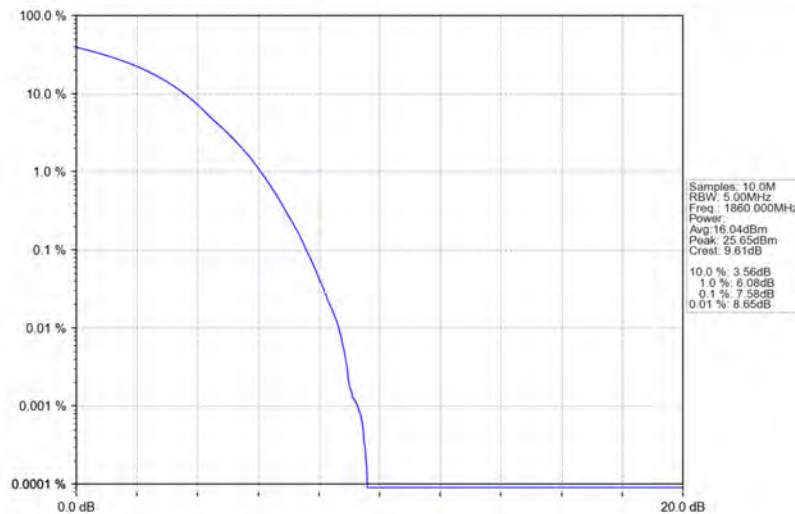
Band25_20MHz_16QAM_LCH_1860MHz_RB_100_0_NTNV
