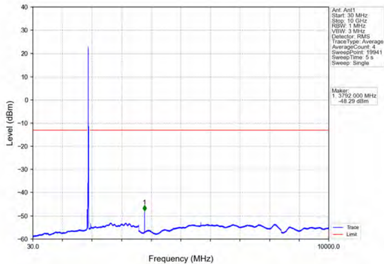
Band25_20MHz_16QAM_HCH_1905MHz_RB_1_0_NTNV
