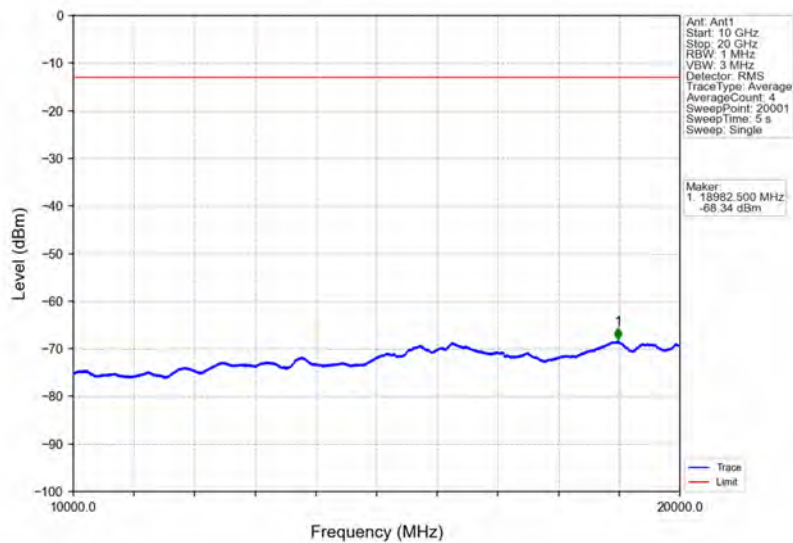
Band25_3MHz_QPSK_MCH_1882.5MHz_RB_1_0_NTNV
