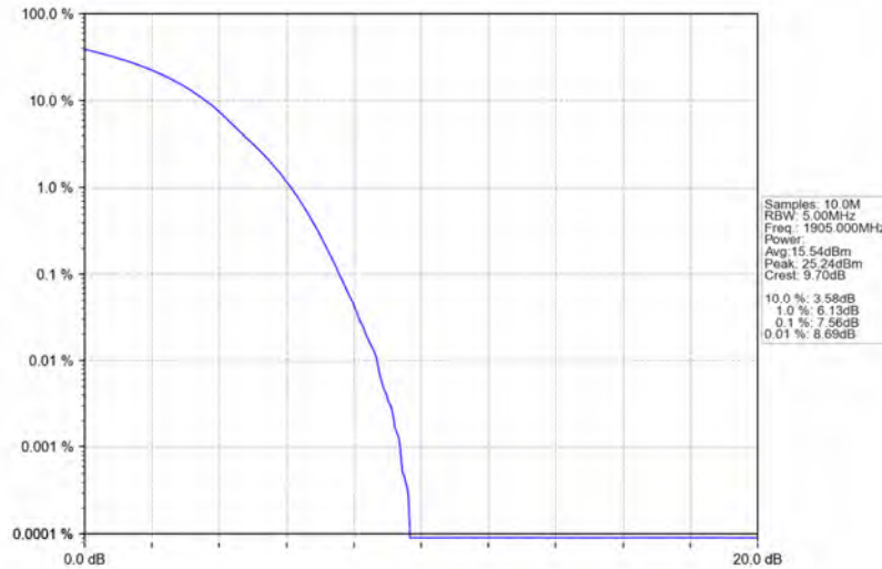
Band25_20MHz_64QAM_HCH_1905MHz_RB_100_0_NTNV
