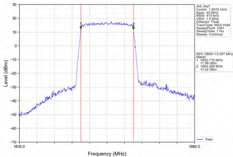
Band25_15MHz_16QAM_LCH_1857.5MHz_RB_75_0_NTNV
