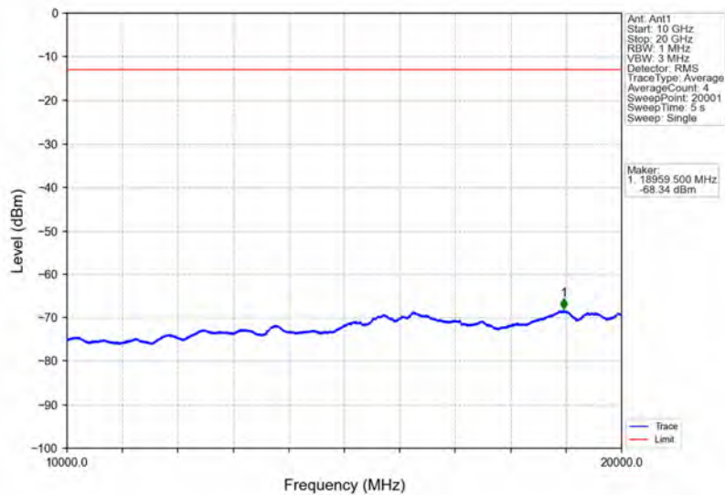
Band25_10MHz_16QAM_LCH_1855MHz_RB_50_0_NTNV
