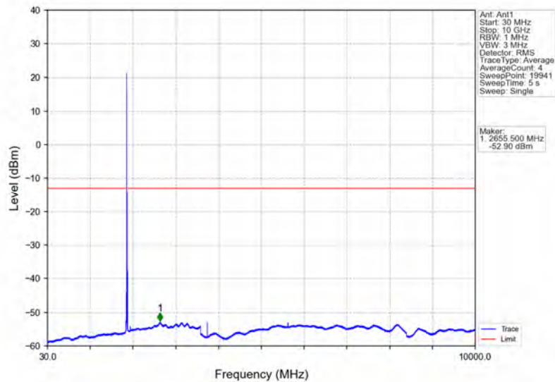
Band25_10MHz_64QAM_MCH_1882.5MHz_RB_1_0_NTNV
