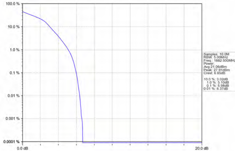
Band25_1.4MHz_16QAM_MCH_1882.5MHz_RB_6_0_NTNV
