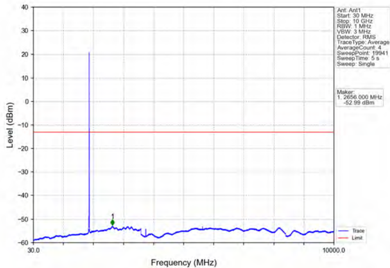
Band25_5MHz_64QAM_MCH_1882.5MHz_RB_1_0_NTNV
