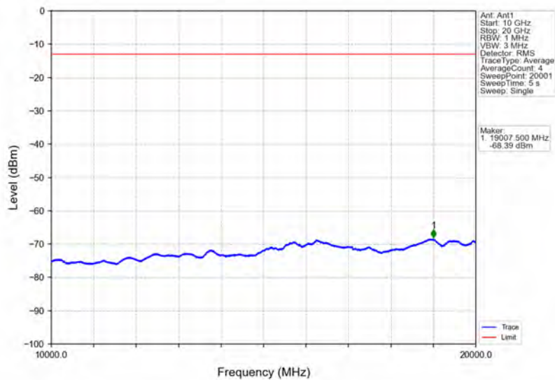
Band25_10MHz_64QAM_MCH_1882.5MHz_RB_1_0_NTNV
