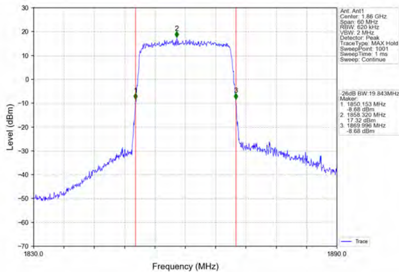
Band25_20MHz_64QAM_LCH_1860MHz_RB_100_0_NTNV
