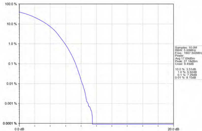
Band25_15MHz_16QAM_HCH_1907.5MHz_RB_75_0_NTNV
