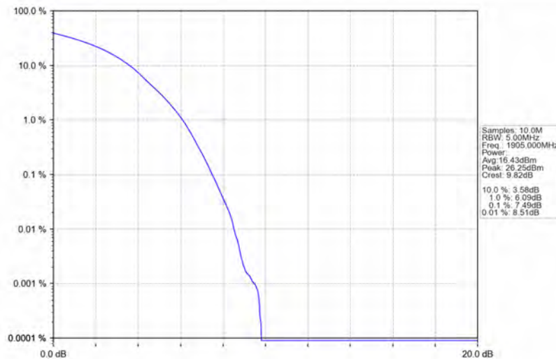
Band25_20MHz_16QAM_HCH_1905MHz_RB_100_0_NTNV
