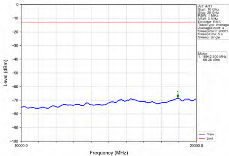
Band25_3MHz_16QAM_MCH_1882.5MHz_RB_1_0_NTNV
