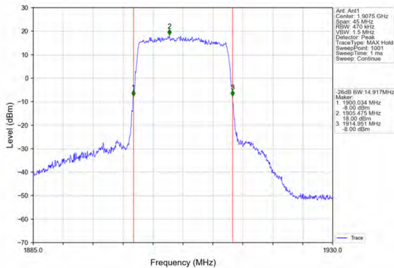
Band25_15MHz_16QAM_HCH_1907.5MHz_RB_75_0_NTNV
