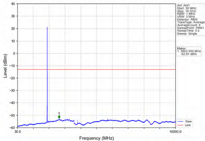
Band25_10MHz_64QAM_HCH_1910MHz_RB_1_0_NTNV
