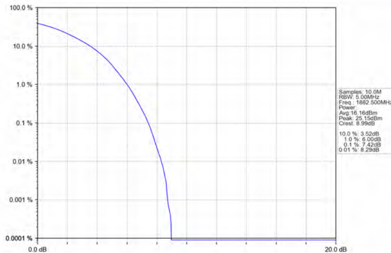
Band25_15MHz_64QAM_MCH_1882.5MHz_RB_75_0_NTNV
