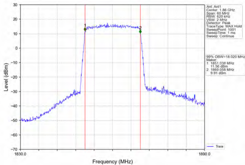
Band25_20MHz_64QAM_LCH_1860MHz_RB_100_0_NTNV
