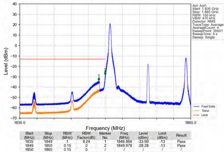
Band25_15MHz_64QAM_LCH_1857.5MHz_RB_1_0_NTNV
