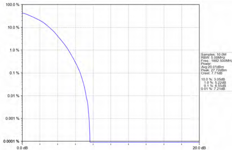
Band25_3MHz_64QAM_MCH_1882.5MHz_RB_15_0_NTNV
