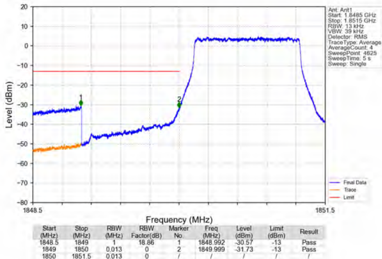
Band25_1.4MHz_QPSK_LCH_1850.7MHz_RB_6_0_NTNV
