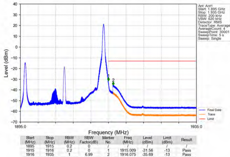
Band25_20MHz_16QAM_HCH_1905MHz_RB_1_99_NTNV
