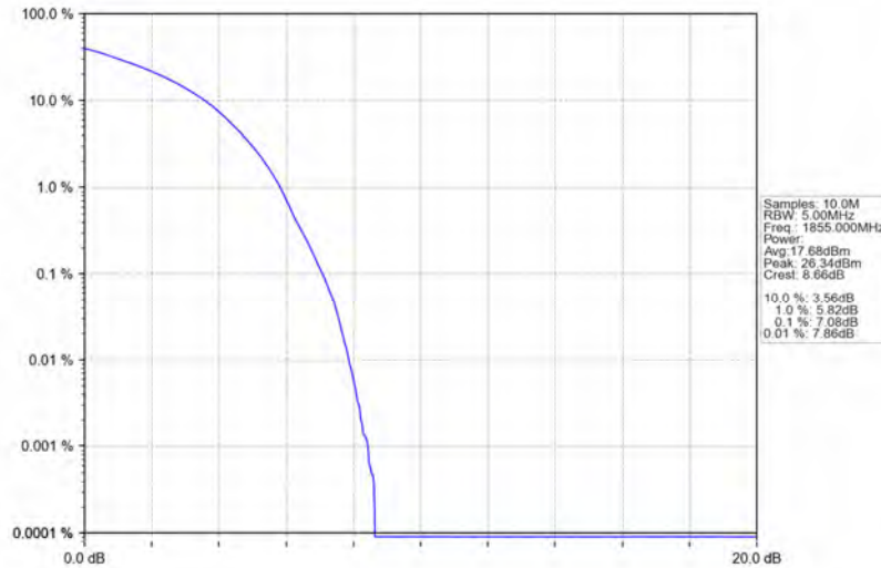
Band25_10MHz_64QAM_LCH_1855MHz_RB_50_0_NTNV
