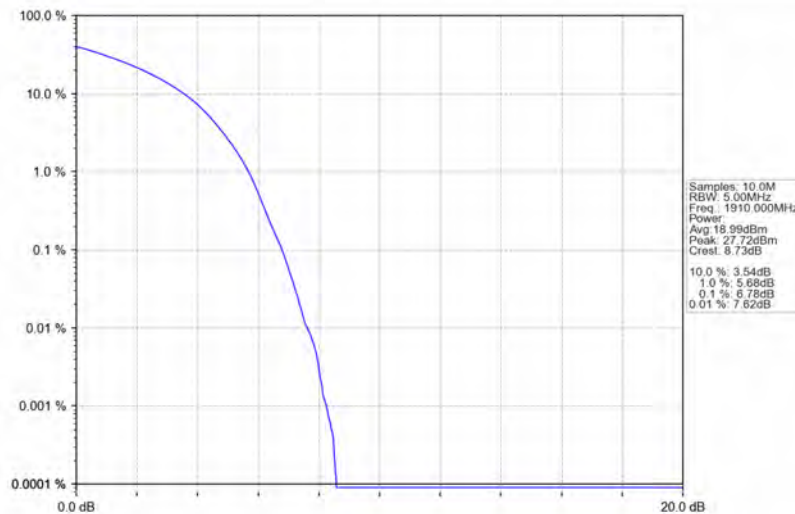
Band25_10MHz_16QAM_HCH_1910MHz_RB_50_0_NTNV
