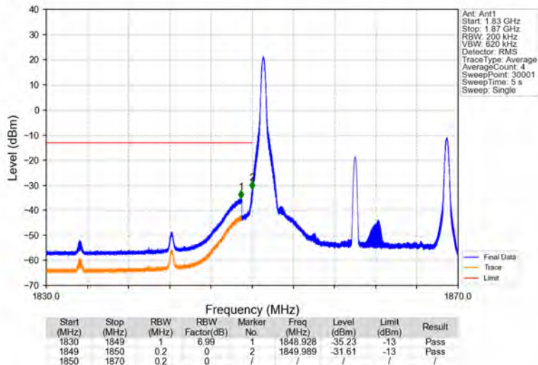
Band25_20MHz_64QAM_LCH_1860MHz_RB_1_0_NTNV
