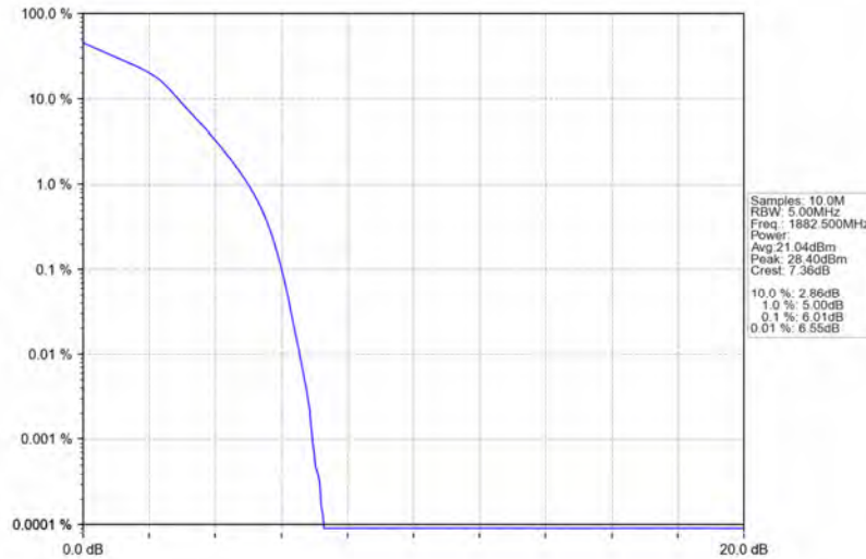
Band25_5MHz_16QAM_MCH_1882.5MHz_RB_25_0_NTNV
