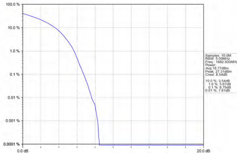
Band25_10MHz_16QAM_MCH_1882.5MHz_RB_50_0_NTNV
