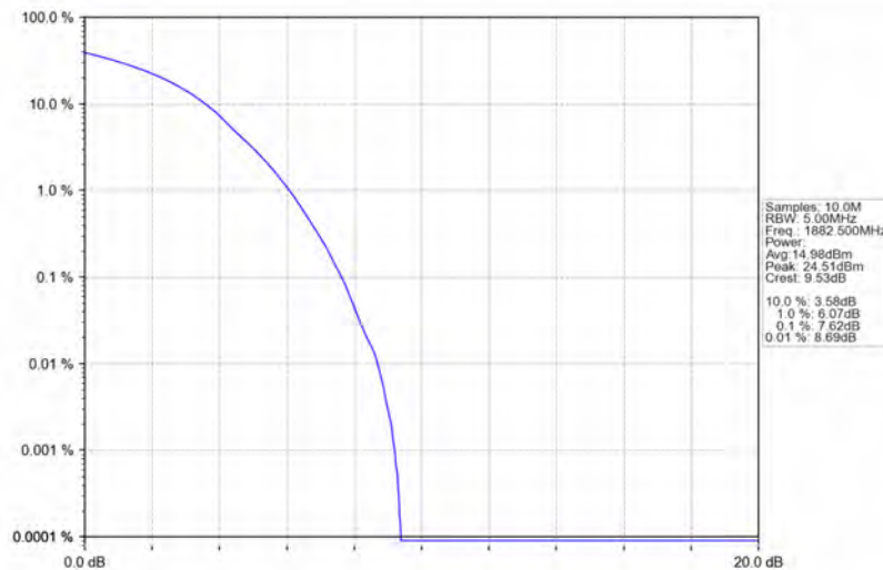
Band25_20MHz_64QAM_MCH_1882.5MHz_RB_100_0_NTNV
