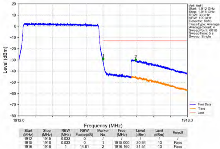
Band25_3MHz_64QAM_HCH_1913.5MHz_RB_15_0_NTNV
