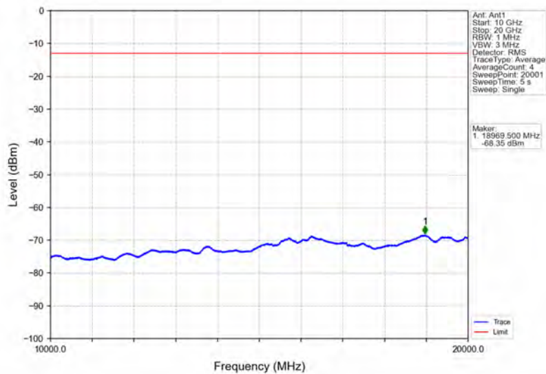
Band25_20MHz_64QAM_HCH_1905MHz_RB_1_0_NTNV
