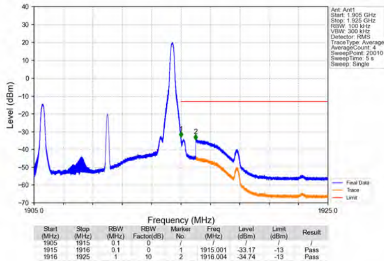
Band25_10MHz_16QAM_HCH_1910MHz_RB_1_49_NTNV
