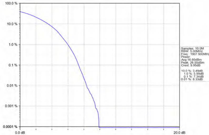
Band25_15MHz_64QAM_HCH_1907.5MHz_RB_75_0_NTNV
