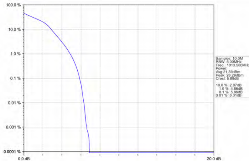
Band25_3MHz_16QAM_HCH_1913.5MHz_RB_15_0_NTNV
