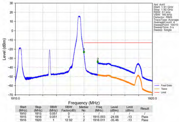
Band25_5MHz_64QAM_HCH_1912.5MHz_RB_1_24_NTNV
