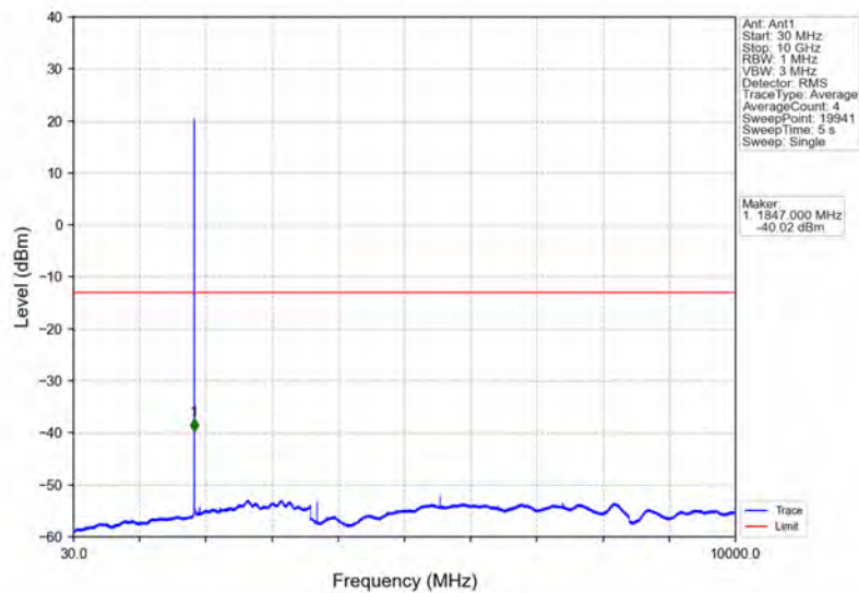
Band25_1.4MHz_64QAM_LCH_1850.7MHz_RB_1_0_NTNV
