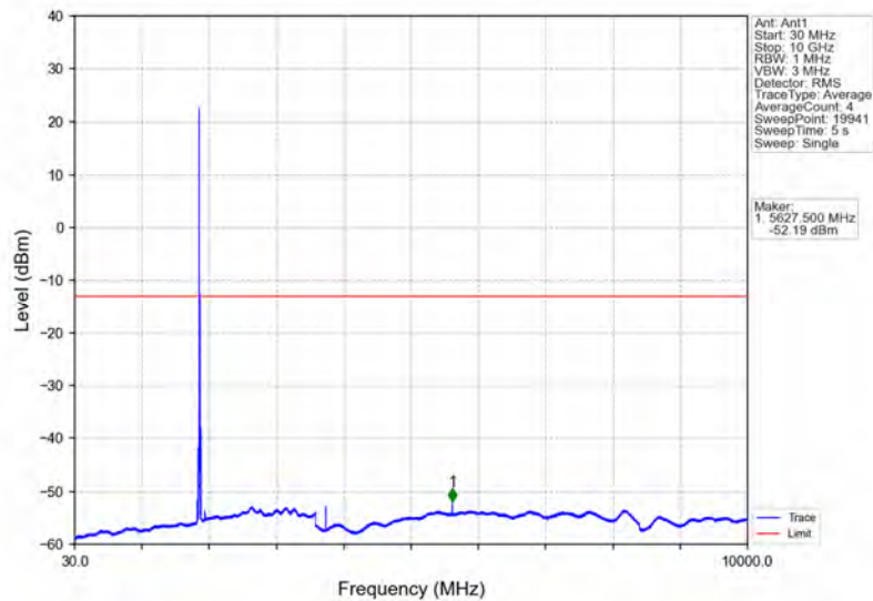
Band25_15MHz_QPSK_MCH_1882.5MHz_RB_1_0_NTNV
