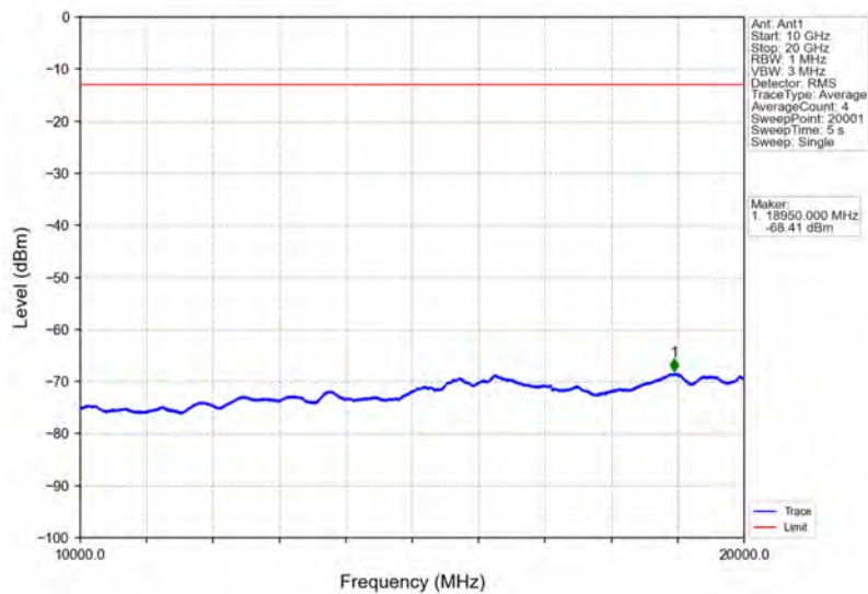
Band25_1.4MHz_16QAM_HCH_1914.3MHz_RB_1_0_NTNV
