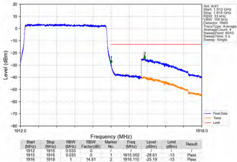
Band25_3MHz_16QAM_HCH_1913.5MHz_RB_15_0_NTNV
