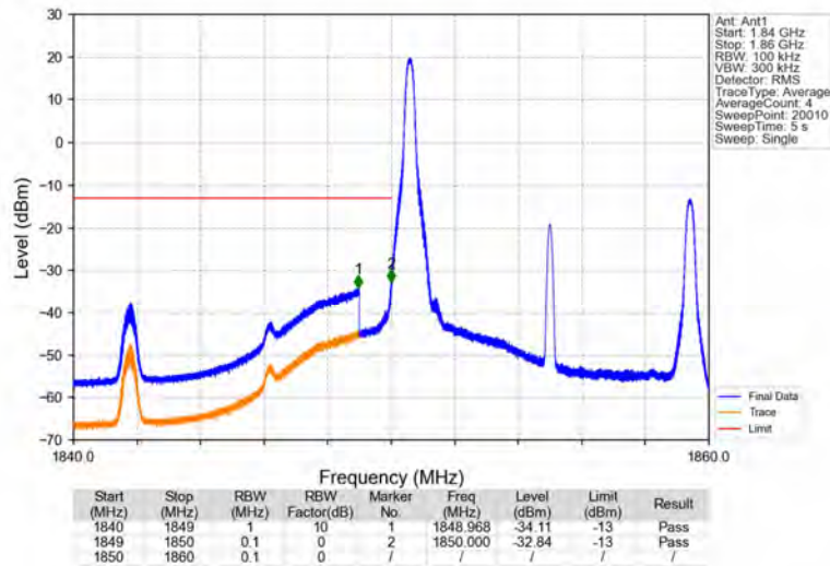
Band25_10MHz_64QAM_LCH_1855MHz_RB_1_0_NTNV
