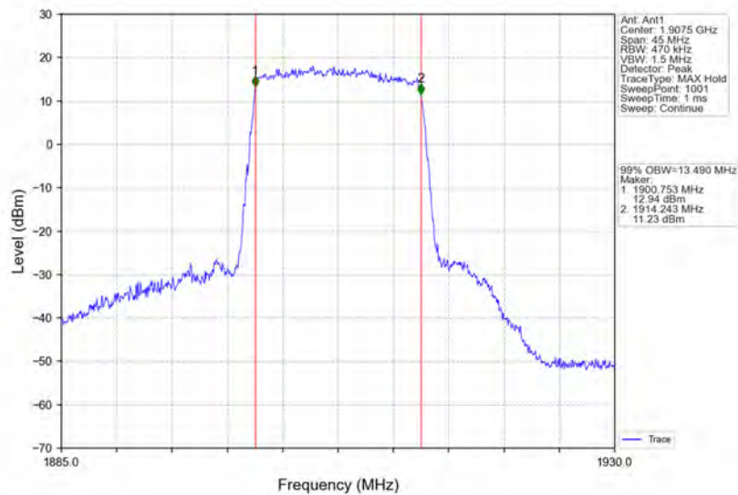
Band25_15MHz_16QAM_HCH_1907.5MHz_RB_75_0_NTNV
