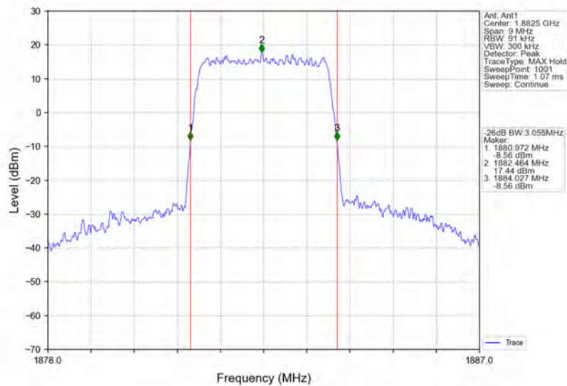
Band25_3MHz_16QAM_MCH_1882.5MHz_RB_15_0_NTNV
