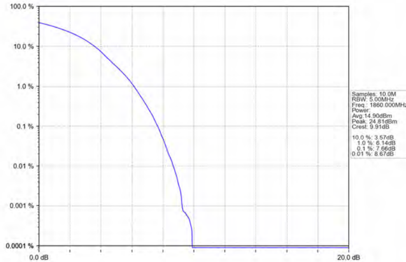
Band25_20MHz_64QAM_LCH_1860MHz_RB_100_0_NTNV
