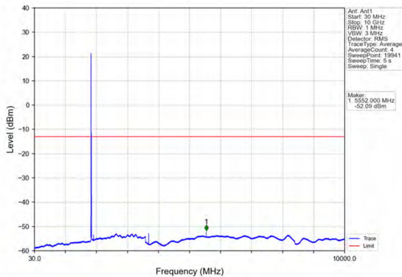
Band25_10MHz_64QAM_LCH_1855MHz_RB_1_0_NTNV
