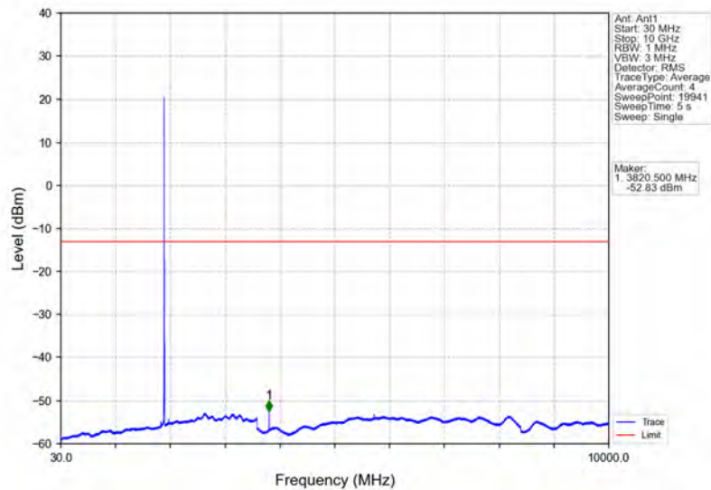
Band25_5MHz_64QAM_HCH_1912.5MHz_RB_1_0_NTNV
