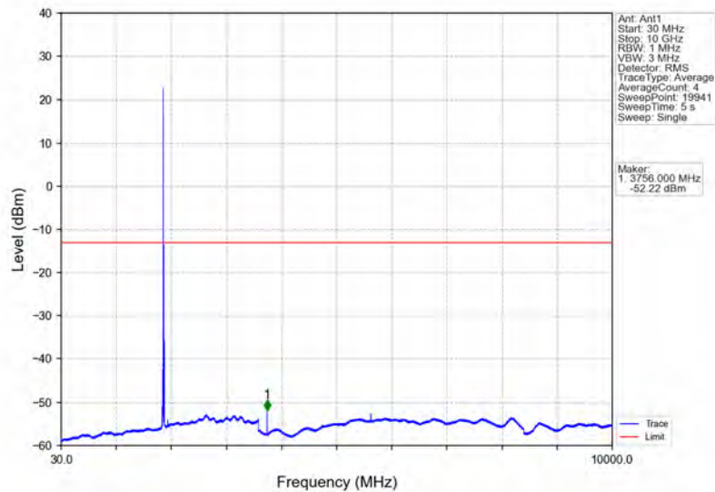
Band25_10MHz_16QAM_MCH_1882.5MHz_RB_1_0_NTNV
