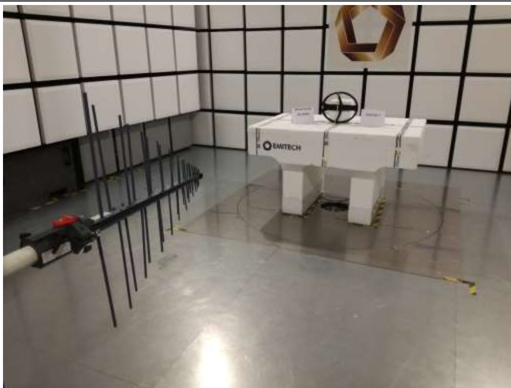
TEST SETUP PHOTO(S) – RX MODE – 200MHZ TO 1GHz
