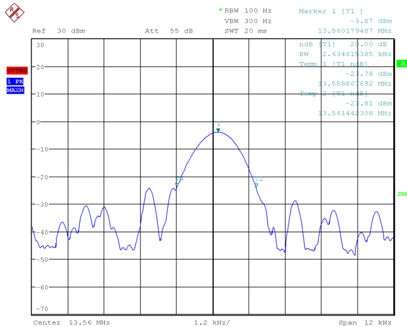
Figure B-9: Measurement results for 20dB Bandwidth
