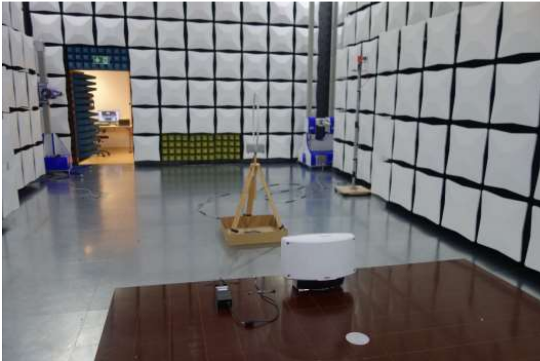
Antenna in parallel to axis position. Picture 1
