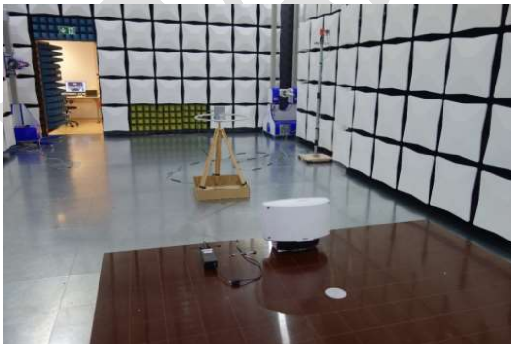
Antenna in parallel to floor position. Picture 2
