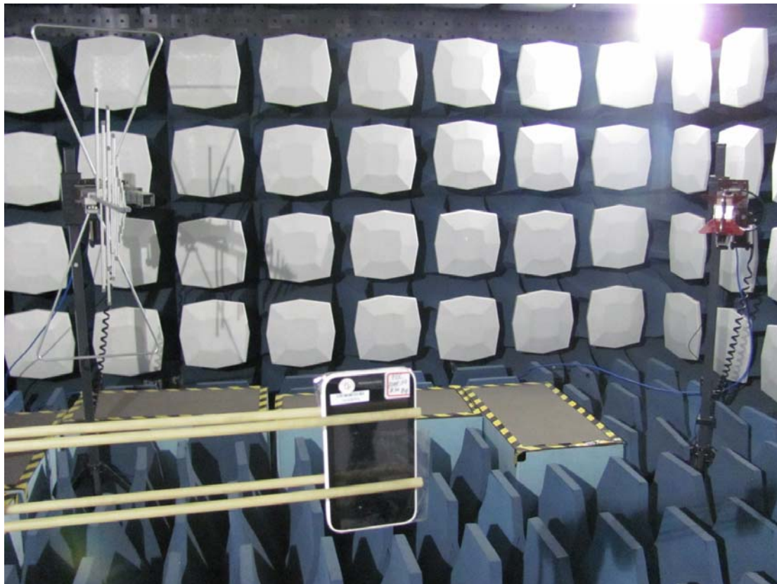
Pic F-1 Radiated Spurious Emission Test Layout
