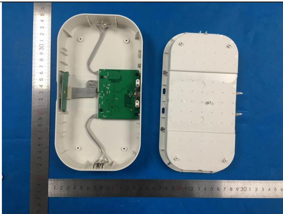
Photo 1 (For model WS-10)
