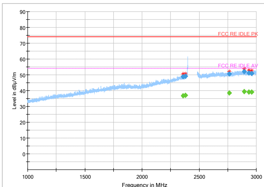
Fig.46 Radiated Spurious Emission (802.11b,Ch1,1GHz~3GHz)
