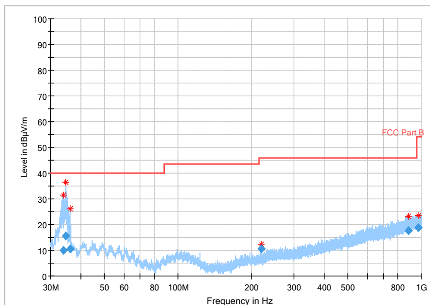
Fig.54 Radiated Spurious Emission (802.11b,Ch1,30MHz~1GHz)
