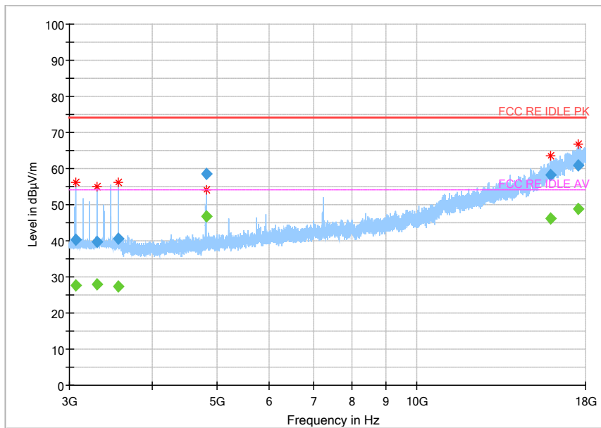
Fig.47 Radiated Spurious Emission (802.11b,Ch1,3GHz~18GHz)
