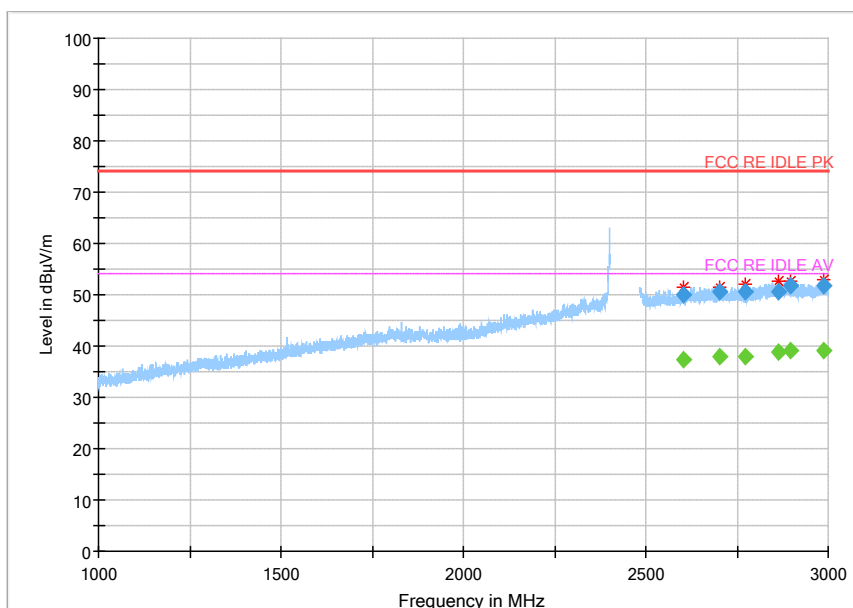
Fig.55 Radiated Spurious Emission (802.11b,Ch1, 1GHz~3GHz))
