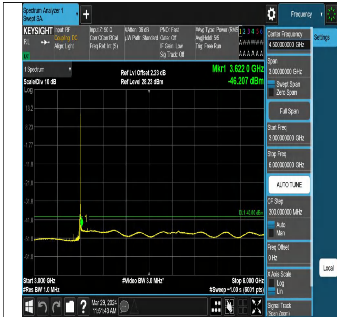
Band43_5MHz_QPSK_43615_1RB#0_3000~6000_3000~600
