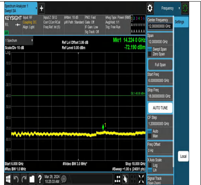
Band43_15MHz_QPSK_43665_1RB#0_6000~18000_6000~1
