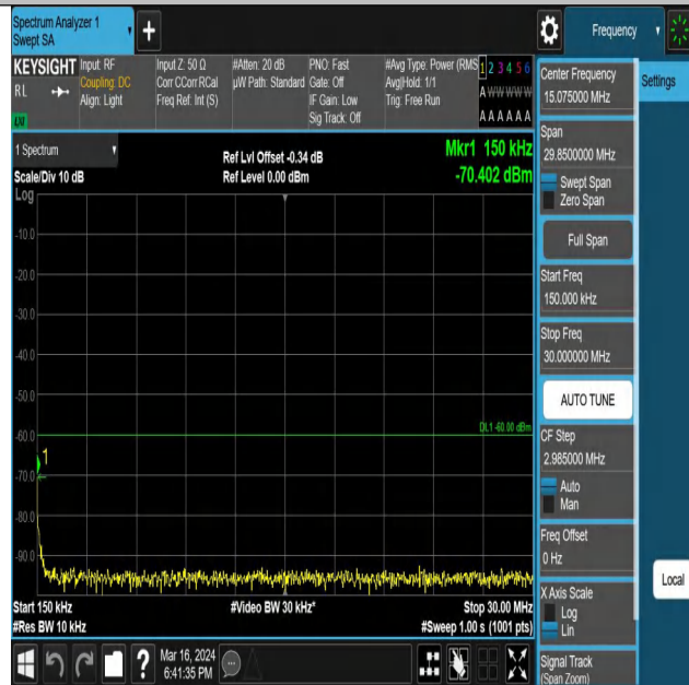
Band43_10MHz_QPSK_44090_1RB#0_0.15~30_0.15~30
