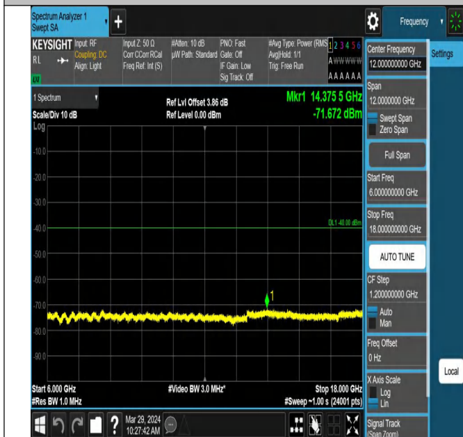
Band43_20MHz_QPSK_43690_1RB#0_6000~18000_6000~1
