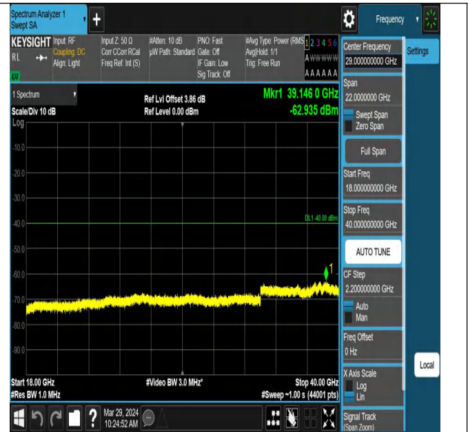
Band43_5MHz_QPSK_44090_1RB#0_18000~40000_18000~40000
