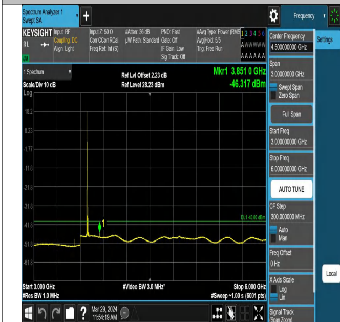
Band43_15MHz_QPSK_44515_1RB#0_3000~6000_3000~6000
