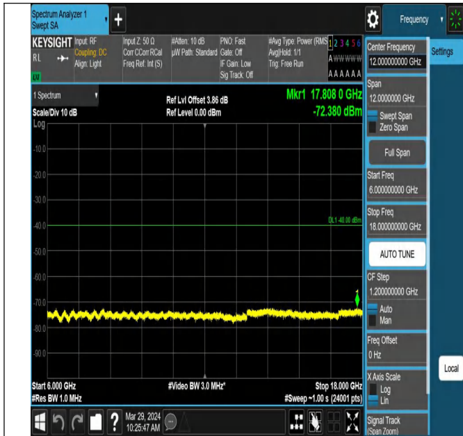
Band43_15MHz_QPSK_44090_1RB#0_6000~18000_6000~18000
