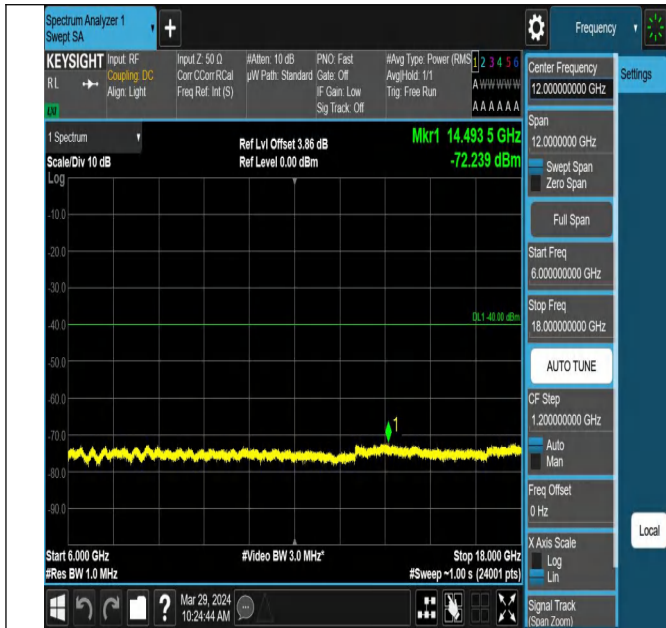
Band43_5MHz_QPSK_44090_1RB#0_6000~18000_6000~18000
