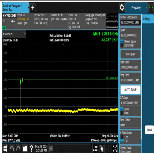
Band43_10MHz_QPSK_44090_1RB#0_6000~18000_6000~18000 8000
