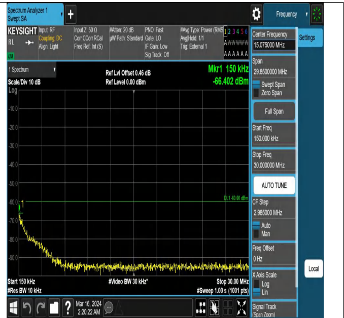
Band43_20MHz_QPSK_44090_1RB#0_0.15~30_0.15~30
