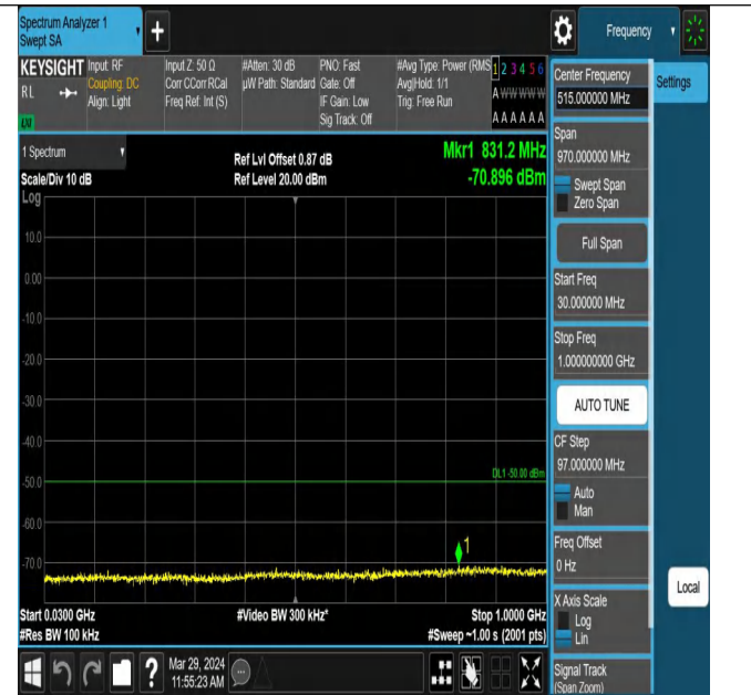
Band43_20MHz_QPSK_44490_1RB#0_30~1000_30~1000
