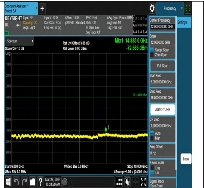
Band43_5MHz_QPSK_43615_1RB#0_6000~18000_6000~18
