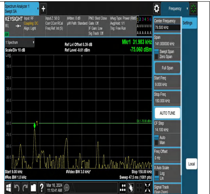
Band43_20MHz_QPSK_43690_1RB#0_0.009~0.15_0.009~0. 15
