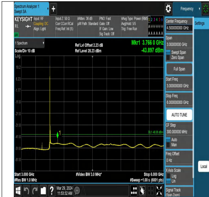
Band43_15MHz_QPSK_43665_1RB#0_3000~6000_3000~60
