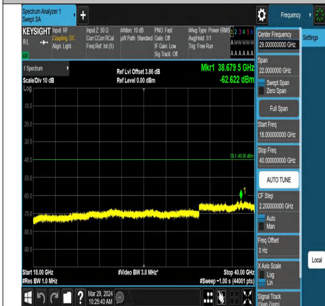
Band43_15MHz_QPSK_43665_1RB#0_18000~40000_18000
