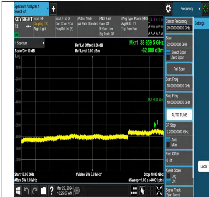
Band43_5MHz_QPSK_44565_1RB#0_18000~40000_18000~40000
