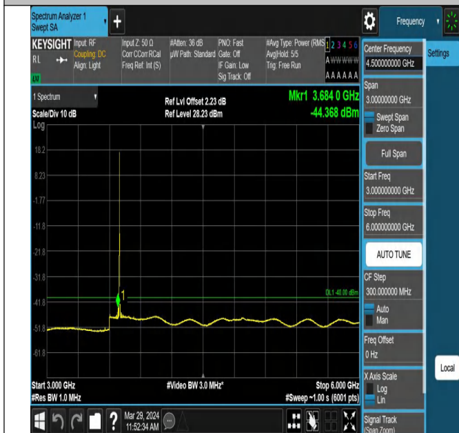
Band43_5MHz_QPSK_44565_1RB#0_3000~6000_3000~600
