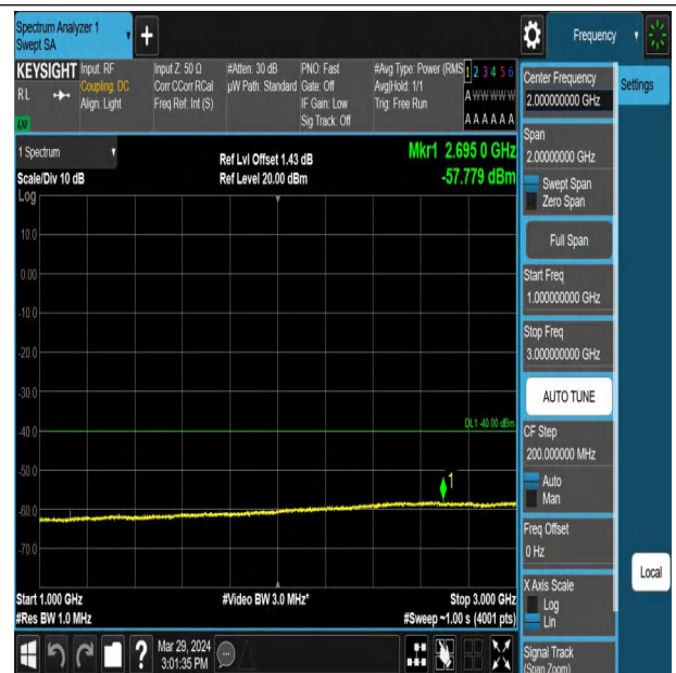
Band43_10MHz_QPSK_44090_1RB#0_1000~3000_1000~3000 00
