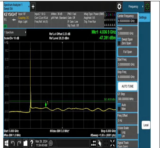
Band43_20MHz_QPSK_43690_1RB#0_3000~6000_3000~60
