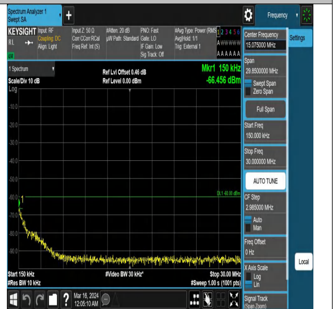
Band43_5MHz_QPSK_44565_1RB#0_0.15~30_0.15~30
