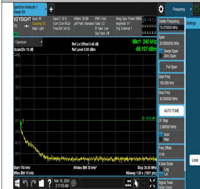
Band43_20MHz_QPSK_43690_1RB#0_0.15~30_0.15~30
