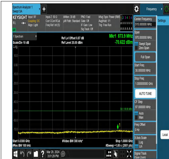
Band43_10MHz_QPSK_44090_1RB#0_30~1000_30~1000
