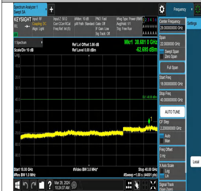
Band43_5MHz_QPSK_43615_1RB#0_18000~40000_18000~
