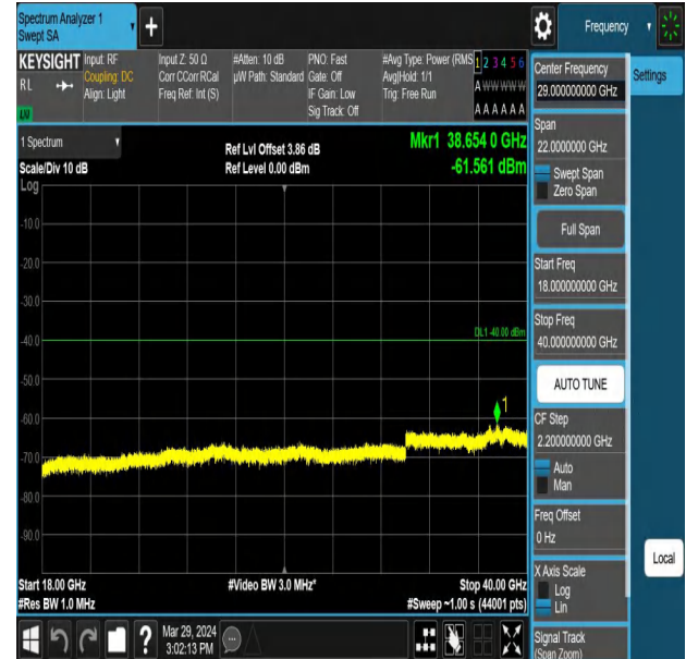
Band43_10MHz_QPSK_43640_1RB#0_18000~40000_18000~40000
