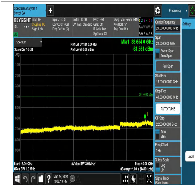
Band43_10MHz_QPSK_44090_1RB#0_18000~40000_18000~40000
