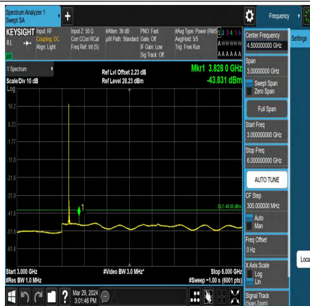
Band43_10MHz_QPSK_44090_1RB#0_3000~6000_3000~6000 00
