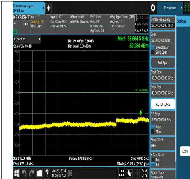
Band43_15MHz_QPSK_44515_1RB#0_18000~40000_18000 ~40000
