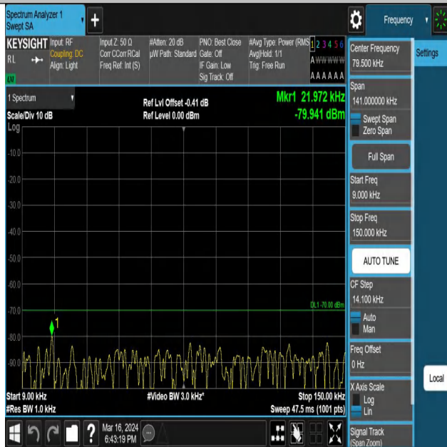
Band43_10MHz_QPSK_44090_1RB#0_0.009~0.15_0.009~0.15
