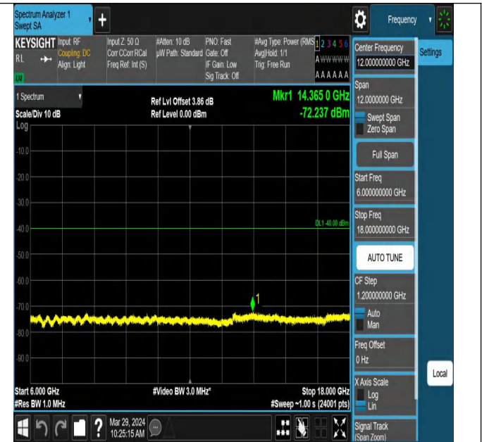
Band43_10MHz_QPSK_40640_1RB#0_6000~18000_6000~1
