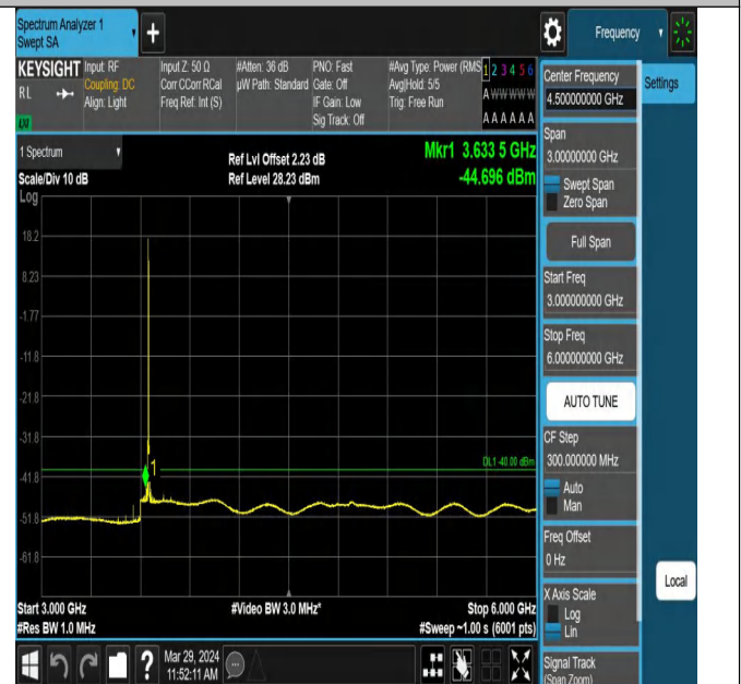
Band43_5MHz_QPSK_44090_1RB#0_3000~6000_3000~600
