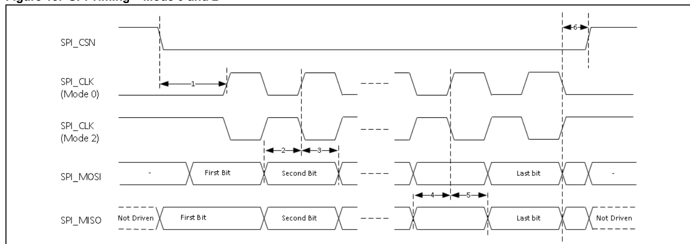
Figure 13. SPI Timing – Mode 0 and 2
