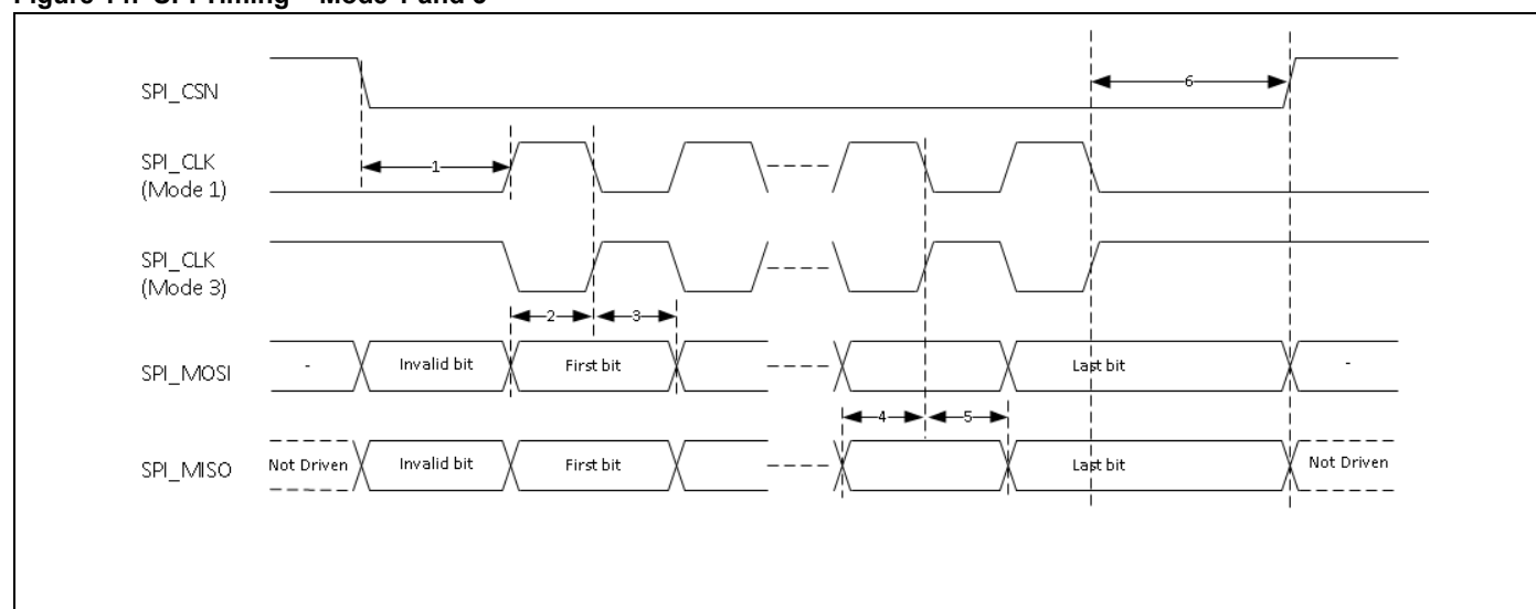
Figure 14. SPI Timing – Mode 1 and 3
