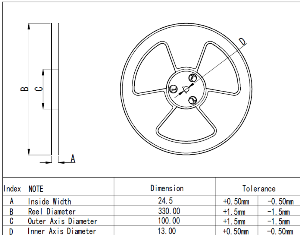
Figure 22. Reel Dimensions
