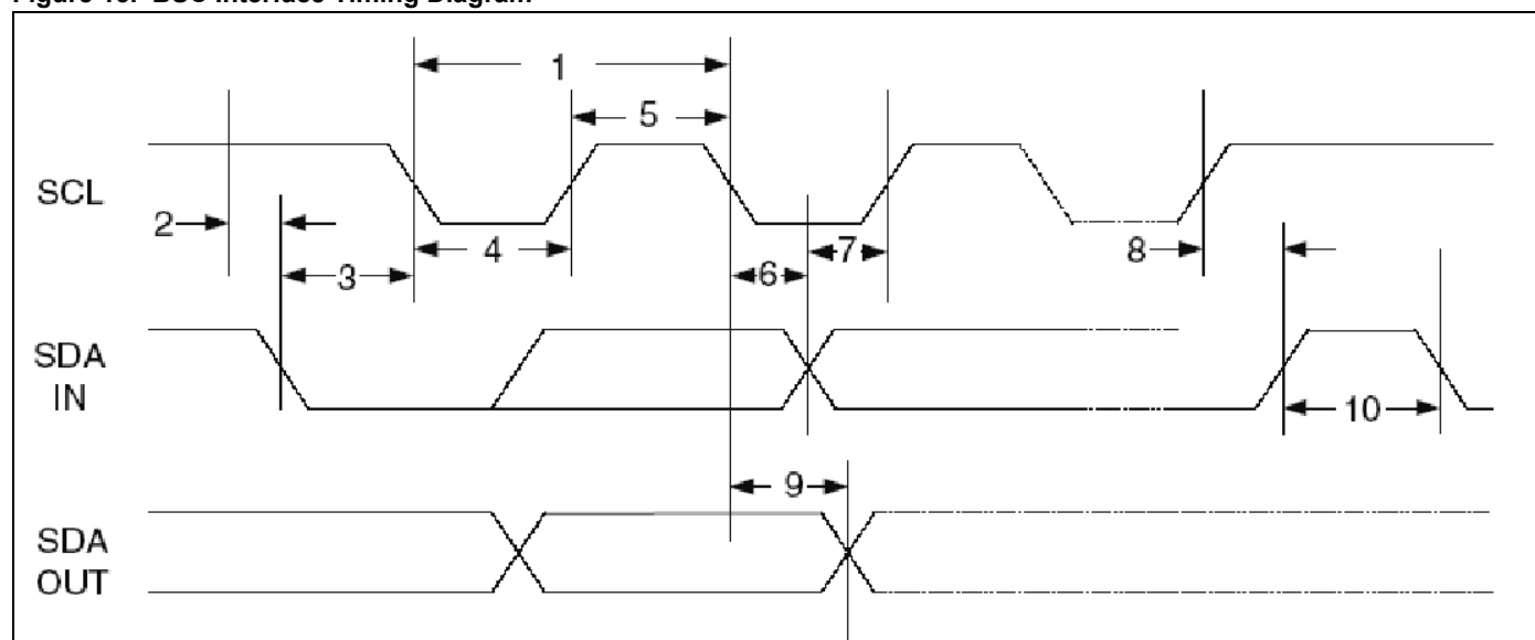
Figure 15. BSC Interface Timing Diagram
