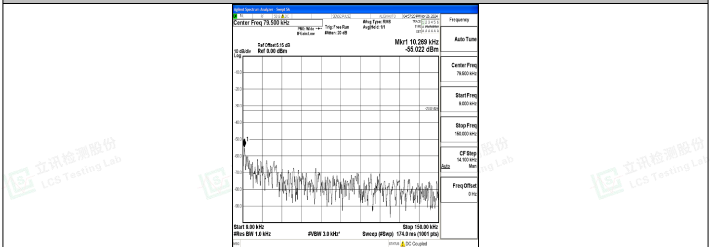
Band5_5MHz_QPSK_20425_1RB#0_0.009~0.15_0.009~0.15
