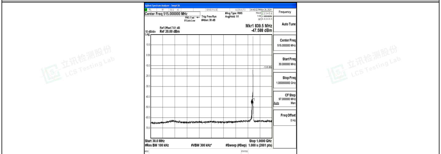
Band5_3MHz_QPSK_20635_1RB#0_30~1000_30~1000
