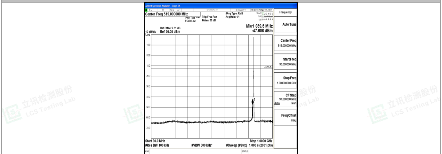
Band5_3MHz_16QAM_20635_1RB#0_30~1000_30~1000
