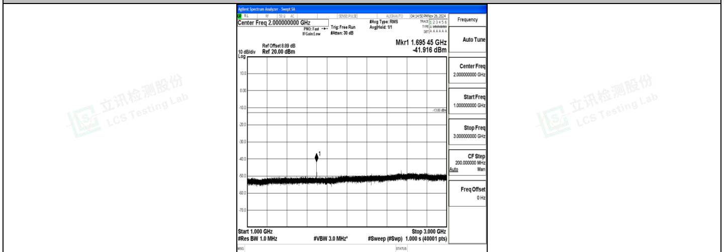
Band5_1.4MHz_16QAM_20643_1RB#0_1000~3000_1000~3000
