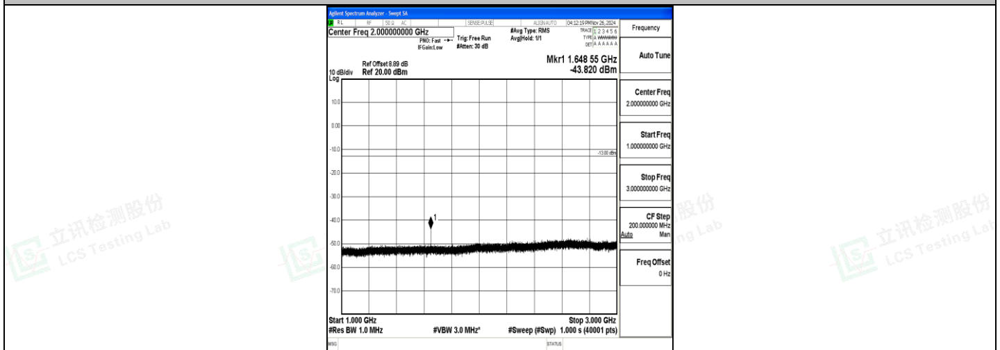
Band5_1.4MHz_QPSK_20407_1RB#0_1000~3000_1000~3000
