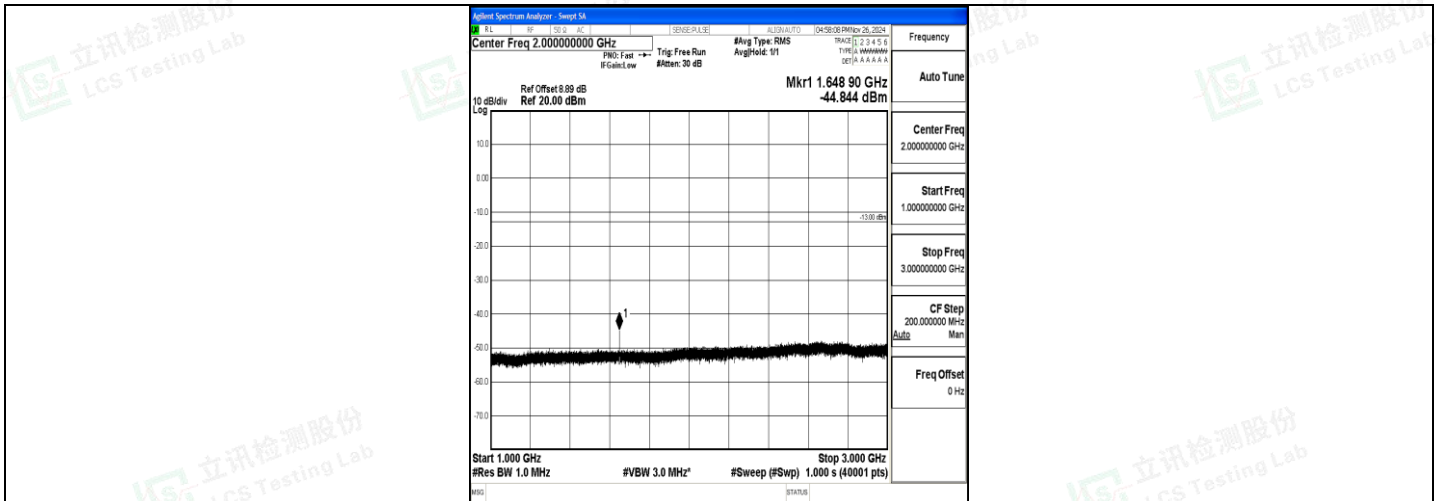
Band5_5MHz_16QAM_20425_1RB#0_1000~3000_1000~3000
