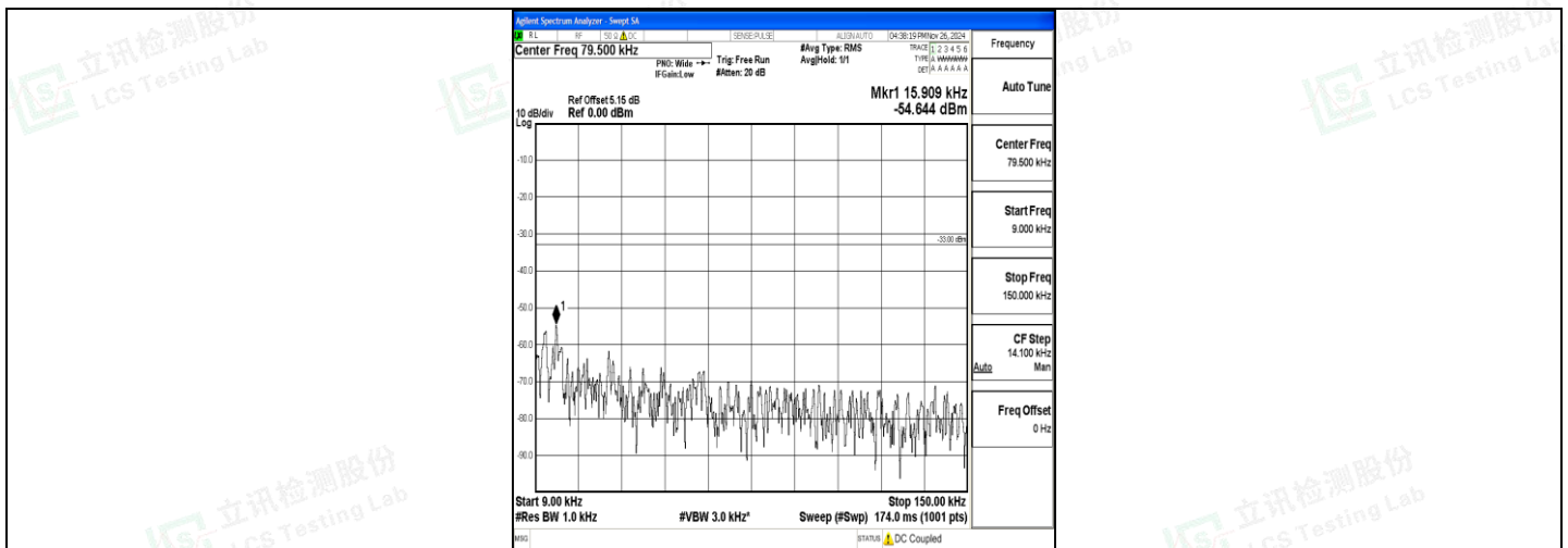
Band5_3MHz_16QAM_20415_1RB#0_0.009~0.15_0.009~0.15
