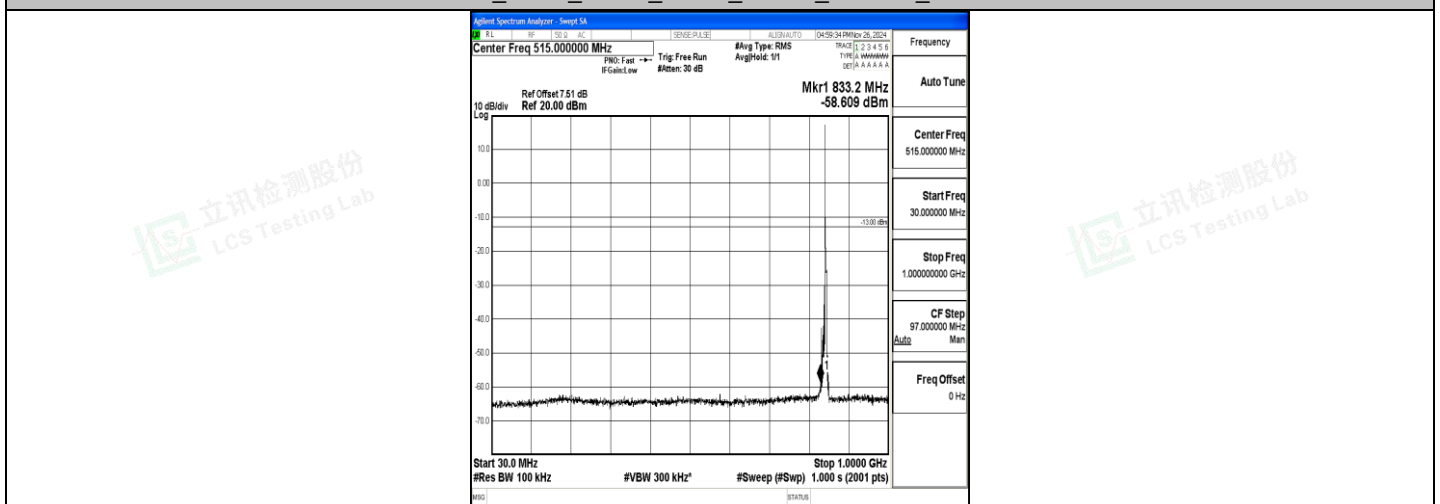
Band5_5MHz_QPSK_20625_1RB#0_30~1000_30~1000
