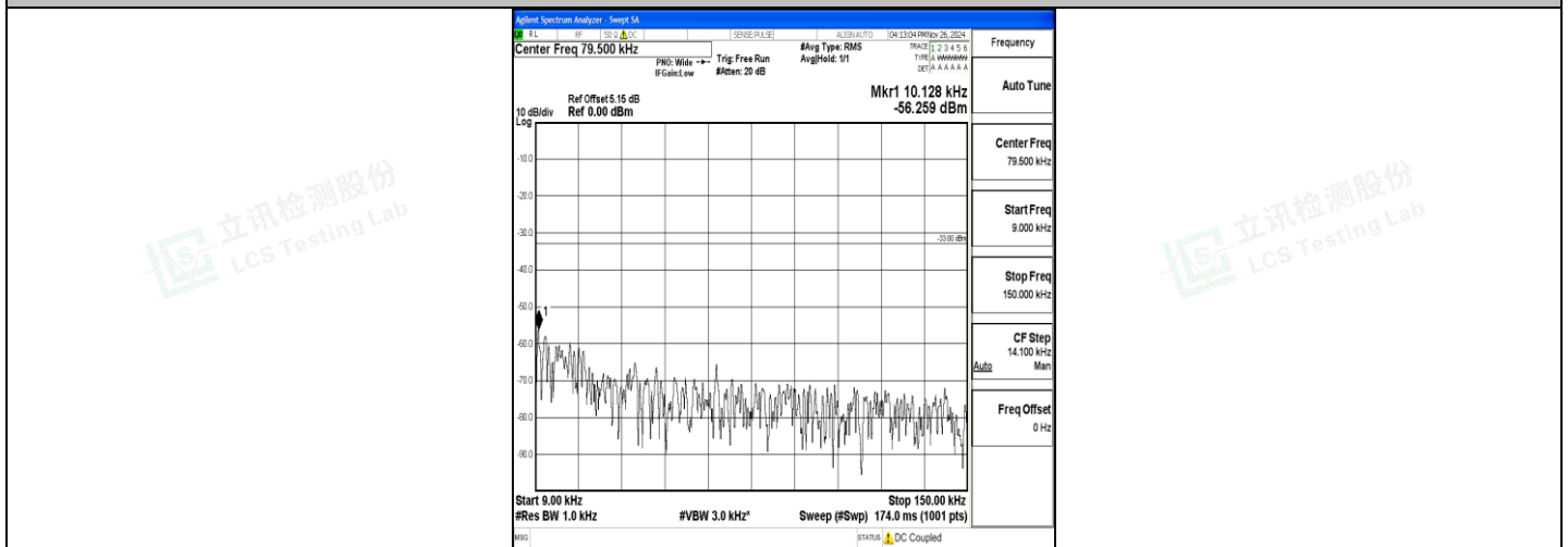
Band5_1.4MHz_QPSK_20525_1RB#0_0.009~0.15_0.009~0.15
