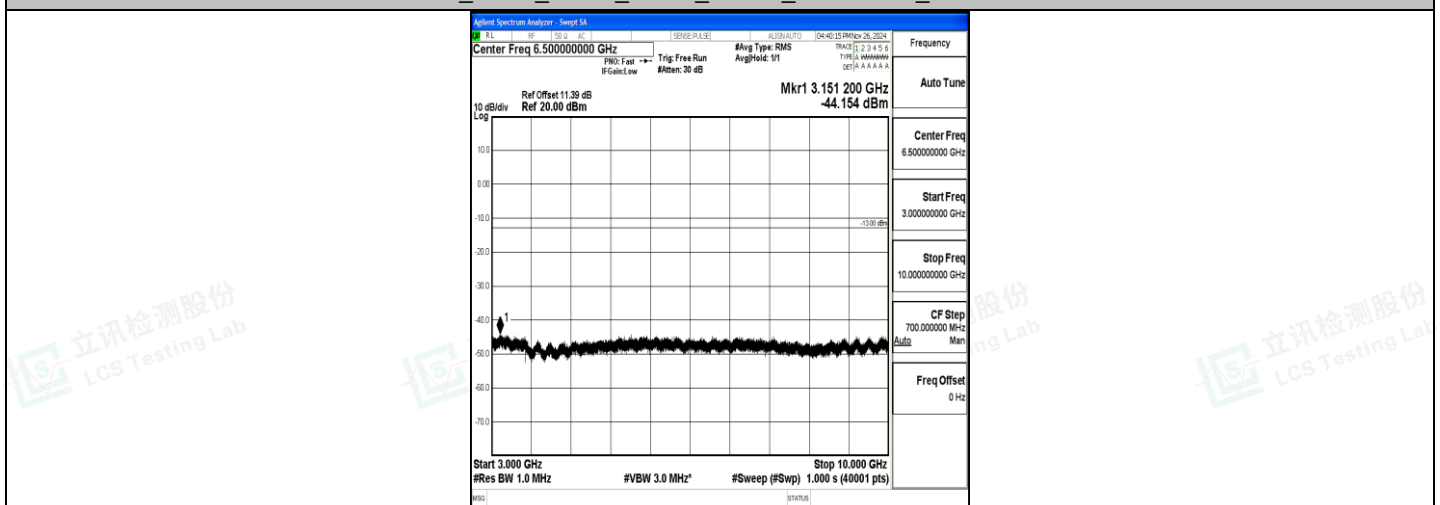
Band5_3MHz_QPSK_20635_1RB#0_3000~10000_3000~10000
