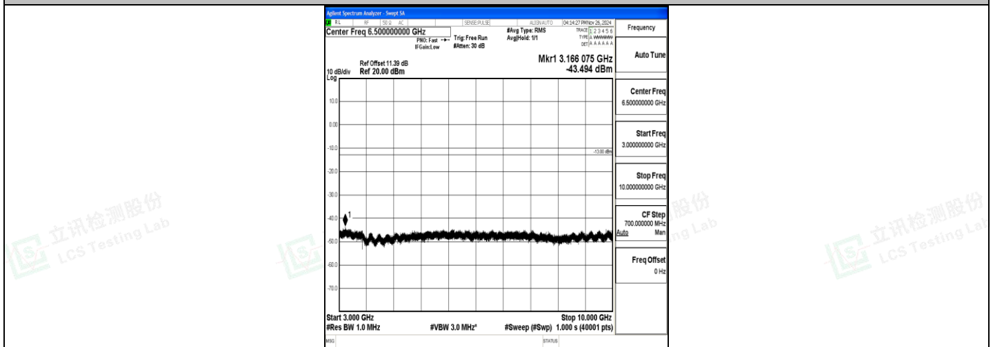
Band5_1.4MHz_QPSK_20643_1RB#0_3000~10000_3000~10000
