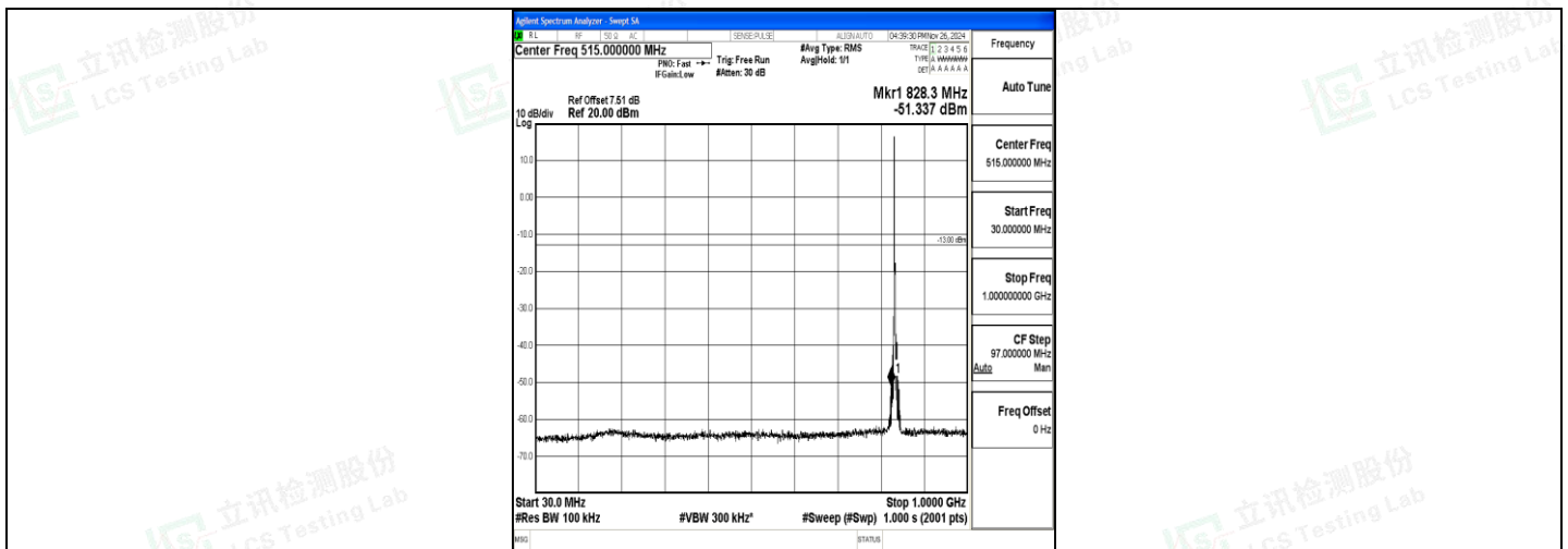
Band5_3MHz_16QAM_20525_1RB#0_30~1000_30~1000
