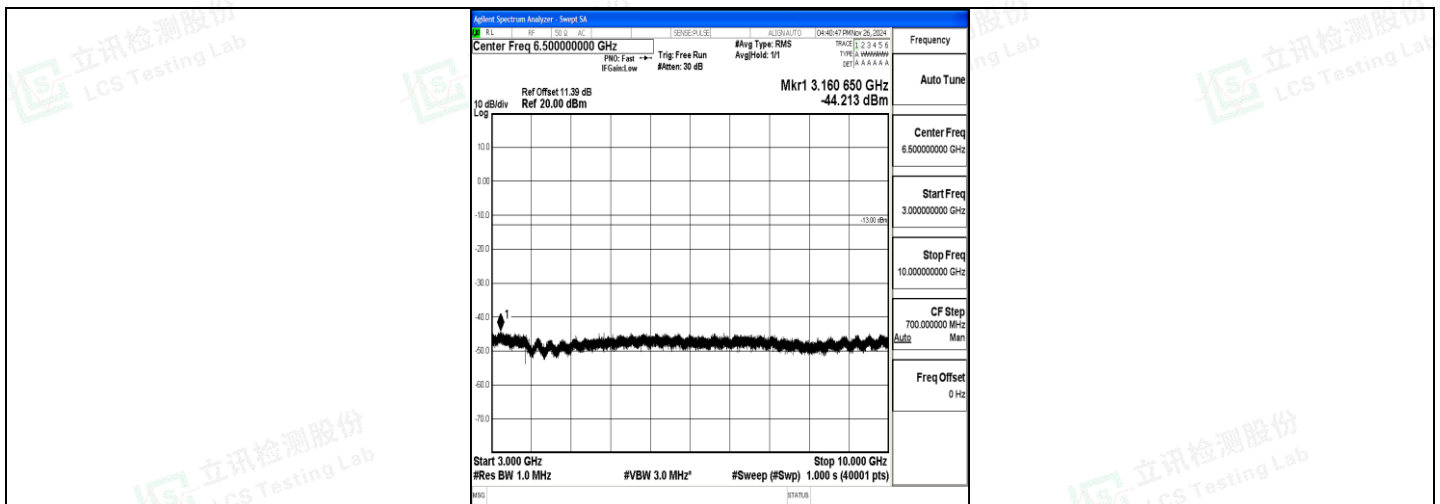
Band5_3MHz_16QAM_20635_1RB#0_3000~10000_3000~10000
