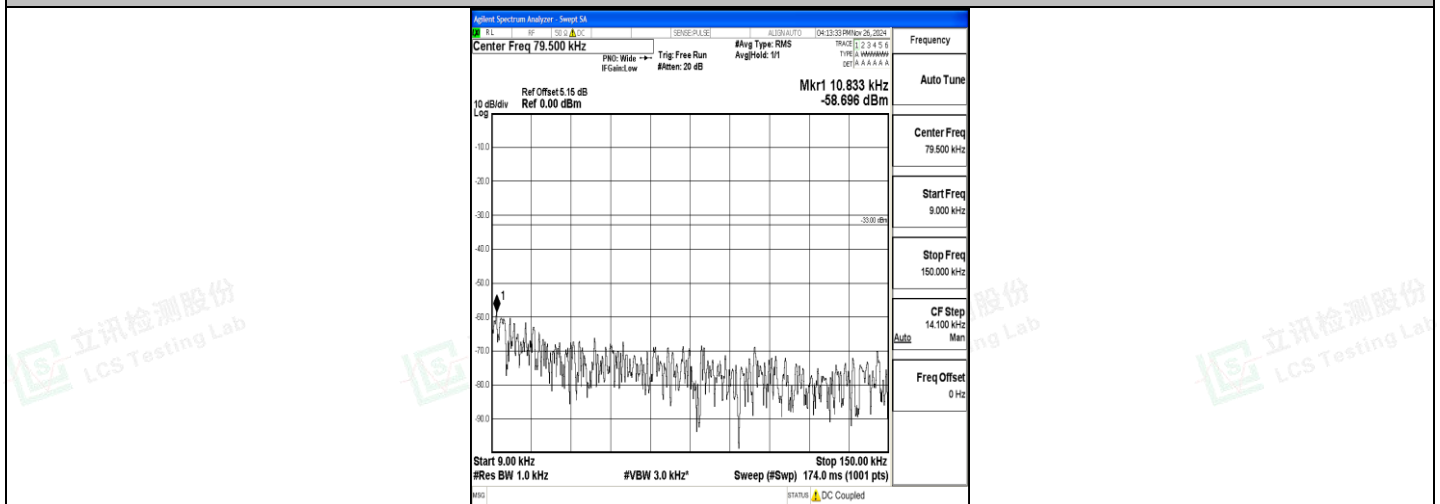
Band5_1.4MHz_16QAM_20525_1RB#0_0.009~0.15_0.009~0.15
