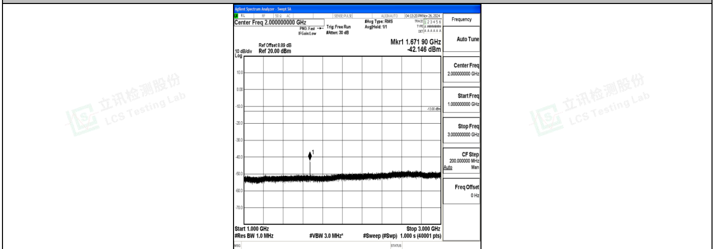
Band5_1.4MHz_QPSK_20525_1RB#0_1000~3000_1000~3000
