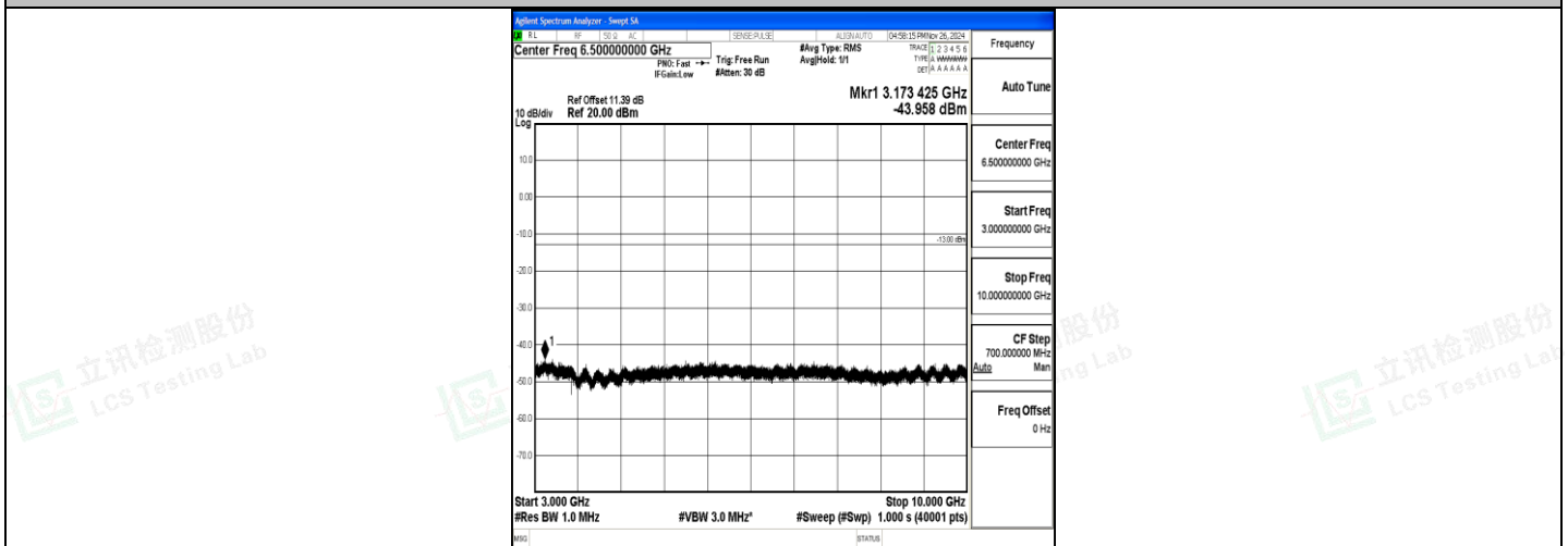
Band5_5MHz_16QAM_20425_1RB#0_3000~10000_3000~10000
