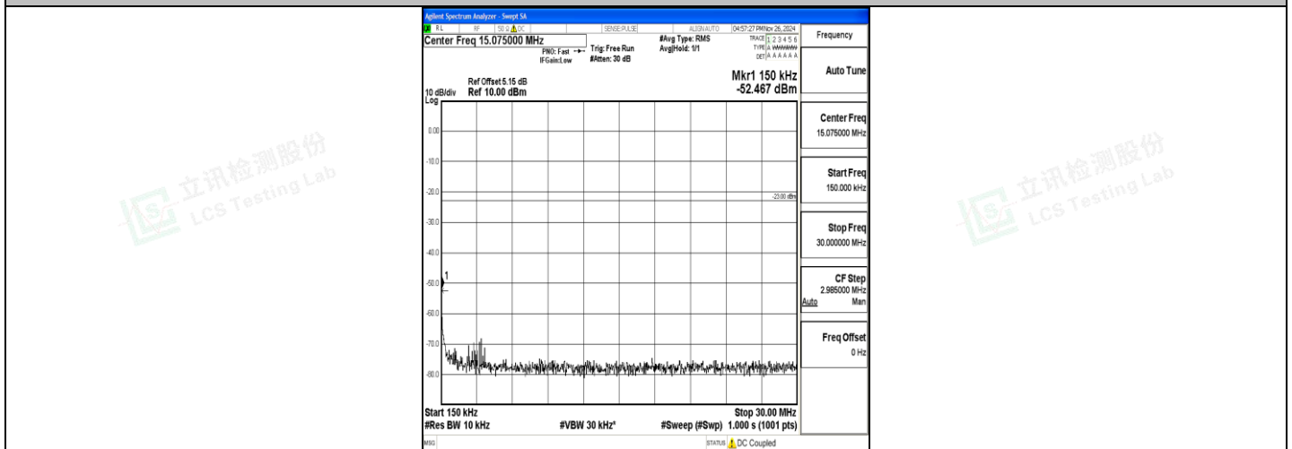
Band5_5MHz_QPSK_20425_1RB#0_0.15~30_0.15~30
