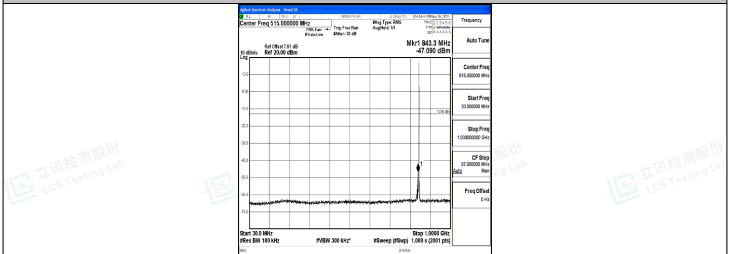
Band5_1.4MHz_16QAM_20643_1RB#0_30~1000_30~1000
