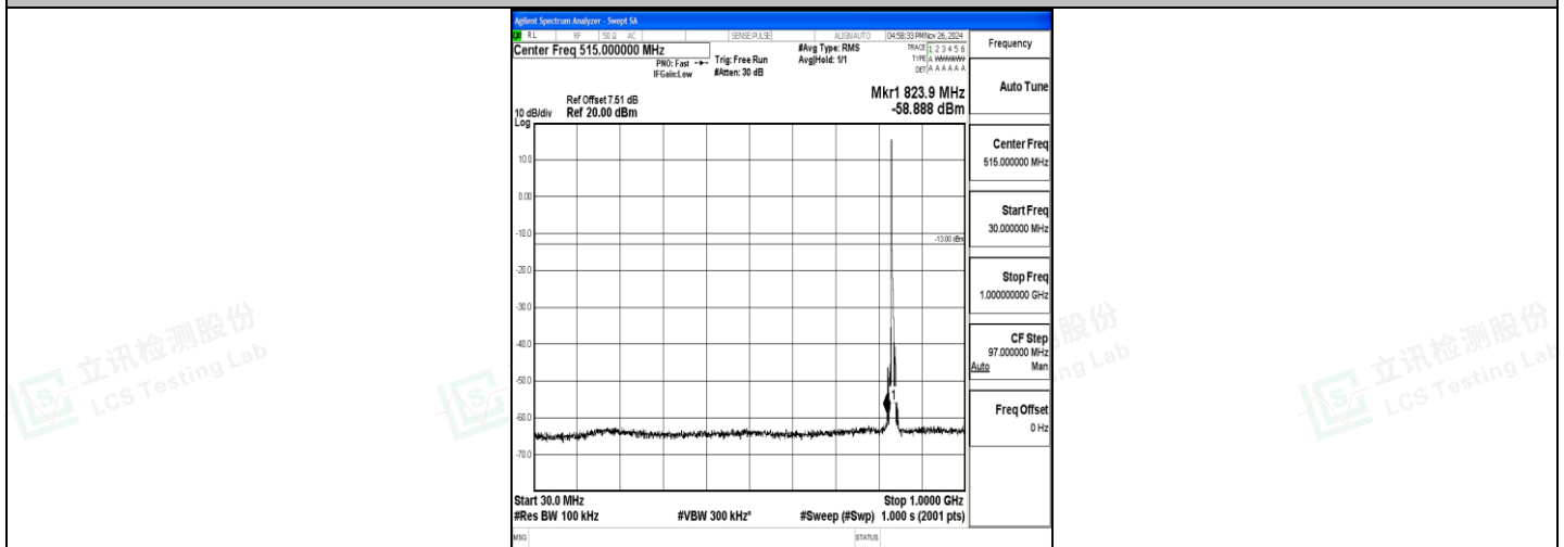
Band5_5MHz_QPSK_20525_1RB#0_30~1000_30~1000
