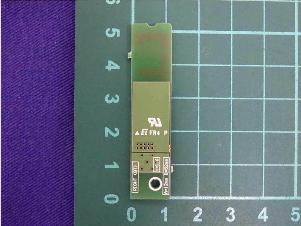
(51) EUT Photo
