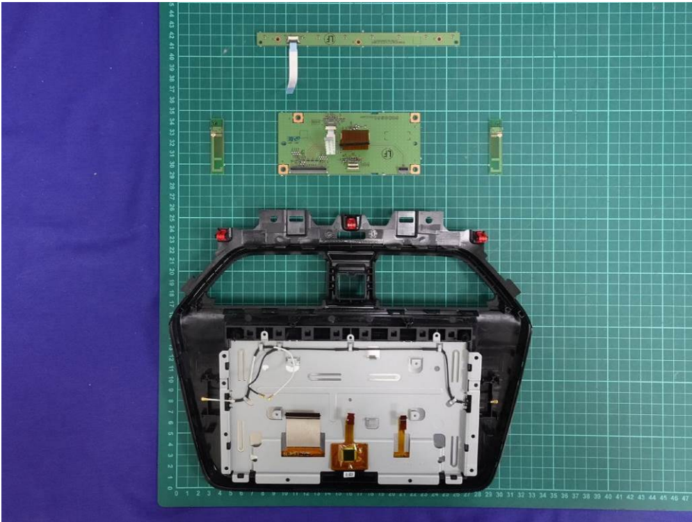
(43) EUT Photo
