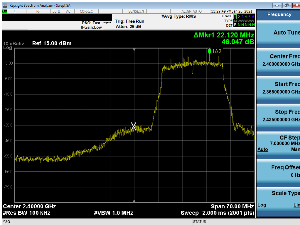
Plot 7-29. Band Edge Plot (802.11n (2.4GHz) – Ch. 2)
