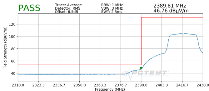
Plot 7-46. Radiated Restricted Lower Band Edge Measurement (Average)
