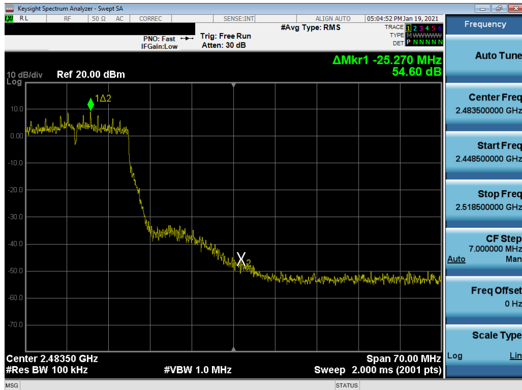
Plot 7-30. Band Edge Plot (802.11n (2.4GHz) – Ch. 10)
