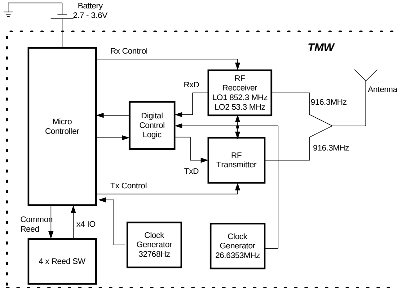
Figure 1: TMW Block Diagram
