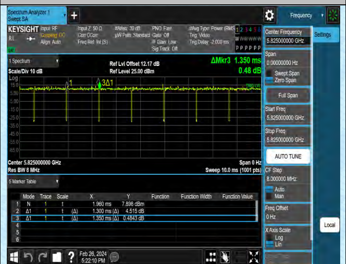
NTNV-11N20MIMO-Ant2-5825
