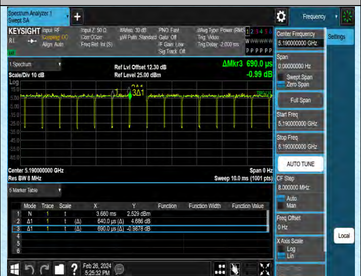
NTNV-11N40MIMO-Ant2-5190
