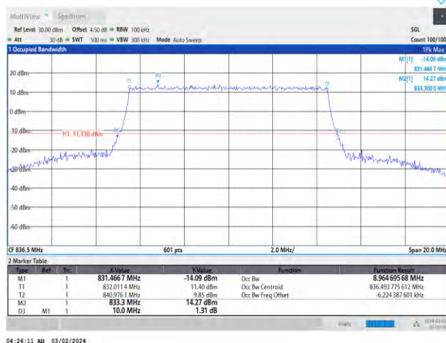
Band26-10MHz-256QAM-26915-50RB#0
