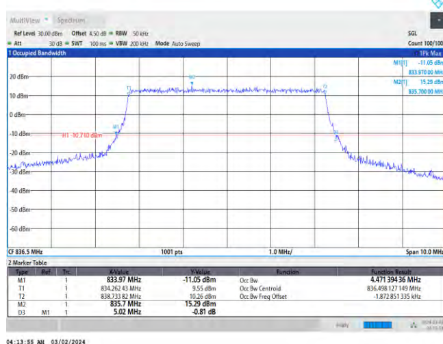
Band26-5MHz-64QAM-26915-25RB#0
