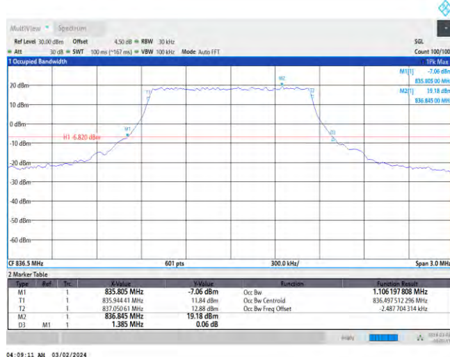
Band26-1.4MHz-64QAM-26915-6RB#0
