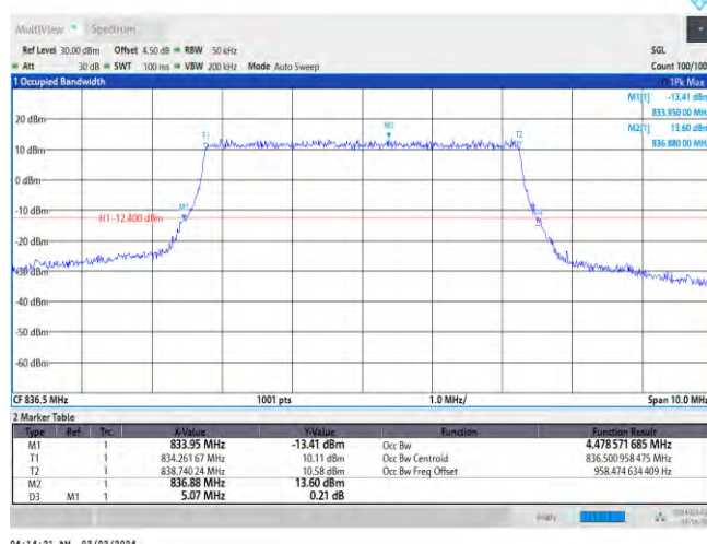
Band26-5MHz-256QAM-26915-25RB#0
