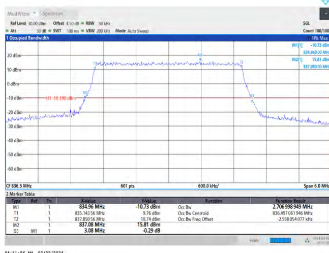
Band26-3MHz-256QAM-26915-15RB#0
