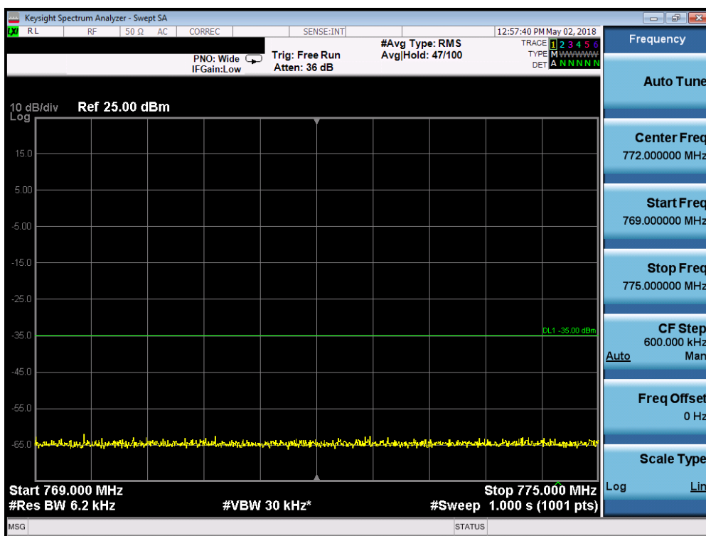
Plot 7-13. Lower Emission Mask Band Edge Plot (Band 14 - 10.0MHz QPSK - Full RB Configuration)
