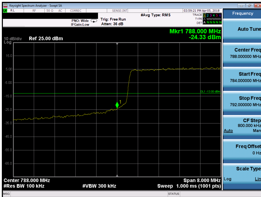
Plot 7-12. Lower Band Edge Plot (Band 14 - 10.0MHz QPSK - Full RB Configuration)
