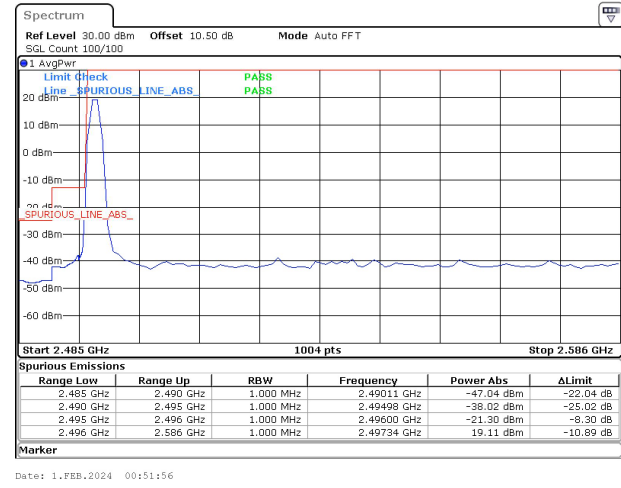
90MHz_30kHz_2541MHz_DFT-s-OFDM QPSK_RB1@0~-21.30 dBm
