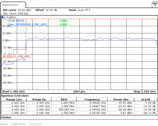
60MHz_30kHz_2526MHz_DFT-s-OFDM QPSK_RB162@0&-32.93 dBm
