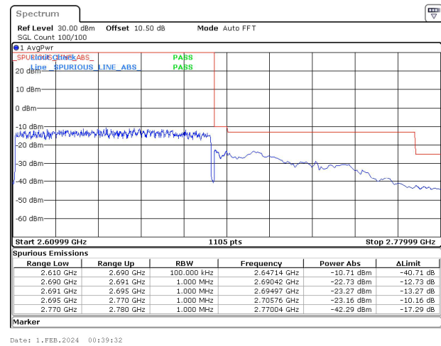
80MHz_30kHz_2649.99MHz_DFT-s-OFDM QPSK_RB216@0~-23.16 dBm
