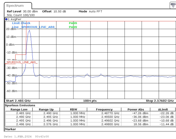
80MHz_30kHz_2536.02MHz_DFT-s-OFDM QPSK_RB1@0&-23.68 dBm
