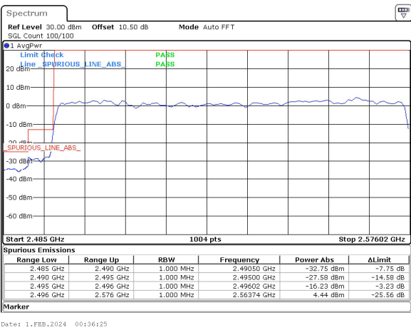
80MHz_30kHz_2536.02MHz_DFT-s-OFDM QPSK_RB216@0&-16.23 dBm
