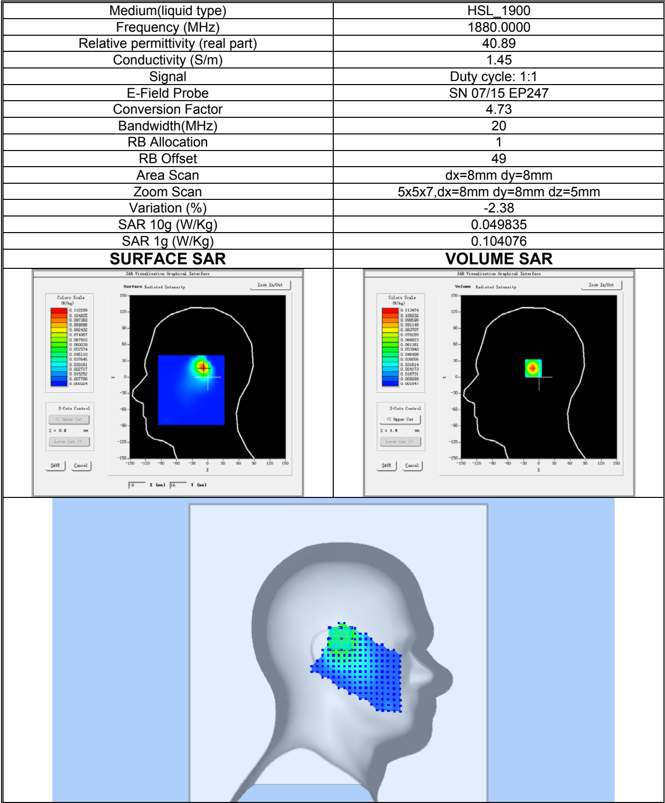
Plot 14:LTE BAND 2, Middle channel (Left Head Tilt) Product Description:Mobile Phone Test Date: 2019-12-25
