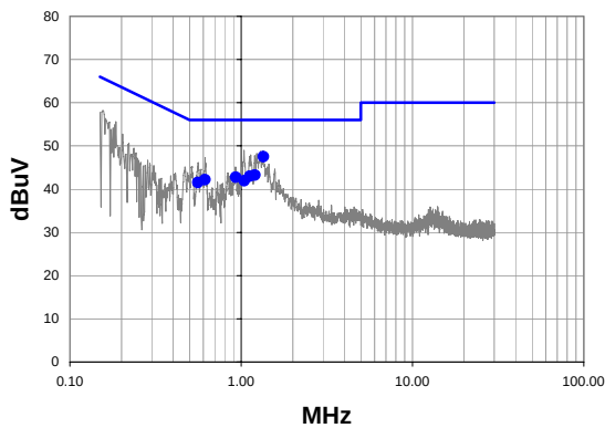
Quasi-Peak
