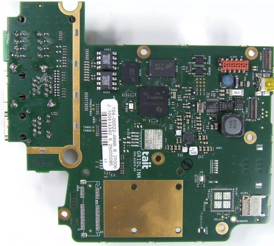
Photograph 02: Main PCB top
