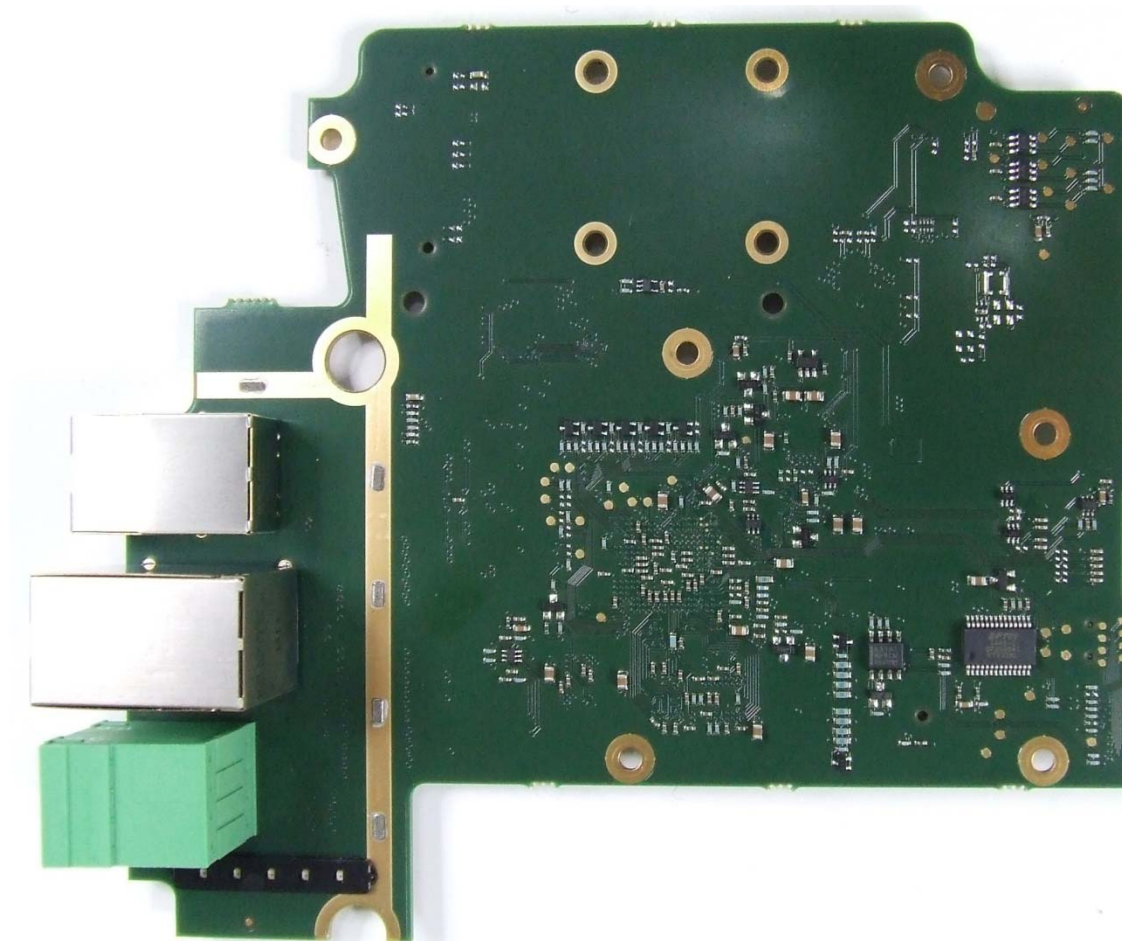
Photograph 03: Main PCB bottom
