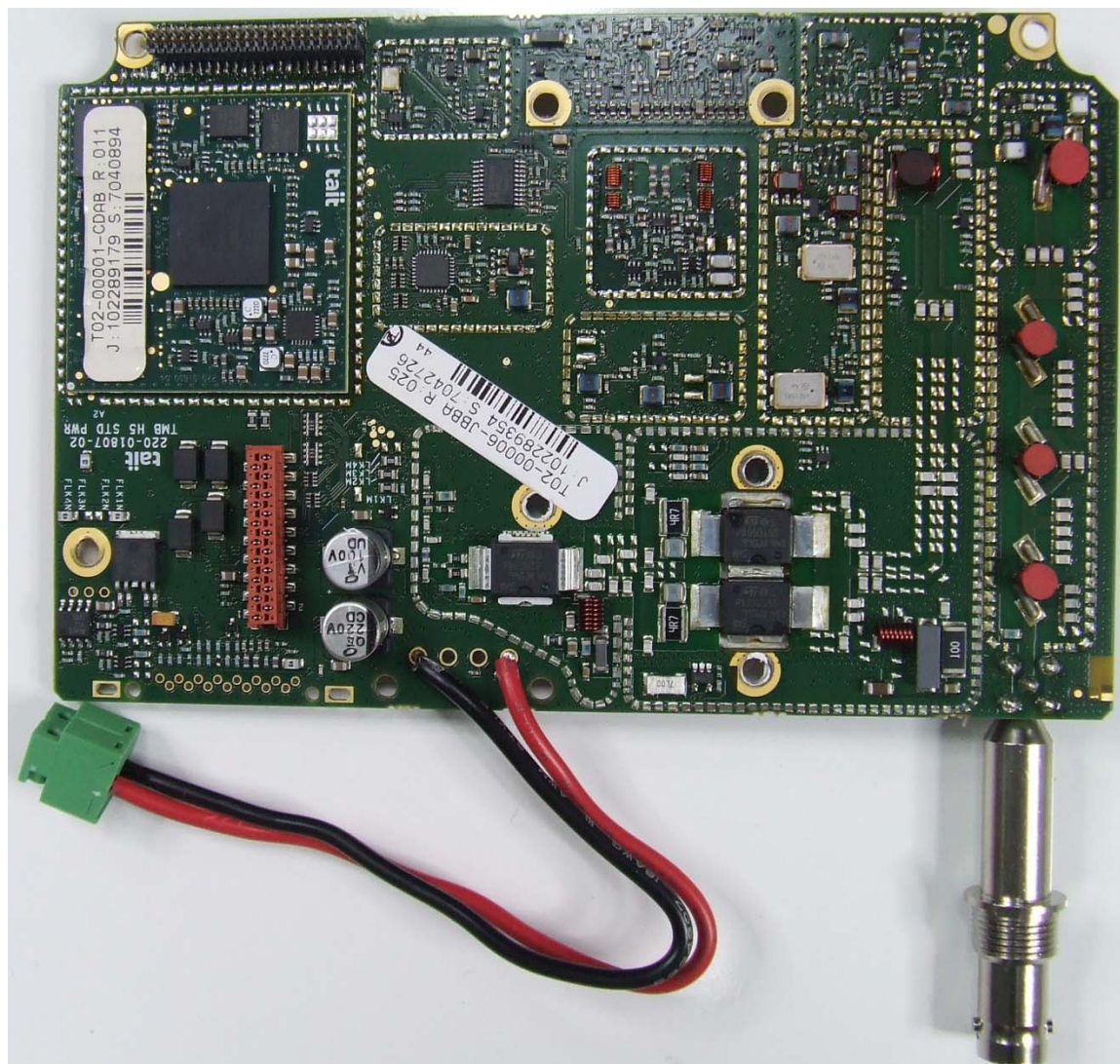
Photograph 05: RF PCB top without shields
