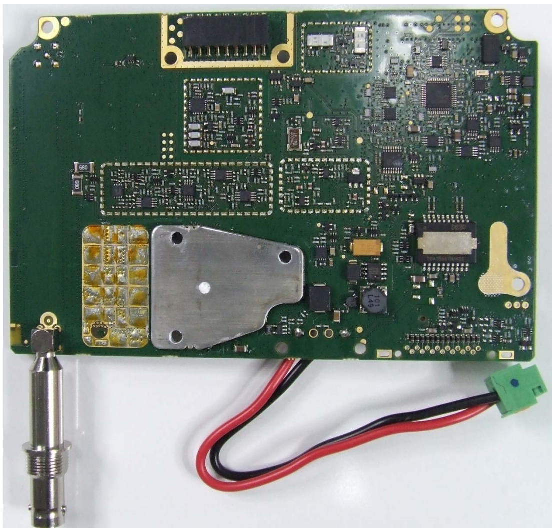
Photograph 07: RF PCB bottom without shields
