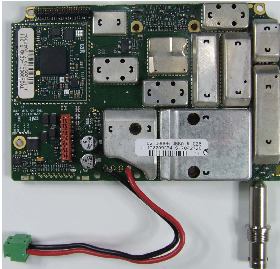
Photograph 04: RF PCB top with shields
