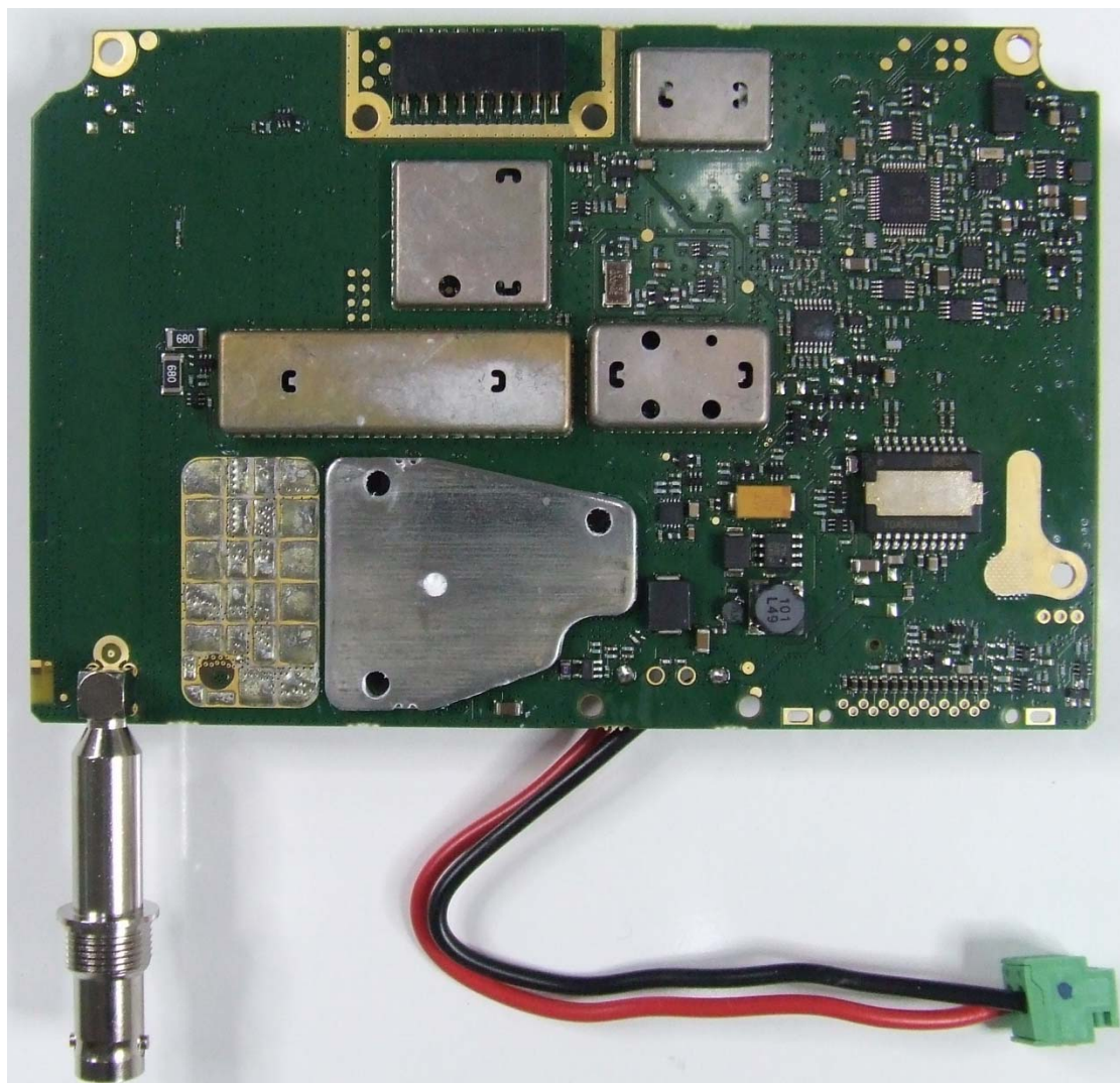
Photograph 06: RF PCB bottom with shields
