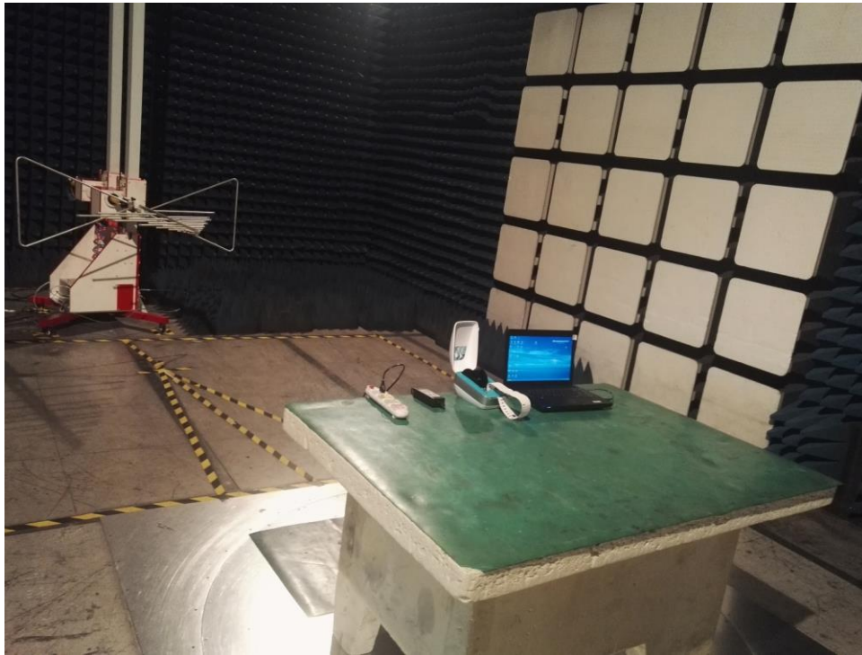
Photograph 1: Setup for Radiated Emissions
