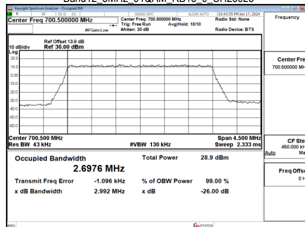
Band12_3MHz_64QAM_RB15_0_CH23095
