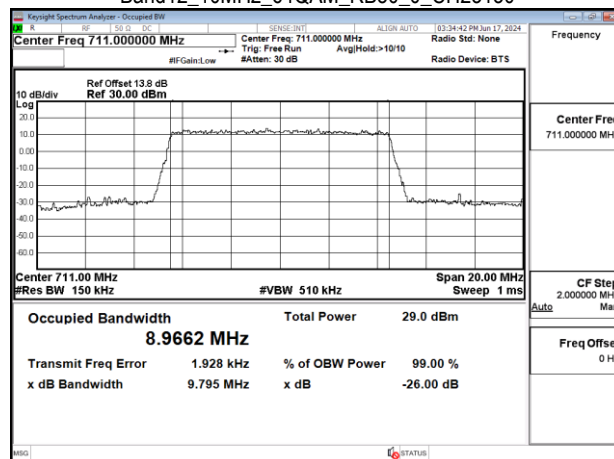
Band12_10MHz_64QAM_RB50_0_CH23130
