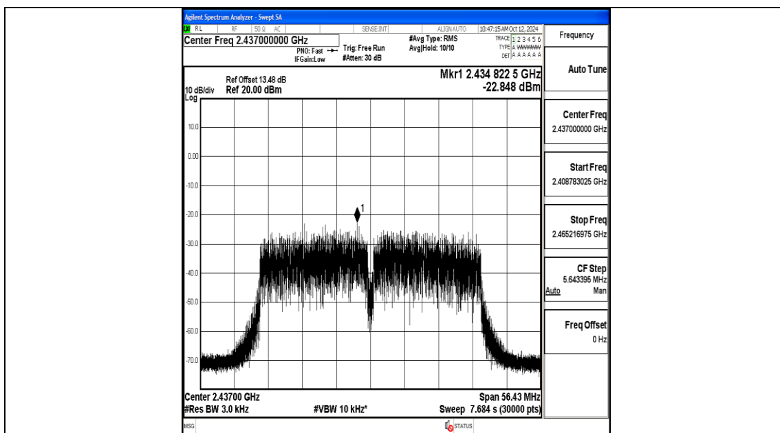
11N40MIMO-Ant1-2437-PASS
