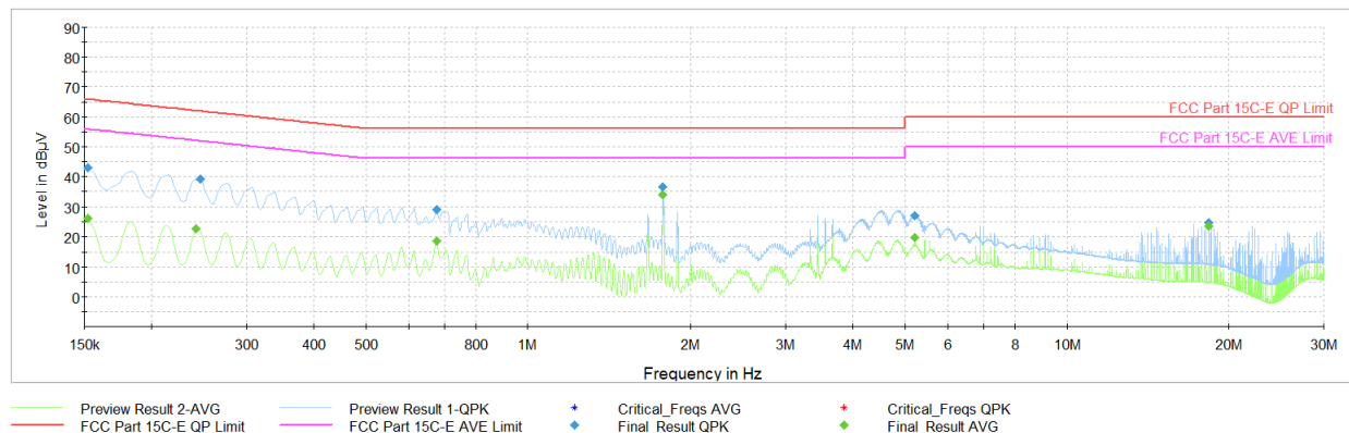
Plot 7-44. AC Line-Conducted Test Plot (N, GFSK ePA – Ch.39, with AC/DC Adapter + Magnetic Charger)
