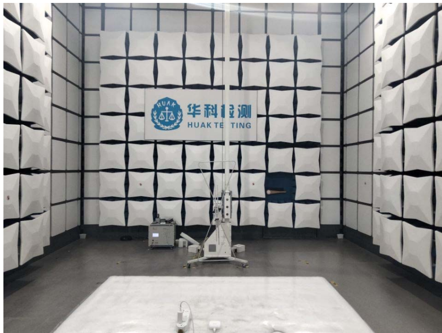
LP-30 pro Radiated Emissions
