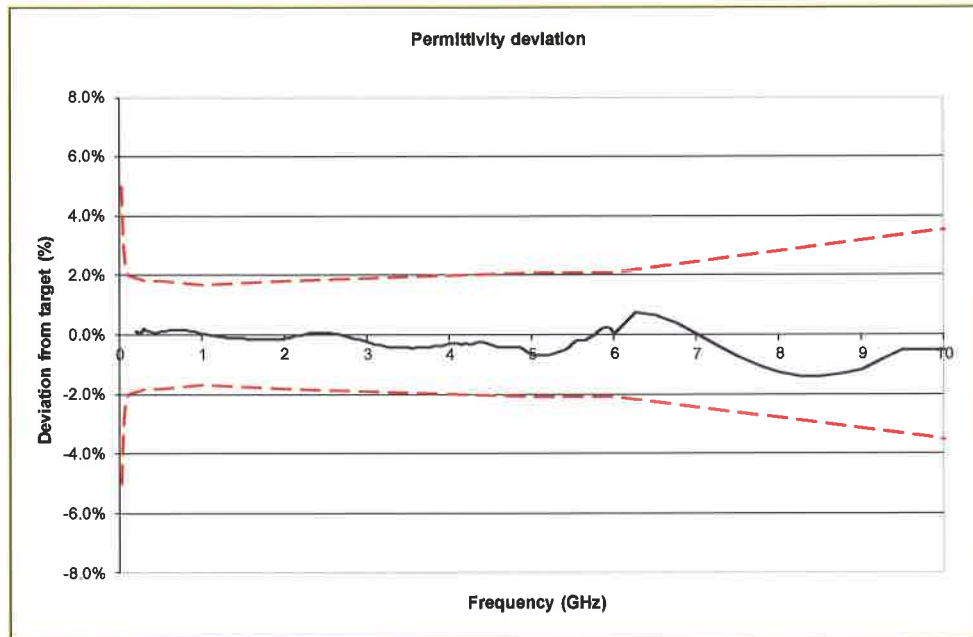
Fig. C.1.1 Methanol permittivity deviation from target, 200 MHz – 10 GHz
