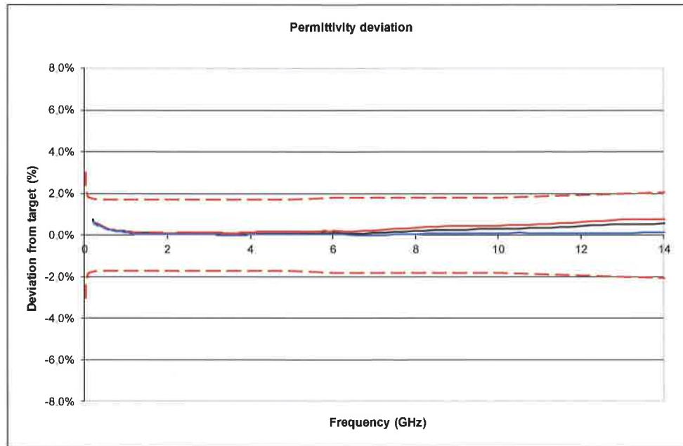
Fig. 5.1 0.05 mol/L solution permittivity deviation from target, 200 MHz – 14 GHz
