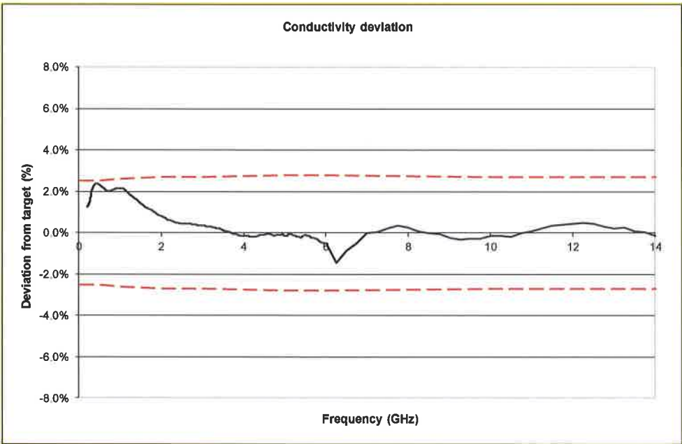
Fig. C.3.2 0.05 mol/L solution conductivity deviation from target, 200 MHz – 14 GHz
