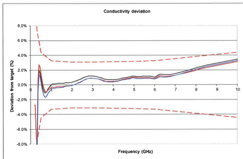
Fig. 3.2 Methanol conductivity deviation from target, 200 MHz – 10 GHz
