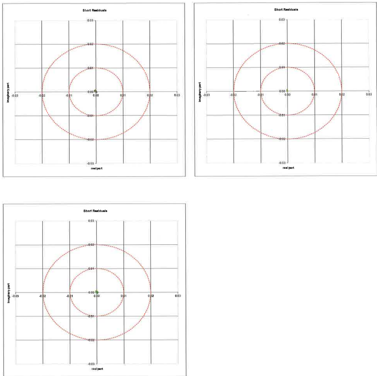
Fig. 2.2a-c Complex representation of the residuals of the shorts, 200 MHz - 14 GHz, after calibrations a)-b) in the top and c) in the bottom
