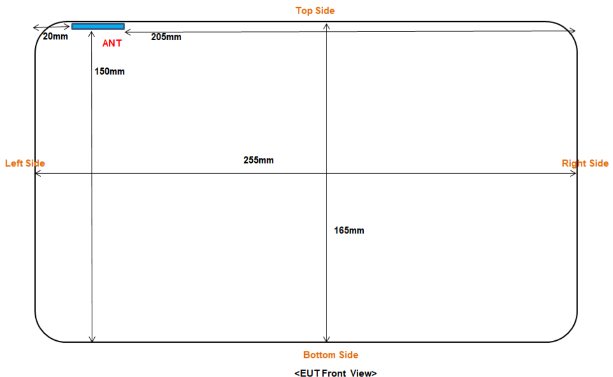
Fig 7.1 Block Diagram for EUT Antenna Position EUT Size: Long*Width*Height=255mm*165mm*23mm
