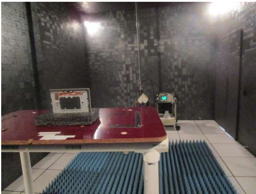
RADIATED EMISSIONS TEST SETUP 18 TO 25 GHZ
