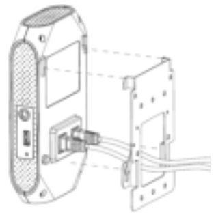
Figure 9 Attaching OAW-AP1301H to wall mounting plate
