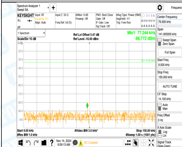
Band5-4233-3-0.009~0.15MHz-PASS
