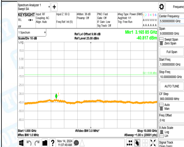
Band5-4132-4-1000~10000MHz-PASS
