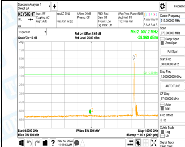
Band5-4132-5-30~1000MHz-PASS
