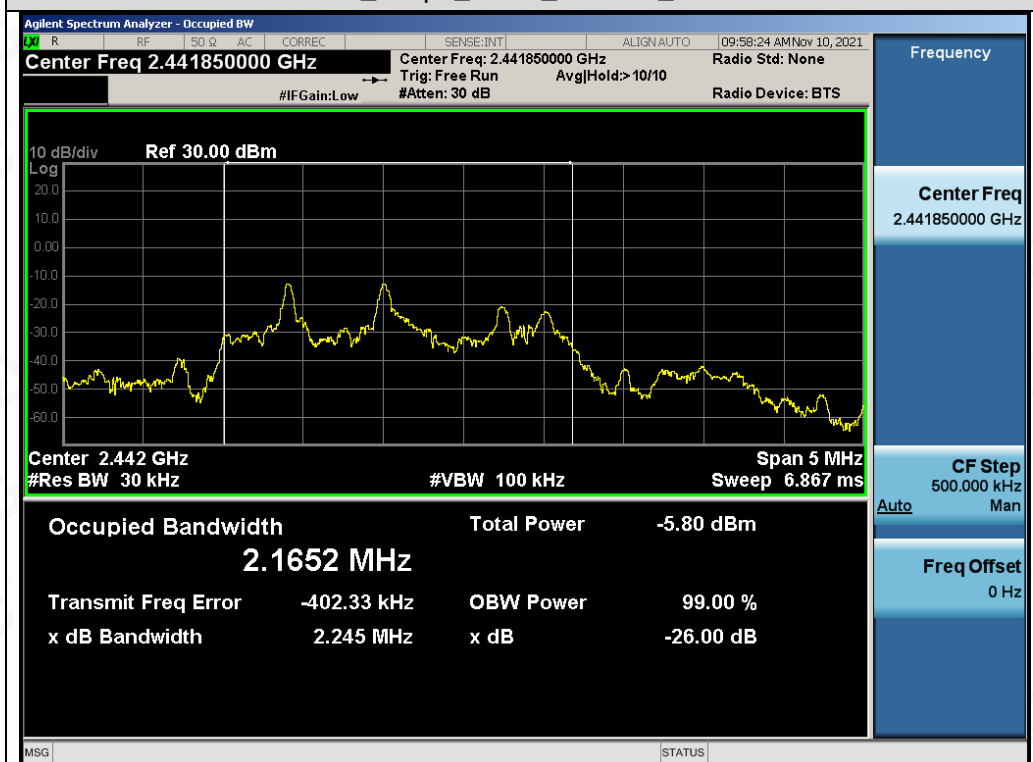
Test_Graph_ANT1_2441.85_OBW
