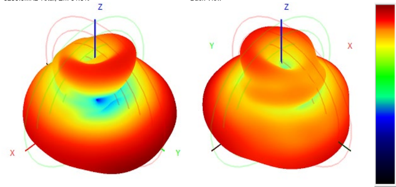
5250.0MHz Total, Eff: 61.3%
