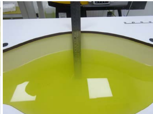
Body 5GHz_16.1cm
