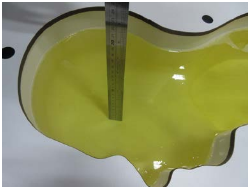
Head 5GHz_15.5cm
