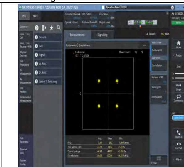
1-25--15-40-M-6-CP-QPSK-Outer_Full-216@0-Ant1-see graph-PASS
