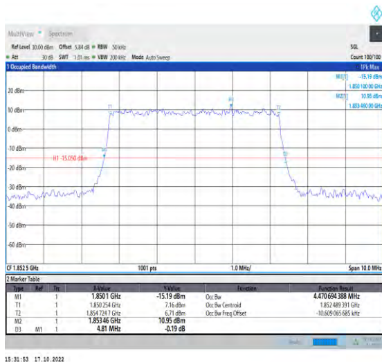
1-N25-PC3-15-5-L-4-DFT-64QAM-Outer_Full-25@0- -Ant1-4.471-4.810-≤5-PASS
