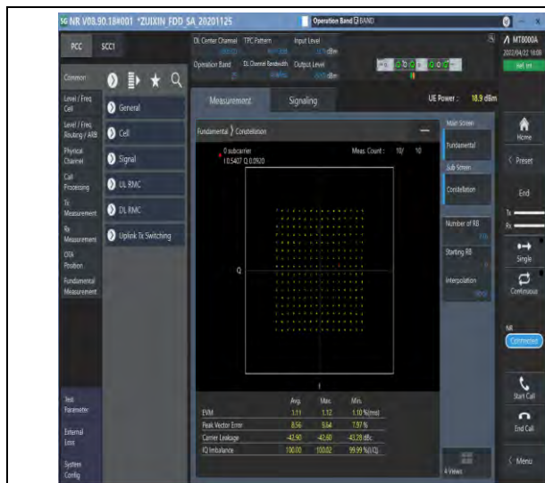
1-25--15-40-M-5-DFT-256QAM-Outer_Full-216@0-Ant1-see graph-PASS
