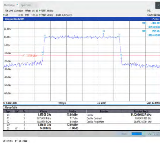
1-N25-PC3-15-15-M-6-CP-QPSK-Outer_Full-79@0-Ant1-14.121-14.880-≤15-PASS
