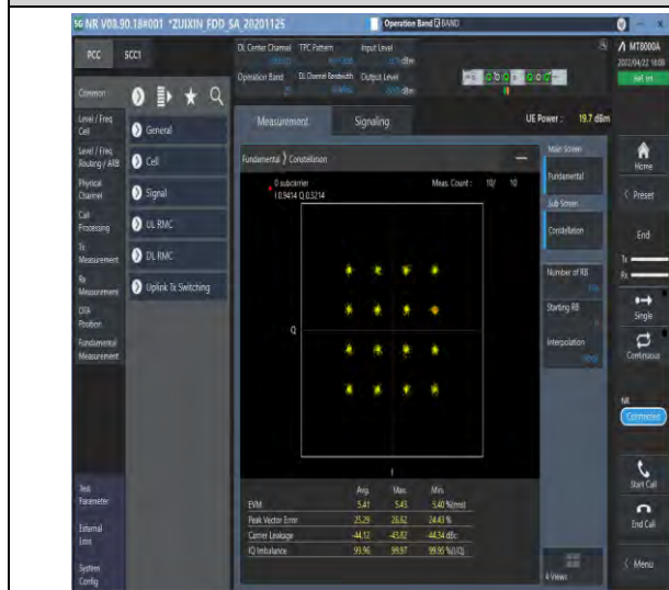
1-25--15-40-M-7-CP-16QAM-Outer_Full-216@0-Ant1-see graph-PASS
