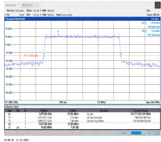
1-N25-PC3-15-15-M-7-CP-16QAM-Outer_Full-79@0-Ant1-14.112-14.850-≤15-PASS
