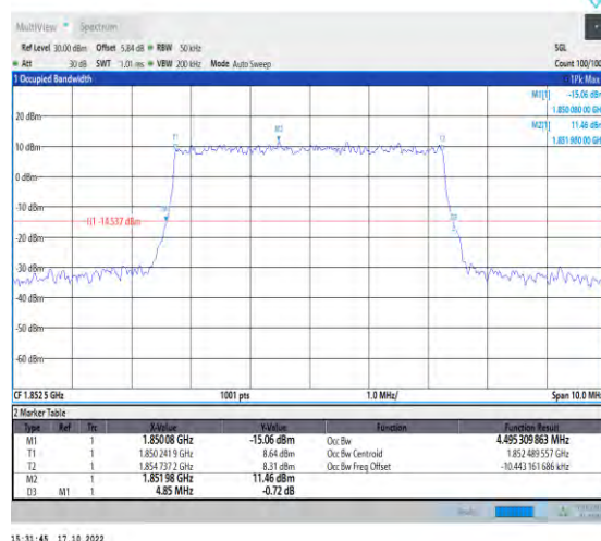
1-N25-PC3-15-5-L-3-DFT-16QAM-Outer_Full-25@0- Ant1-4.495-4.850-≤5-PASS
