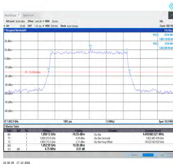
1-N25-PC3-15-5-L-5-DFT-256QAM-Outer_Full-25@0- -Ant1-4.46-4.750-≤5-PASS
