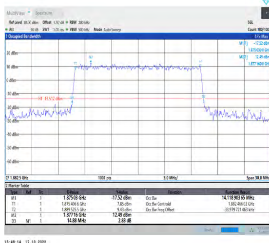
1-N25-PC3-15-15-M-8-CP-64QAM-Outer_Full-79@0-Ant1-14.119-14.880-≤15-PASS
