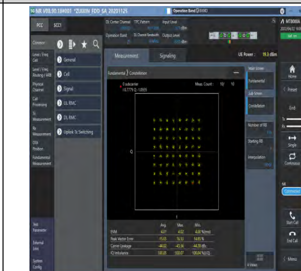
1-25--15-40-M-8-CP-64QAM-Outer_Full-216@0-Ant1-see graph-PASS
