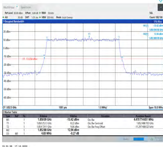
1-N25-PC3-15-5-L-1-DFT-QPSK-Outer_Full-25@0- Ant1-4.471-4.830-≤5-PASS
