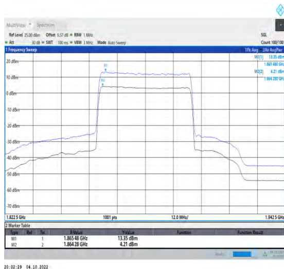
1-N25-PC3-15-40-M-1-DFT-256QAM-Outer_Full-216 @0-Ant1-9.14-100%-0.00-9.14-PASS-≤13
