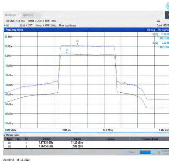
1-N25-PC3-15-40-M-2-CP-256QAM-Outer_Full-216 @0-Ant1-9.27-100%-0.00-9.27-PASS-≤13
