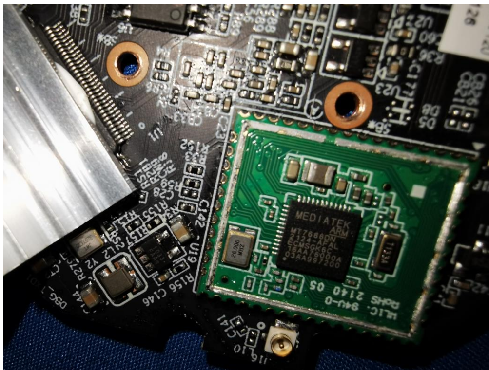
ANTENNA PORT
