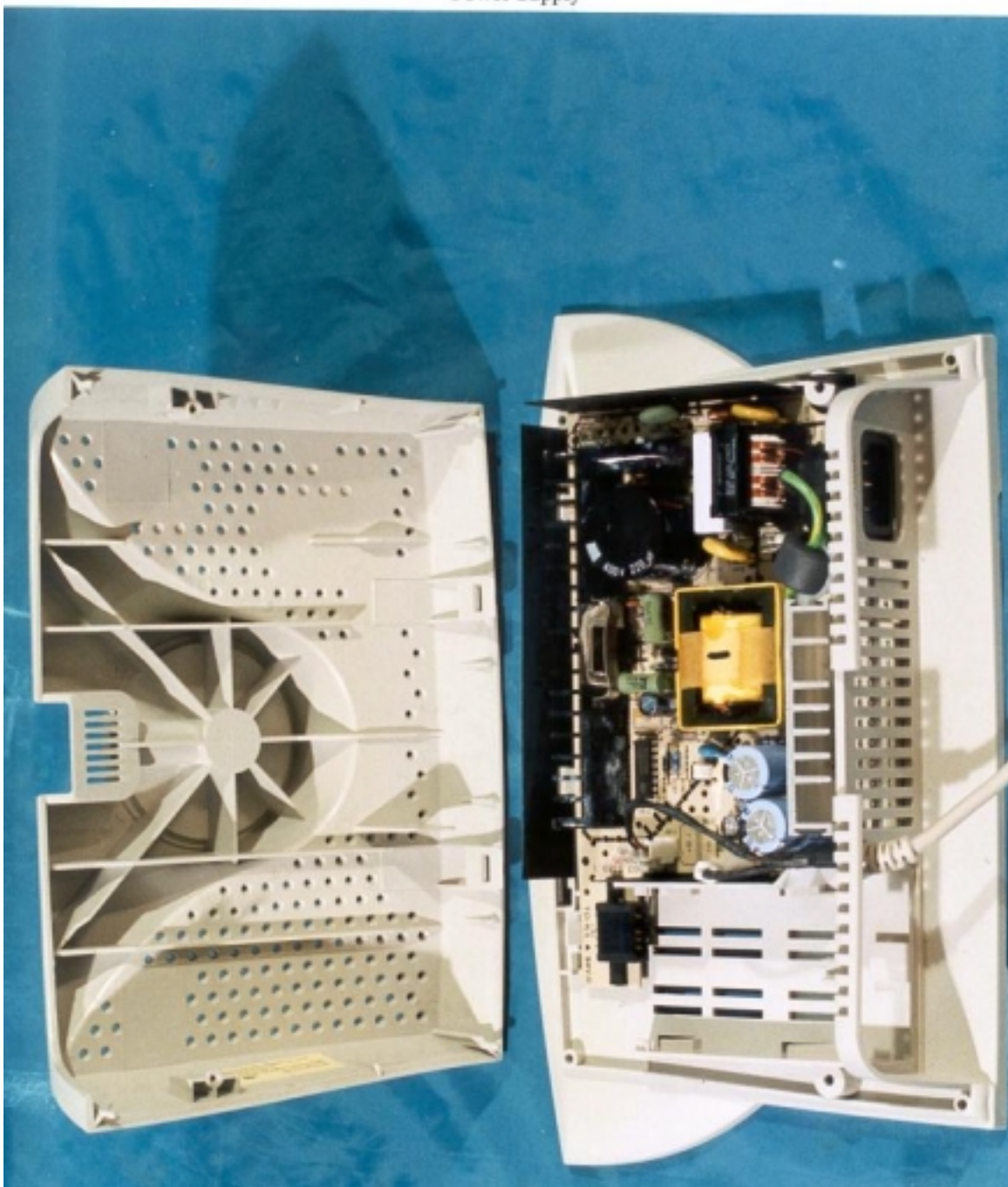
Power Supply
