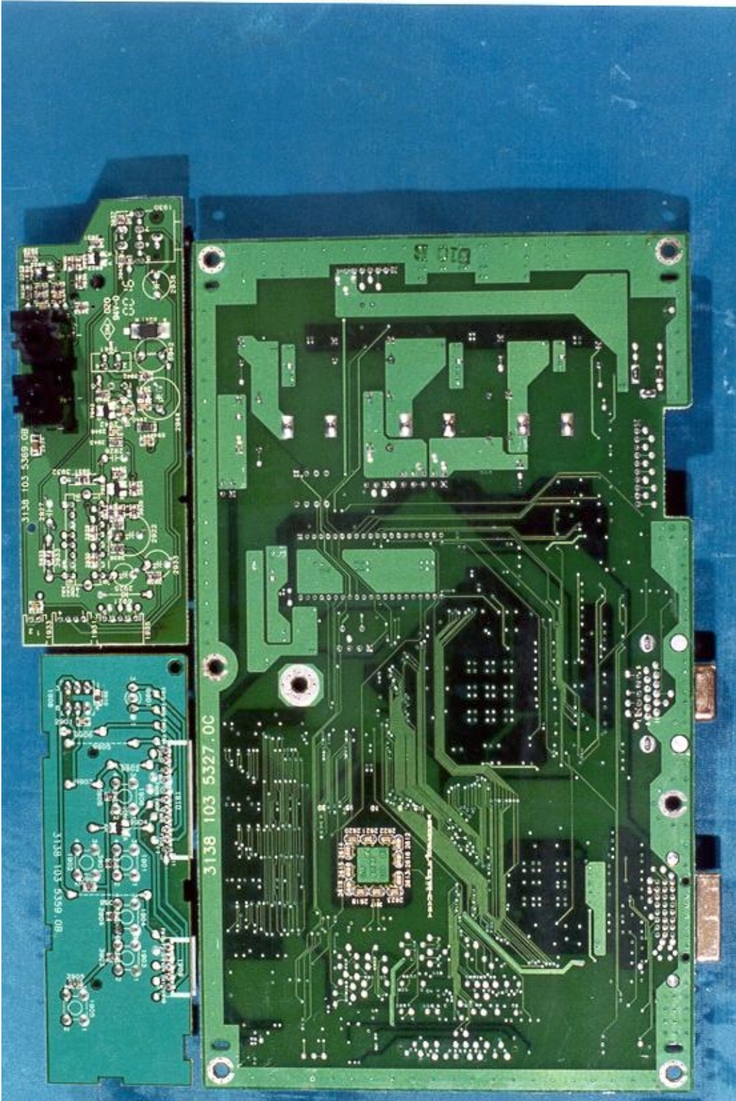
PCB Layout
