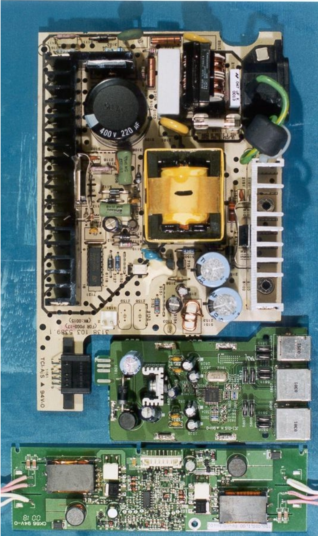
PCB Layout
