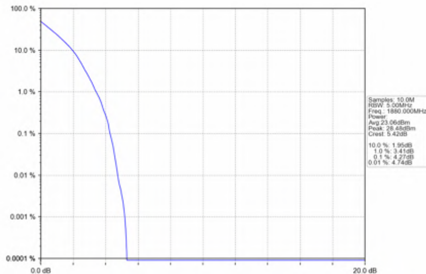
n2_15kHz_SISO_NTNV_5MHz_DFT-s-OFDM PI/2 BPSK_1880MHz_Outer_Full
