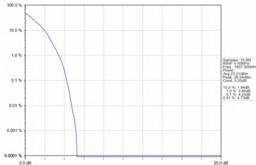
n2_15kHz_SISO_NTNV_5MHz_DFT-s-OFDM PI/2 BPSK_1907.5MHz_Outer_Full
