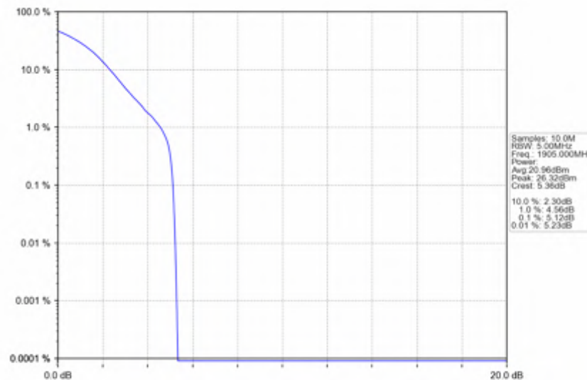
n2_30kHz_SISO_NTNV_10MHz_DFT-s-OFDM PI/2 BPSK_1905MHz_Outer_Full
