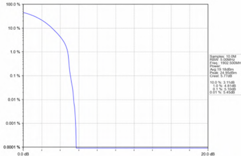
n2_30kHz_SISO_NTNV_15MHz_DFT-s-OFDM PI/2 BPSK_1902.5MHz_Outer_Full
