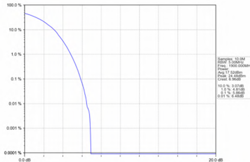
n2_30kHz_SISO_NTNV_20MHz_DFT-s-OFDM PI/2 BPSK_1900MHz_Outer_Full
