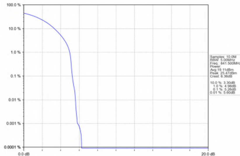
n5_30kHz_SISO_NTNV_15MHz_DFT-s-OFDM PI/2 BPSK_841.5MHz_Outer_Full
