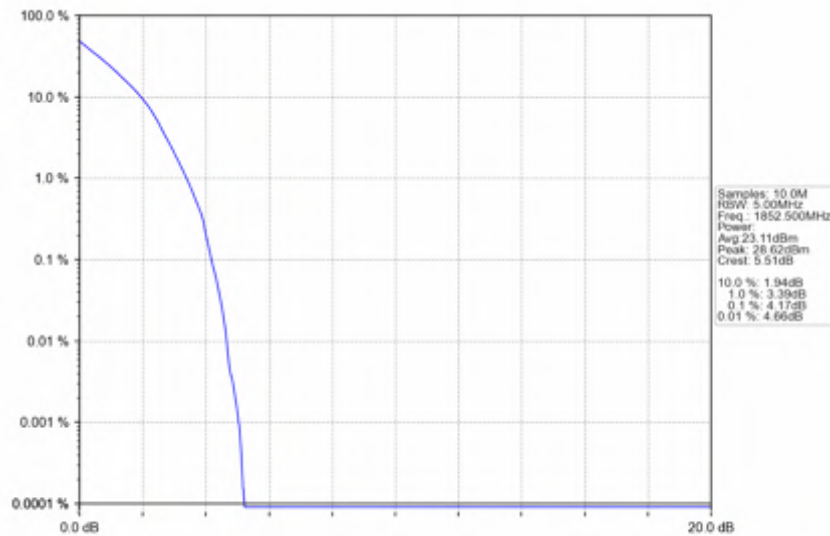
n2_15kHz_SISO_NTNV_5MHz_DFT-s-OFDM PI/2 BPSK_1852.5MHz_Outer_Full
