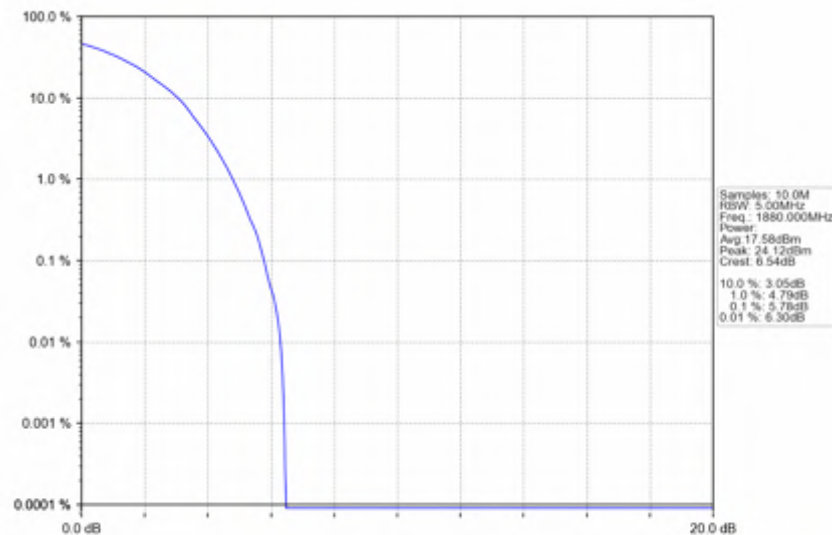
n2_30kHz_SISO_NTNV_20MHz_DFT-s-OFDM PI/2 BPSK_1880MHz_Outer_Full
