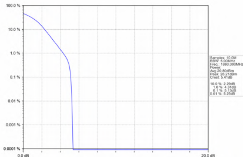
n2_30kHz_SISO_NTNV_10MHz_DFT-s-OFDM PI/2 BPSK_1880MHz_Outer_Full
