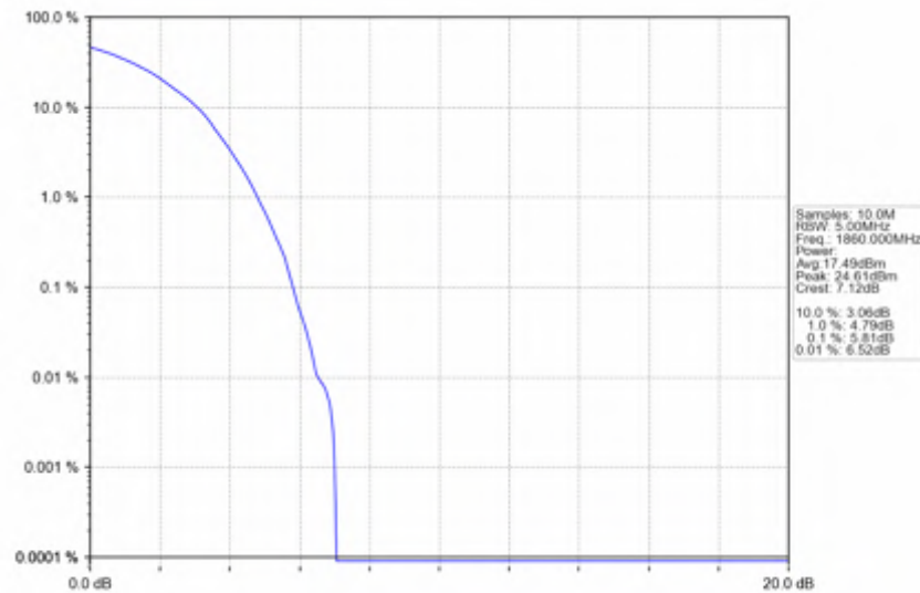
n2_30kHz_SISO_NTNV_20MHz_DFT-s-OFDM PI/2 BPSK_1860MHz_Outer_Full
