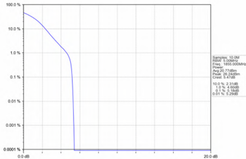
n2_30kHz_SISO_NTNV_10MHz_DFT-s-OFDM PI/2 BPSK_1855MHz_Outer_Full
