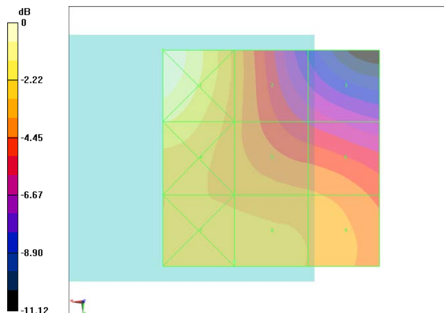
Fig B.15 HAC RF H-Field GSM 1900 Low
