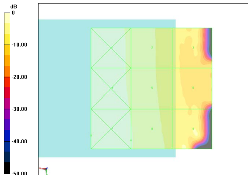
Fig B.17 HAC RF H-Field WCDMA 850 Middle
