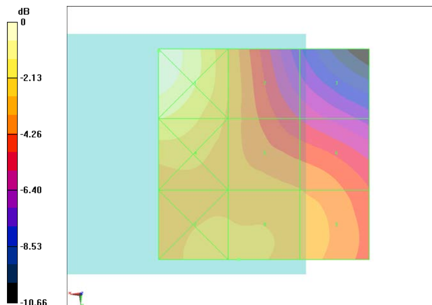
Fig B.13 HAC RF H-Field GSM 1900 High
