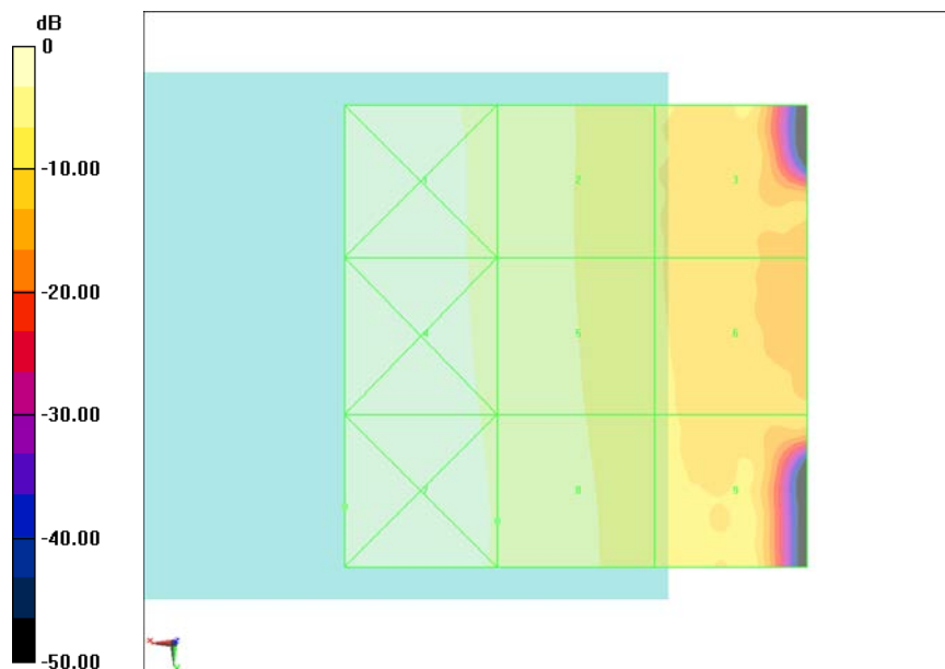
Fig B.10 HAC RF H-Field GSM 850 High
