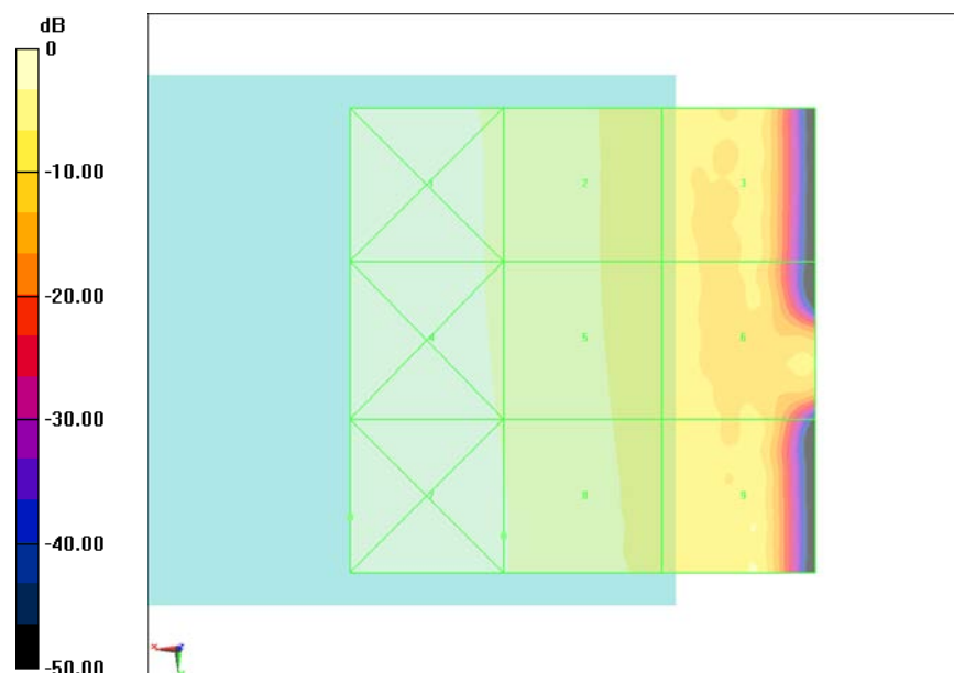
Fig B.18 HAC RF H-Field WCDMA 850 Low
