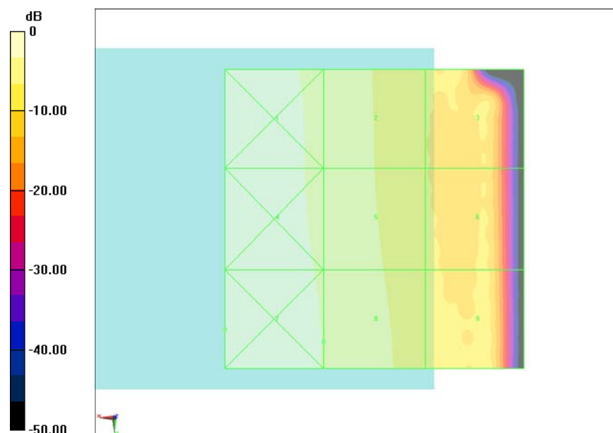
Fig B.11 HAC RF H-Field GSM 850 Middle
