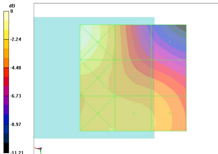
Fig B.14 HAC RF H-Field GSM 1900 Middle
