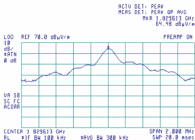
Plot 7.4.9 Radiated emission measurements at the 2 nd harmonic
