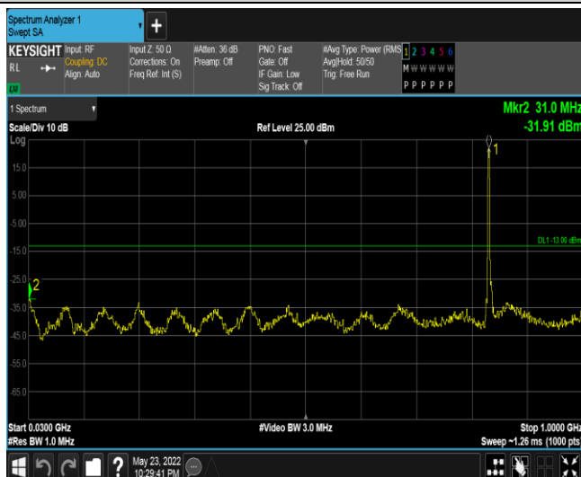
Band5-5MHz-16QAM-20525-1RB#0-Range2:30~1000MHz
