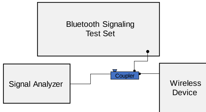
Power Measurement Setup
