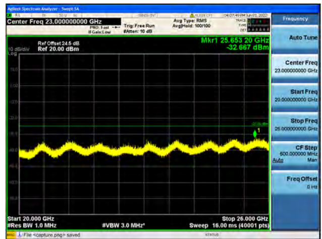
B7-20G-26G / 15MHz / High CH / 64QAM
