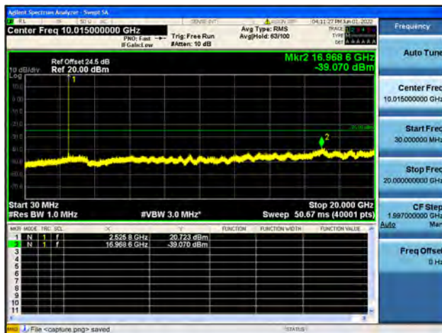
B7-30M-20G / 20MHz / Mid CH / 64QAM
