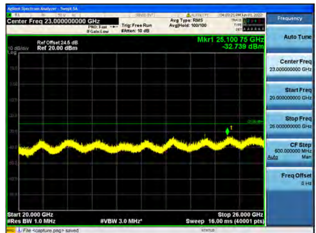
B7-20G-26G / 10MHz / High CH / 64QAM
