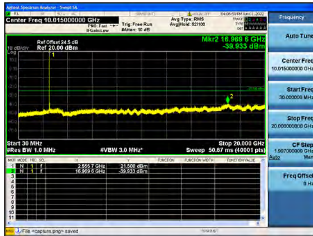
B7-30M-20G / 15MHz / High CH / 16QAM
