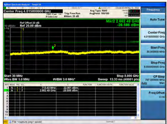
B12 / 3MHz / High CH / 64QAM
