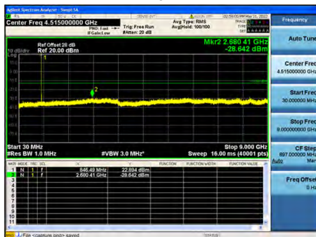
B5 / 3MHz / High CH / 16QAM
