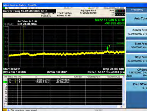
B7-30M-20G / 15MHz / Mid CH / 64QAM
