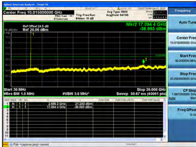
B7-30M-20G / 5MHz / High CH / 64QAM
