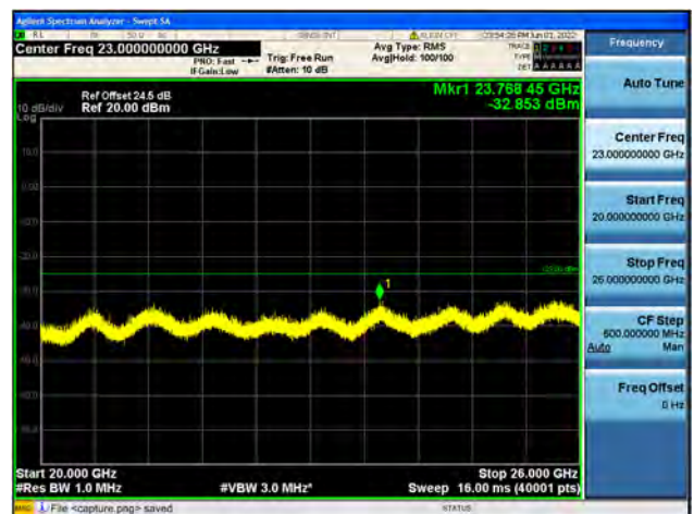
B7-20G-26G / 5MHz / Low CH / 64QAM
