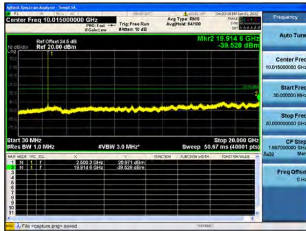
B7-30M-20G / 15MHz / Low CH / 16QAM
