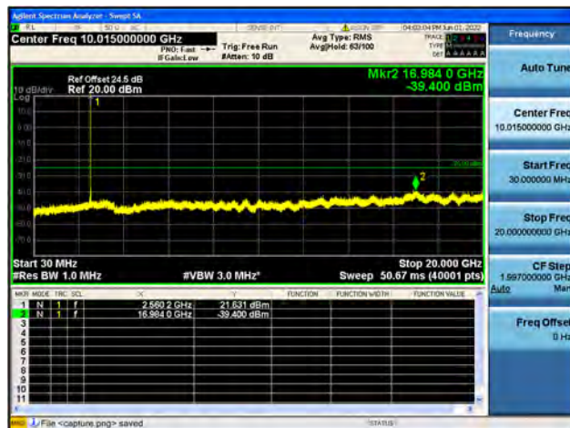
B7-30M-20G / 10MHz / High CH / 64QAM
