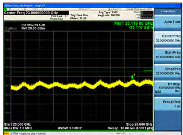
B7-20G-26G / 15MHz / High CH / 64QAM
