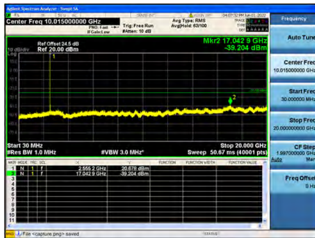
B7-30M-20G / 15MHz / High CH / 64QAM
