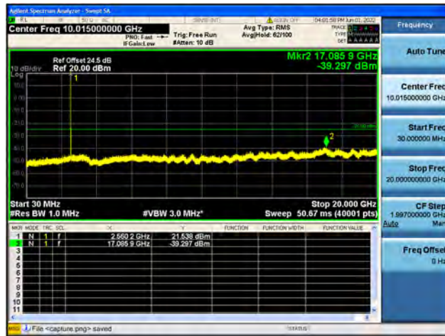
B7-30M-20G / 10MHz / High CH / 16QAM
