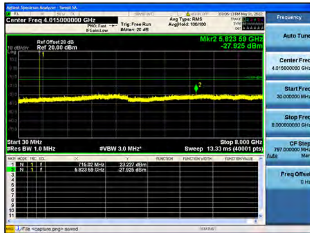
B12 / 1.4MHz / High CH / 64QAM
