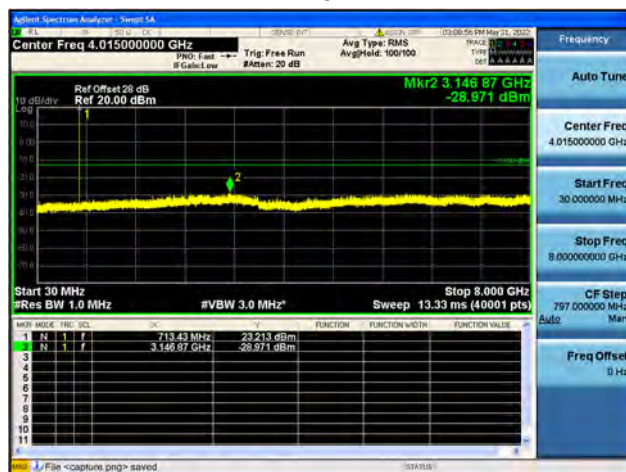
B12 / 3MHz / High CH / 16QAM
