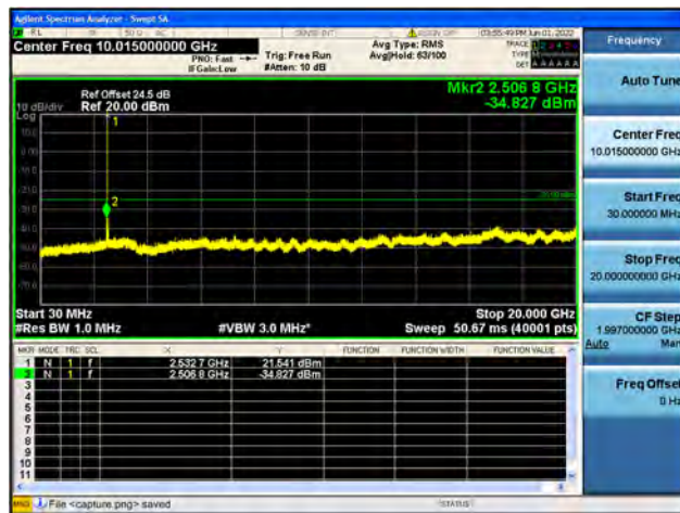
B7-30M-20G / 5MHz / Mid CH / 64QAM
