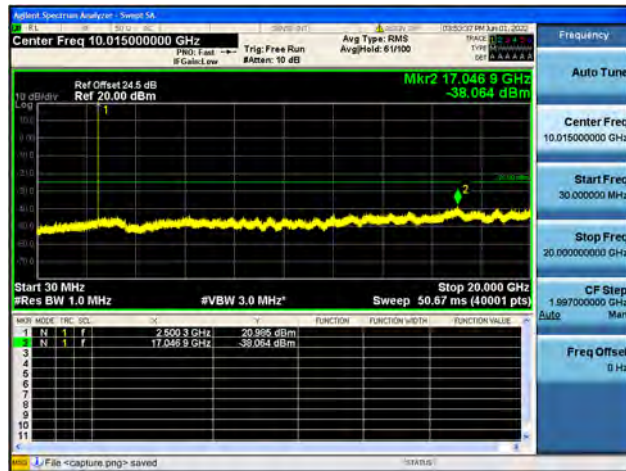
B7-30M-20G / 5MHz / Low CH / 16QAM
