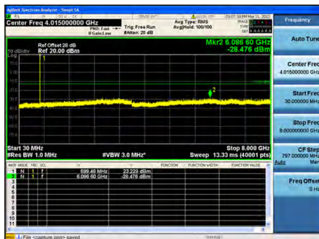
B12 / 3MHz / Low CH / 16QAM
