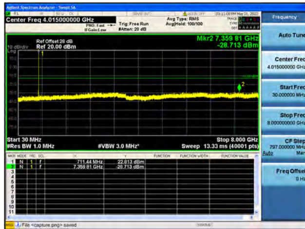
B12 / 5MHz / High CH / 64QAM
