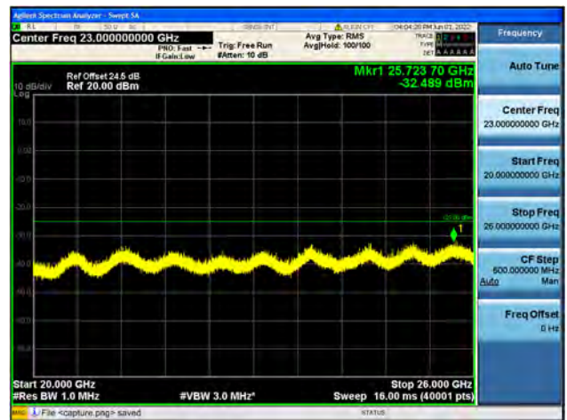
B7-20G-26G / 15MHz / Low CH / 64QAM
