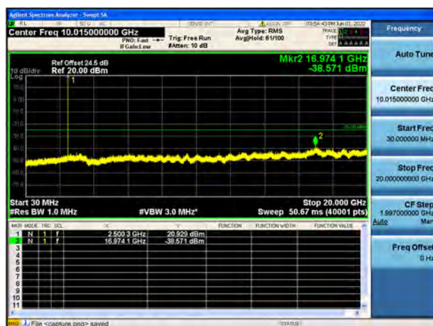
B7-30M-20G / 5MHz / Low CH / 64QAM
