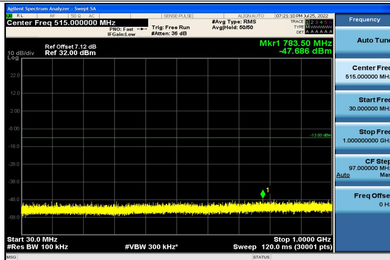
Band4-1.4MHz-QPSK-20175-1RB#0-30~1000MHz
