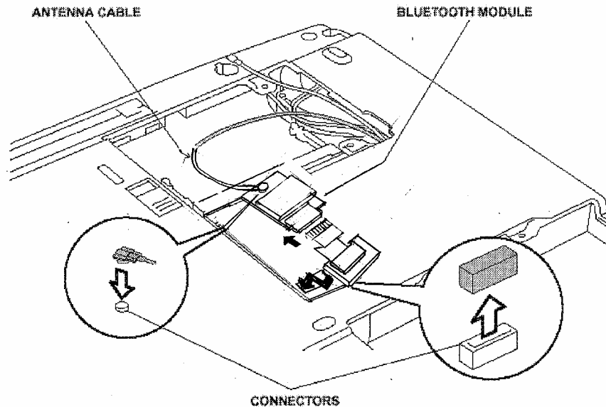
Installing the Bluetooth module
