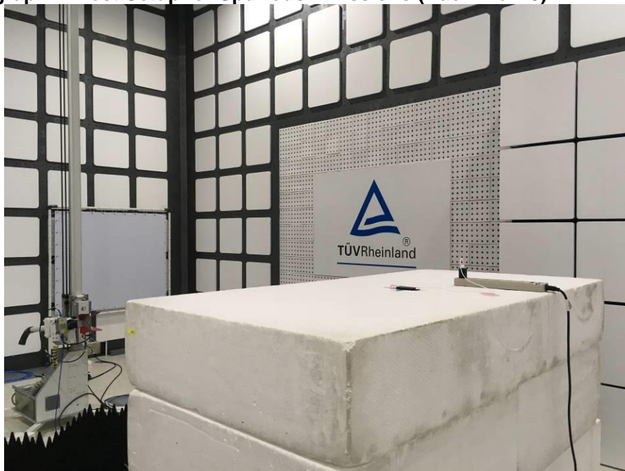
Photograph 4: Test Setup for Spurious Emissions (Back View 3)
