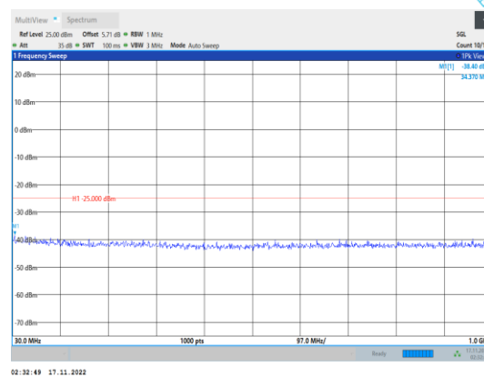
Band38-10MHz-64QAM-38200-1RB#0-Range1:30~1000MHz
