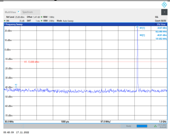
Band26-1.4MHz-64QAM-26783-1RB#0- Range1:30~1000MHz
