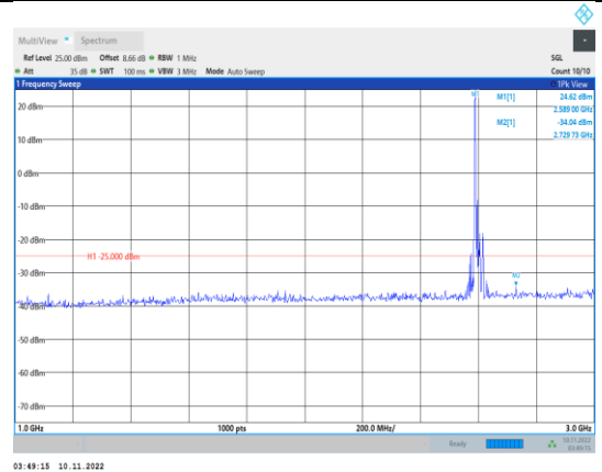
Band38-15MHz-QPSK-38000-1RB#0- Range2:1000~3000MHz
