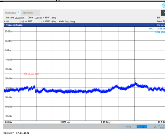
Band38-10MHz-64QAM-37800-1RB#0- Range3:3000~26500MHz
