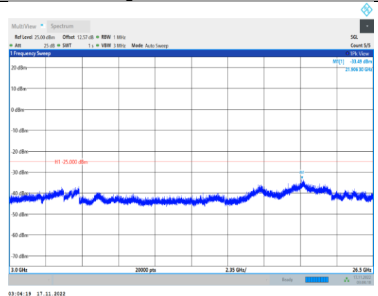
Band38-5MHz-64QAM-38000-1RB#0- Range3:3000~26500MHz
