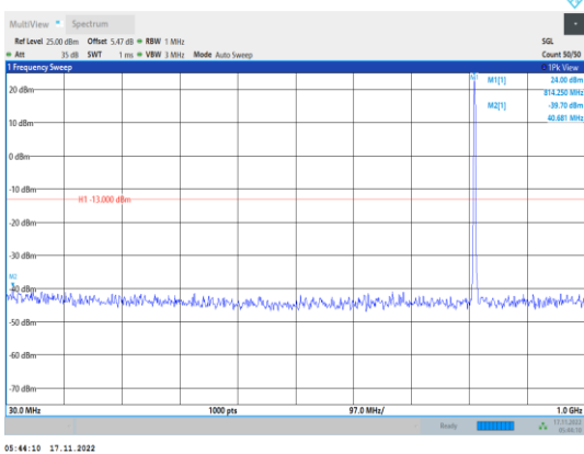
Band26-1.4MHz-64QAM-26697-1RB#0- Range1:30~1000MHz
