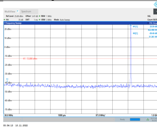
Band26-1.4MHz-16QAM-26783-1RB#0- Range1:30~1000MHz
