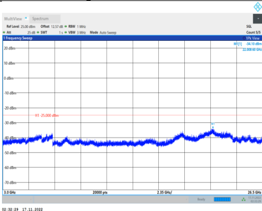
Band38-10MHz-64QAM-38000-1RB#0-Range3:3000~26500MHz
