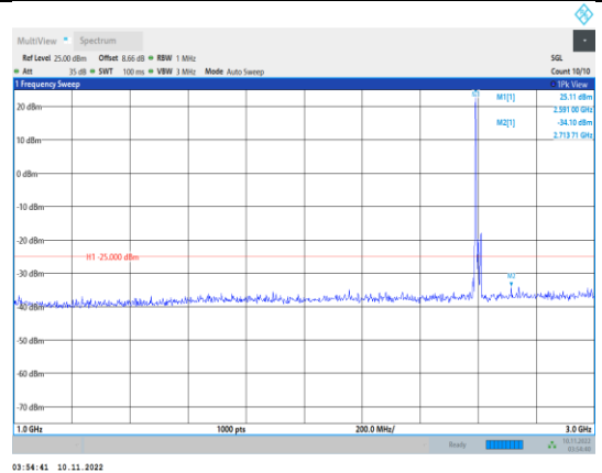
Band38-10MHz-16QAM-38000-1RB#0- Range2:1000~3000MHz
