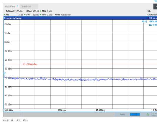
Band38-10MHz-64QAM-37800-1RB#0- Range1:30~1000MHz
