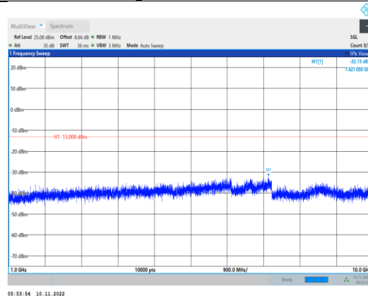
Band26-1.4MHz-QPSK-26783-1RB#0- Range2:1000~10000MHz
