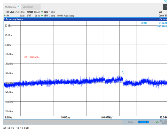
Band26-1.4MHz-16QAM-26740-1RB#0- Range2:1000~10000MHz
