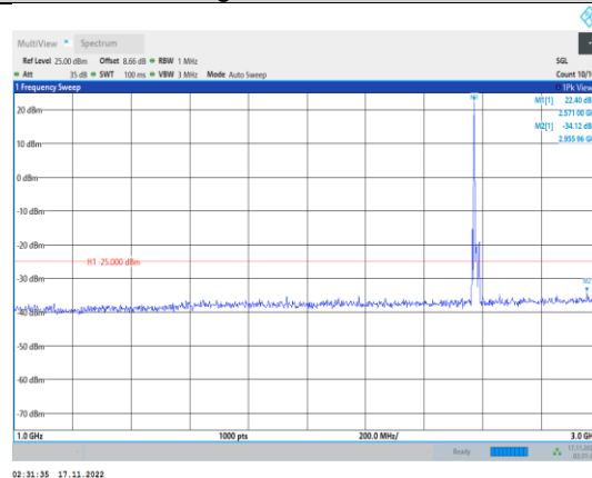
Band38-10MHz-64QAM-37800-1RB#0- Range2:1000~3000MHz
