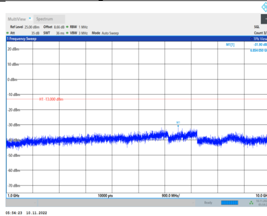
Band26-1.4MHz-16QAM-26783-1RB#0- Range2:1000~10000MHz
