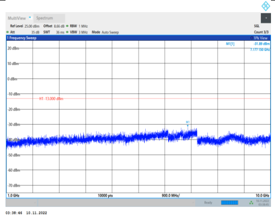
Band26-15MHz-QPSK-26915-1RB#0- Range2:1000~10000MHz
