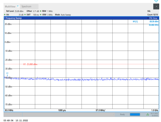
Band38-15MHz-QPSK-38000-1RB#0- Range1:30~1000MHz
