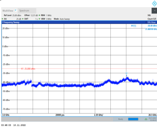
Band38-15MHz-QPSK-37825-1RB#0- Range3:3000~26500MHz
