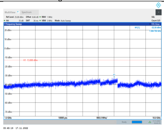
Band26-1.4MHz-64QAM-26783-1RB#0- Range2:1000~10000MHz
