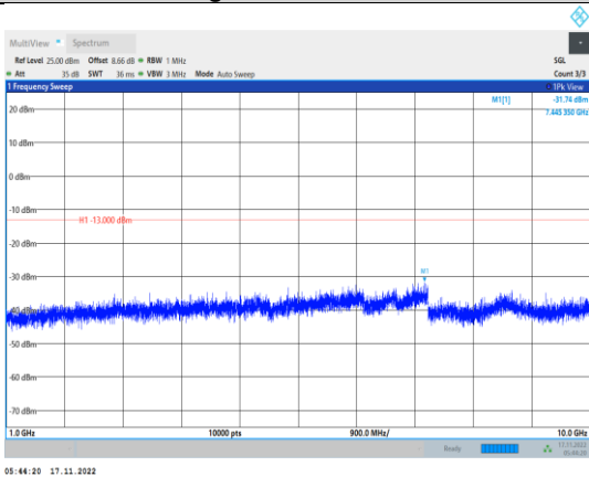
Band26-1.4MHz-64QAM-26697-1RB#0- Range2:1000~10000MHz
