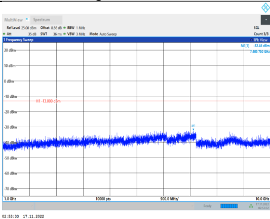
Band26-15MHz-64QAM-26865-1RB#0- Range2:1000~10000MHz
