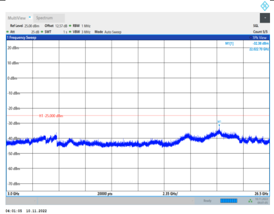
Band38-5MHz-16QAM-38225-1RB#0- Range3:3000~26500MHz
