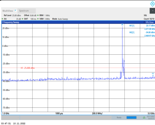
Band38-15MHz-QPSK-37825-1RB#0- Range2:1000~3000MHz
