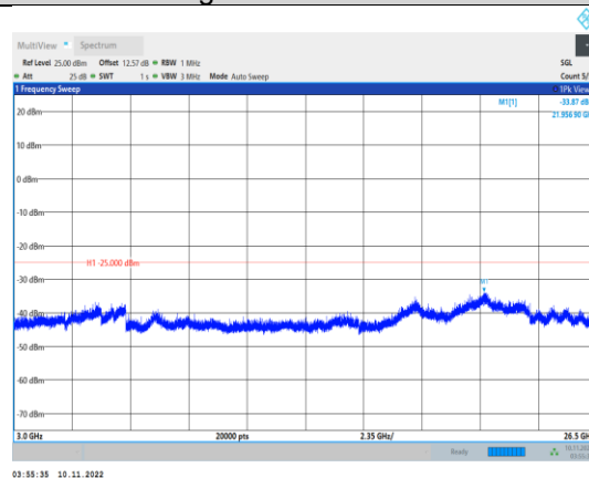
Band38-10MHz-QPSK-38200-1RB#0- Range3:3000~26500MHz
