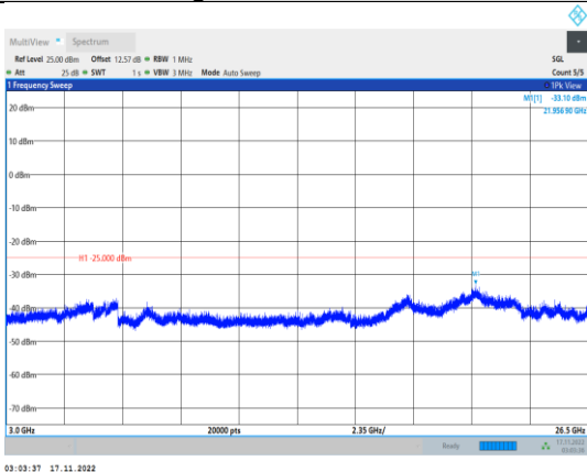
Band38-5MHz-64QAM-37775-1RB#0- Range3:3000~26500MHz
