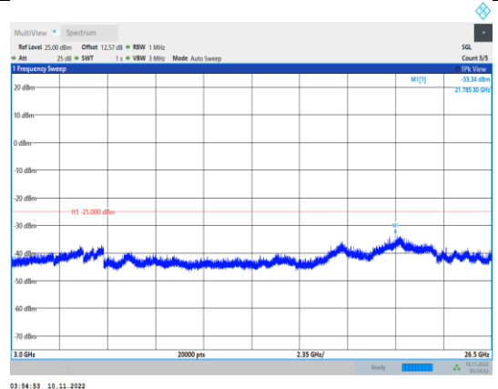
Band38-10MHz-16QAM-38000-1RB#0- Range3:3000~26500MHz
