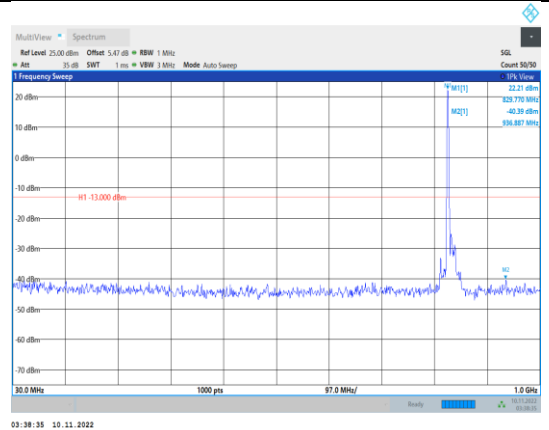
Band26-15MHz-QPSK-26915-1RB#0- Range1:30~1000MHz
