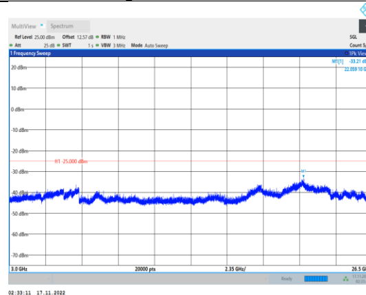
Band38-10MHz-64QAM-38200-1RB#0-Range3:3000~26500MHz
