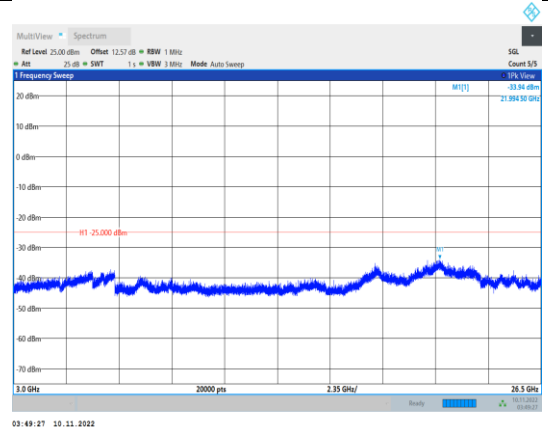
Band38-15MHz-QPSK-38000-1RB#0- Range3:3000~26500MHz
