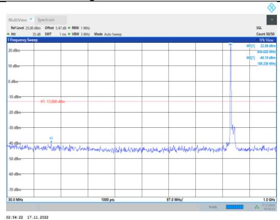
Band26-15MHz-64QAM-26965-1RB#0- Range1:30~1000MHz
