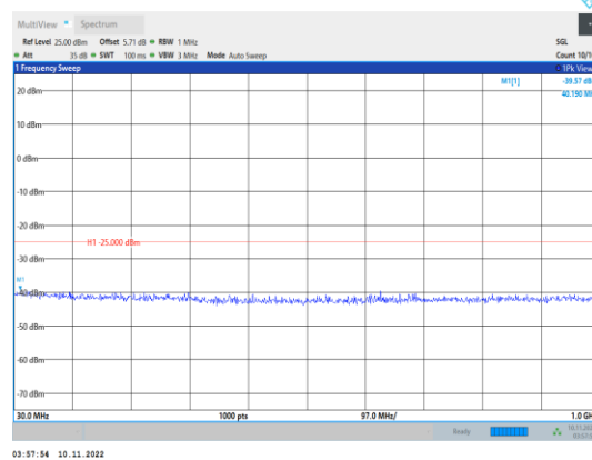
Band38-5MHz-16QAM-37775-1RB#0- Range1:30~1000MHz
