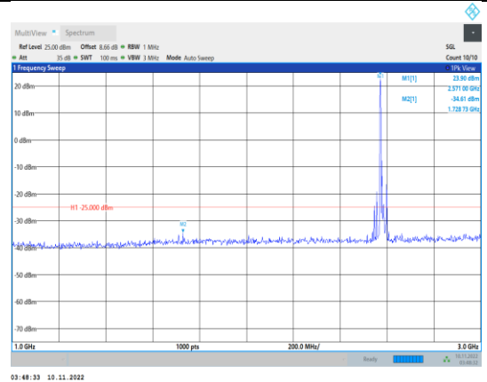
Band38-15MHz-16QAM-37825-1RB#0- Range2:1000~3000MHz
