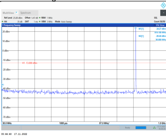
Band26-1.4MHz-64QAM-26740-1RB#0- Range1:30~1000MHz
