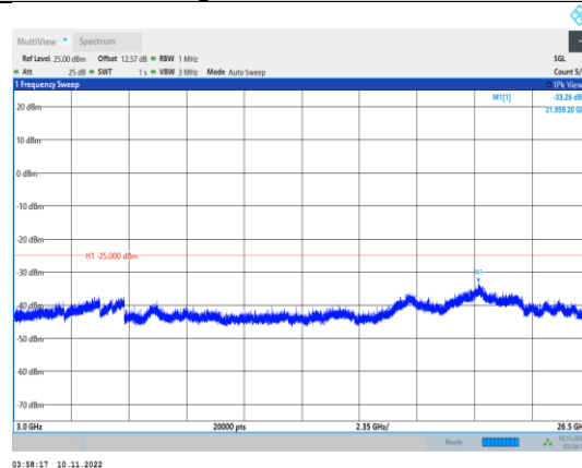
Band38-5MHz-16QAM-37775-1RB#0- Range3:3000~26500MHz
