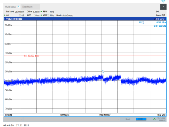
Band26-1.4MHz-64QAM-26740-1RB#0- Range2:1000~10000MHz
