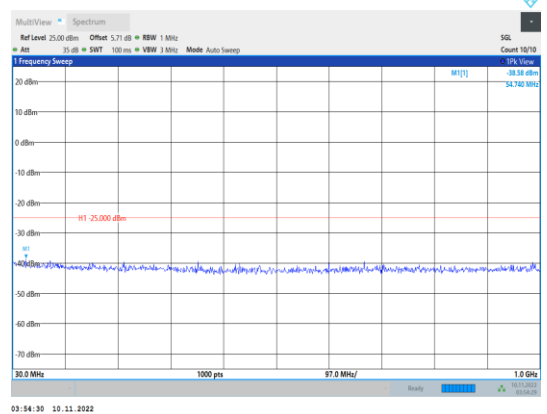
Band38-10MHz-16QAM-38000-1RB#0- Range1:30~1000MHz
