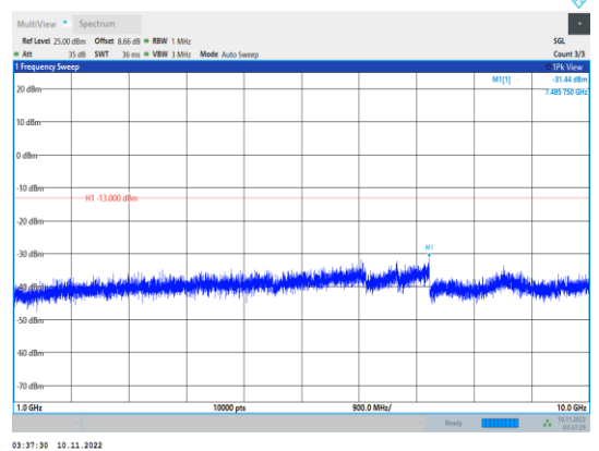
Band26-15MHz-QPSK-26865-1RB#0- Range2:1000~10000MHz
