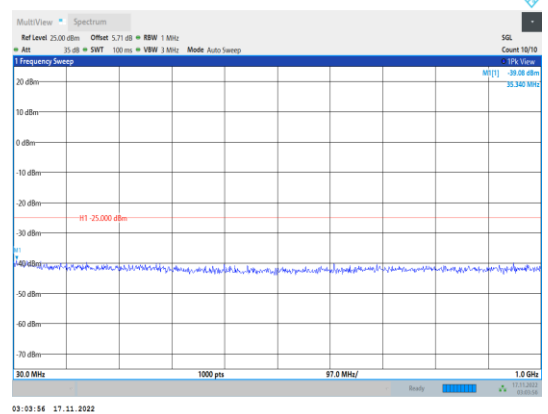
Band38-5MHz-64QAM-38000-1RB#0- Range1:30~1000MHz
