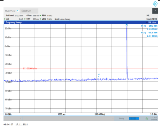
Band38-5MHz-64QAM-38000-1RB#0- Range2:1000~3000MHz
