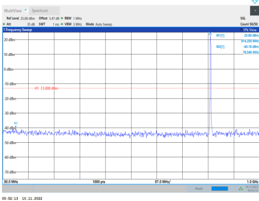
Band26-1.4MHz-16QAM-26697-1RB#0- Range1:30~1000MHz
