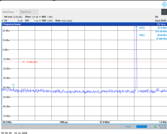
Band26-1.4MHz-QPSK-26740-1RB#0- Range1:30~1000MHz
