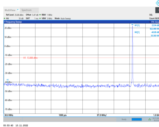
Band26-1.4MHz-QPSK-26783-1RB#0- Range1:30~1000MHz
