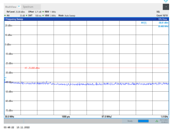
Band38-15MHz-16QAM-37825-1RB#0- Range1:30~1000MHz
