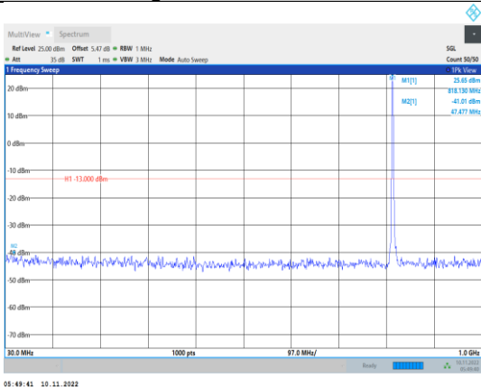
Band26-3MHz-16QAM-26740-1RB#0- Range1:30~1000MHz
