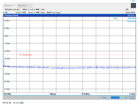
Band38-5MHz-16QAM-38225-1RB#0- Range1:30~1000MHz
