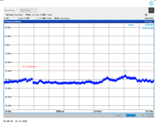
Band38-15MHz-16QAM-37825-1RB#0- Range3:3000~26500MHz
