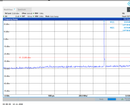
Band38-5MHz-16QAM-37775-1RB#0- Range2:1000~3000MHz
