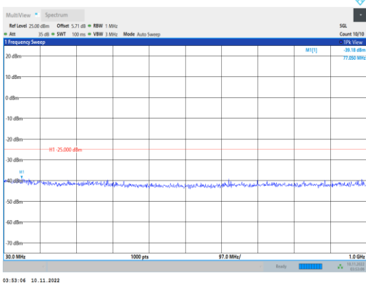
Band38-10MHz-16QAM-37800-1RB#0- Range1:30~1000MHz
