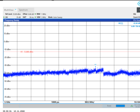
Band26-3MHz-16QAM-26775-1RB#0- Range2:1000~10000MHz
