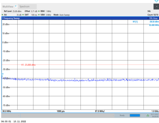
Band38-5MHz-QPSK-38225-1RB#0- Range1:30~1000MHz
