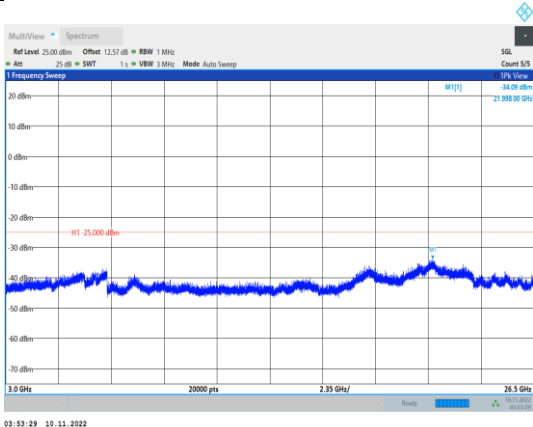
Band38-10MHz-16QAM-37800-1RB#0- Range3:3000~26500MHz
