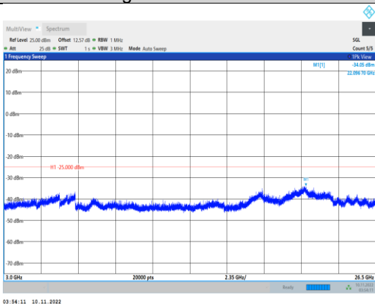
Band38-10MHz-QPSK-38000-1RB#0- Range3:3000~26500MHz
