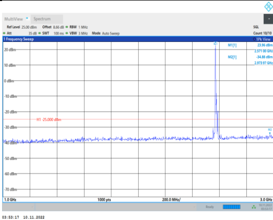
Band38-10MHz-16QAM-37800-1RB#0- Range2:1000~3000MHz
