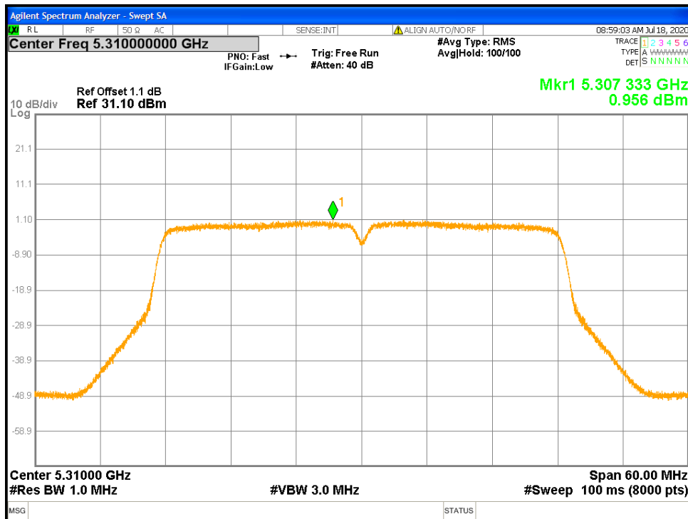
Figure 71: RSS Correlated Power Spectral Density-5310 MHz-802.11n-HT40-MCS0-Ch1
