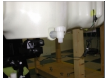
Fig. 22. Body SAR Test Setup with Holster
