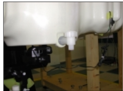
Fig. 20. Body SAR Test Setup with Holster
