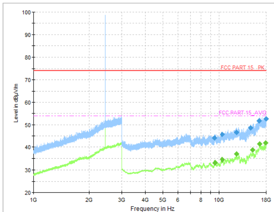
Fig.50 Radiated Spurious Emission (Ch19, 1 GHz - 18 GHz), 2M
