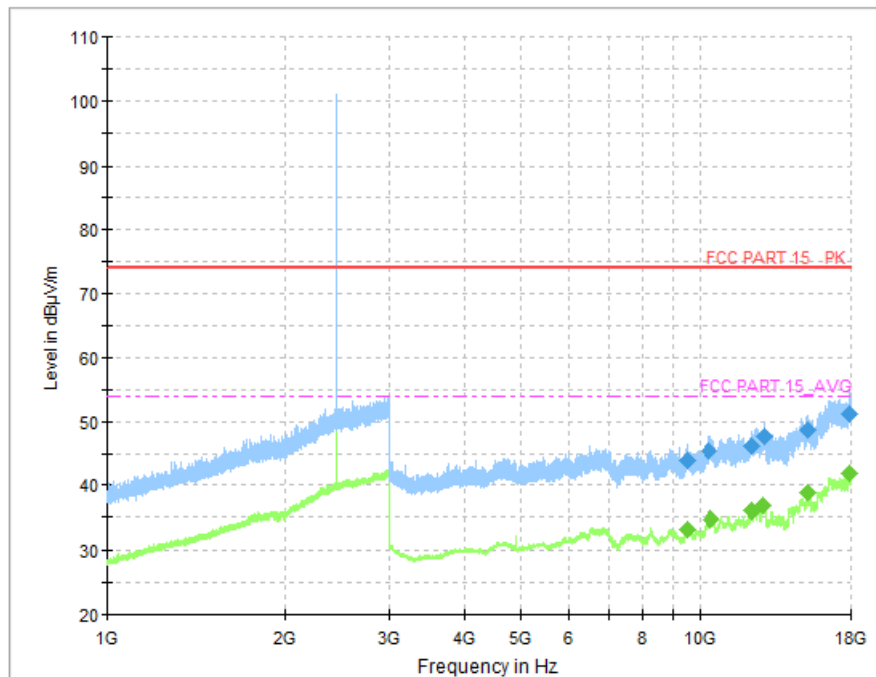
Fig.42 Radiated Spurious Emission (Ch19, 1 GHz - 18 GHz), 1M
