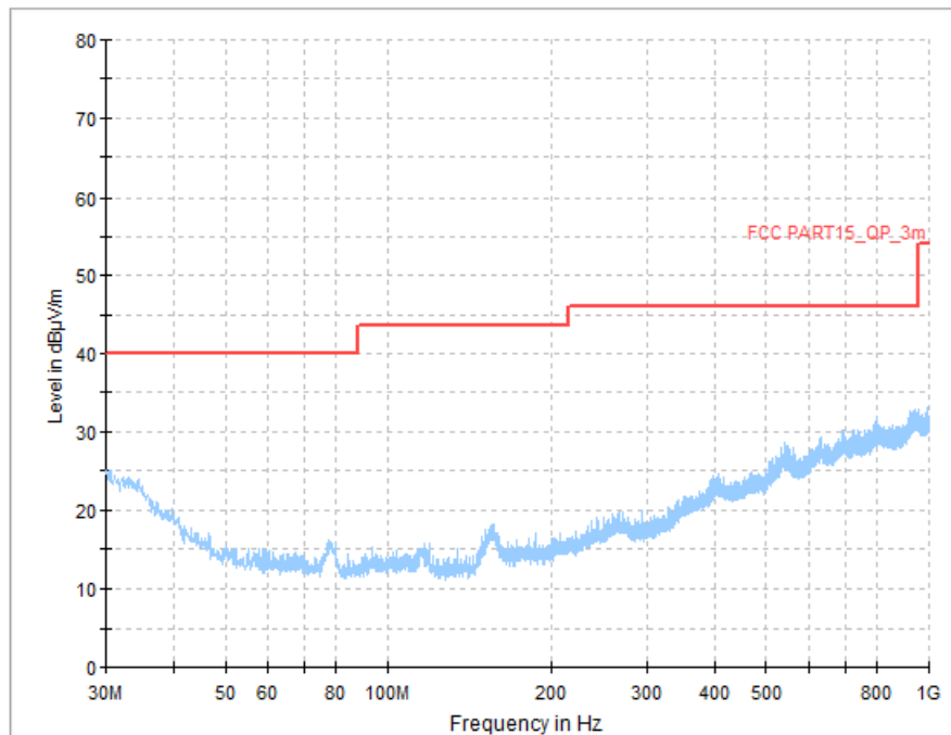
Fig.49 Radiated Spurious Emission (Ch19, 30 MHz - 1 GHz), 2M
