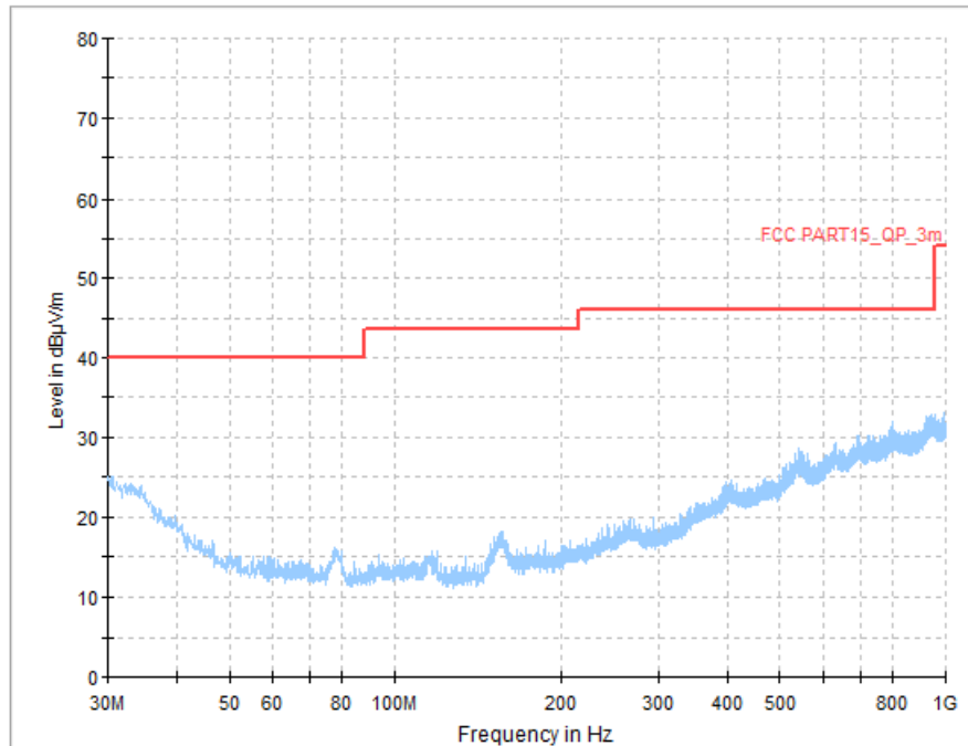
Fig.41 Radiated Spurious Emission (Ch19, 30 MHz - 1 GHz), 1M
