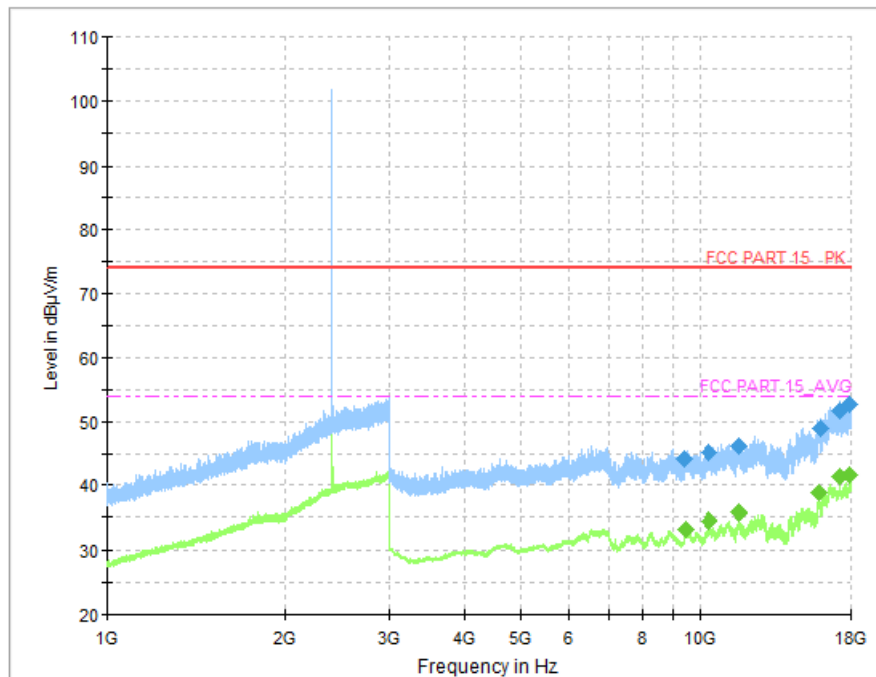
Fig.47 Radiated Spurious Emission (Ch0, 1 GHz - 18 GHz), 2M
