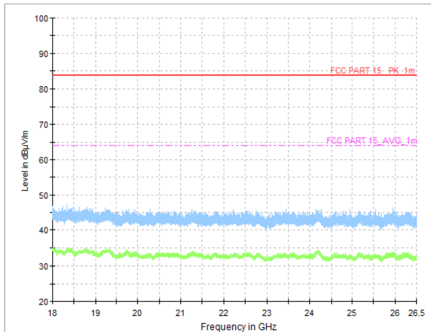
Fig.51 Radiated Spurious Emission (Ch19, 18 GHz - 26.5 GHz), 2M
