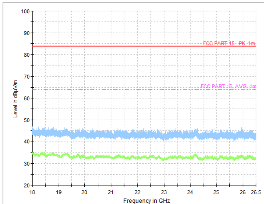
Fig.43 Radiated Spurious Emission (Ch19, 18 GHz - 26.5 GHz), 1M
