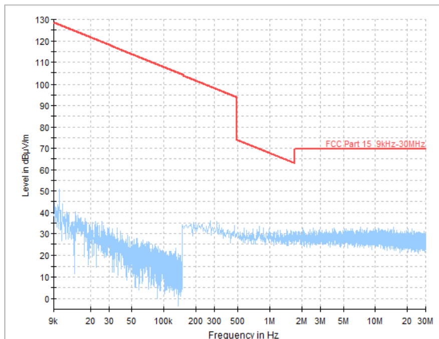
Fig.40 Radiated Spurious Emission (Ch19, 9 kHz - 30 MHz), 1M
