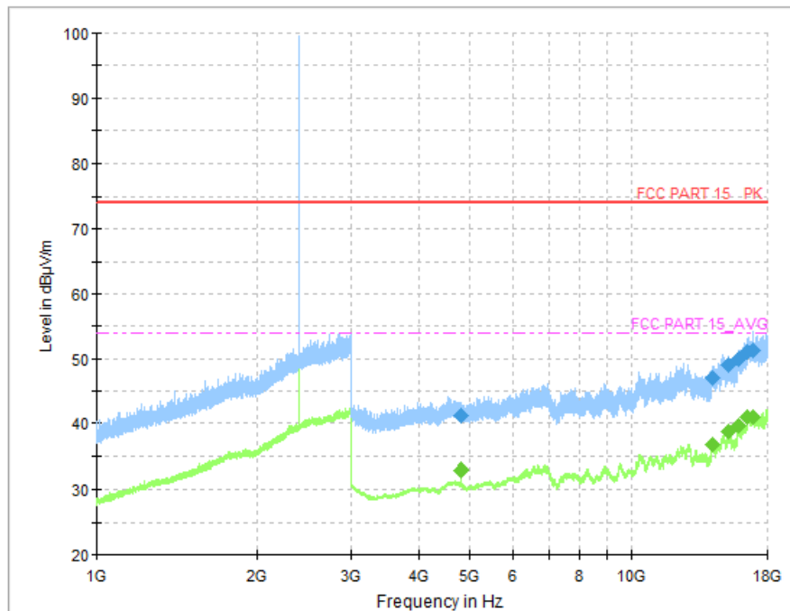
Fig.39 Radiated Spurious Emission (Ch0, 1 GHz - 18 GHz), 1M
