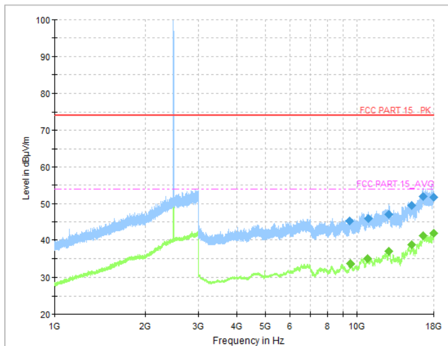
Fig.52 Radiated Spurious Emission (Ch39, 1 GHz - 18 GHz), 2M
