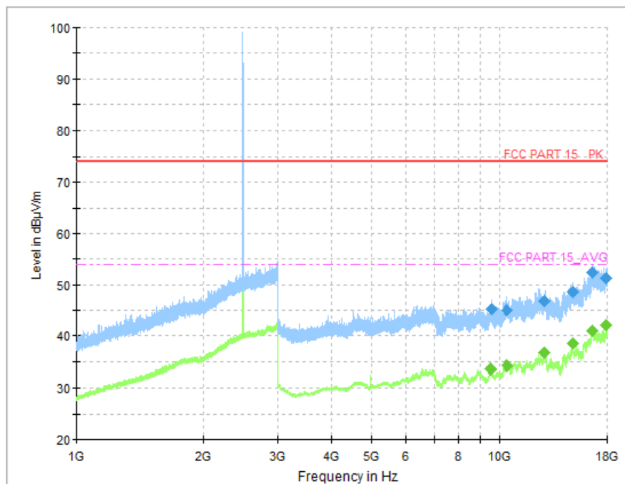
Fig.44 Radiated Spurious Emission (Ch39, 1 GHz - 18 GHz), 1M
